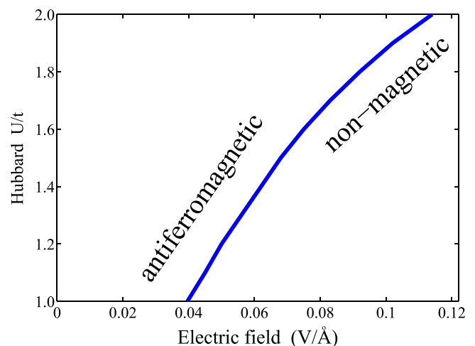
FIG. 6. Ground state phase diagram of the zBGNF for 1.0 \leq U/t \leq 2.0 .
