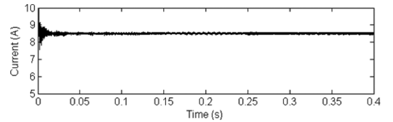
Fig. 10. Waveform of the SB current during charging.
