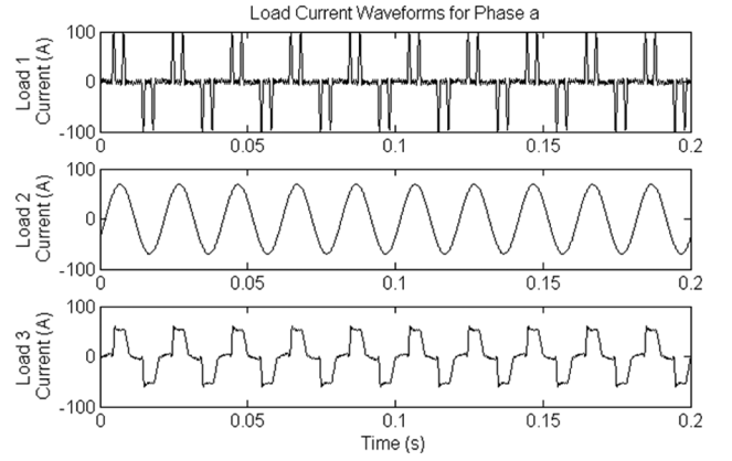
Fig. 9. Per-phase currents drawn by loads 1, 2, and 3.
