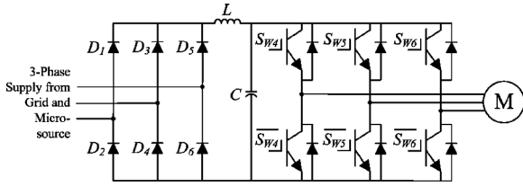
Fig. 8. Configuration of a 15-kVA three-phase ASD.
