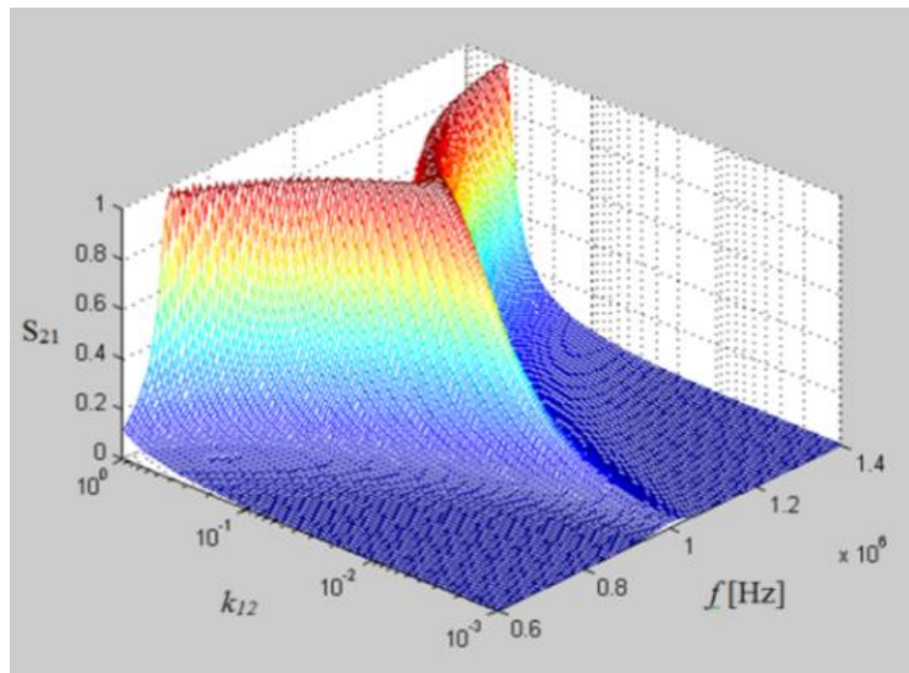
Fig.7 A plot of S_{21} as a function of mutual coupling coefficient and operating frequency for the example with parameters shown in Table I.
