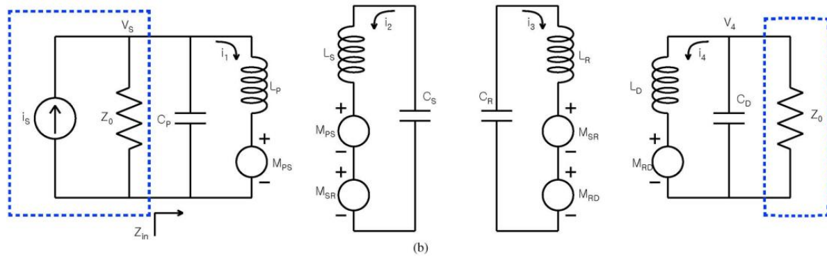
Fig.8 (a) Wireless power system with two coil-resonators, a power driving coil and a load coil, and (b) the equivalent circuits [36] – copyright IEEE
