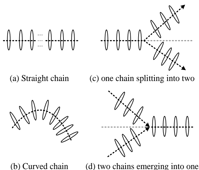
Fig.9 Examples of domino-resonator arrangements [60] - copyright IEEE
