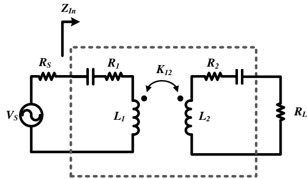
Fig.6 Equivalent circuit of a 2-coil system
