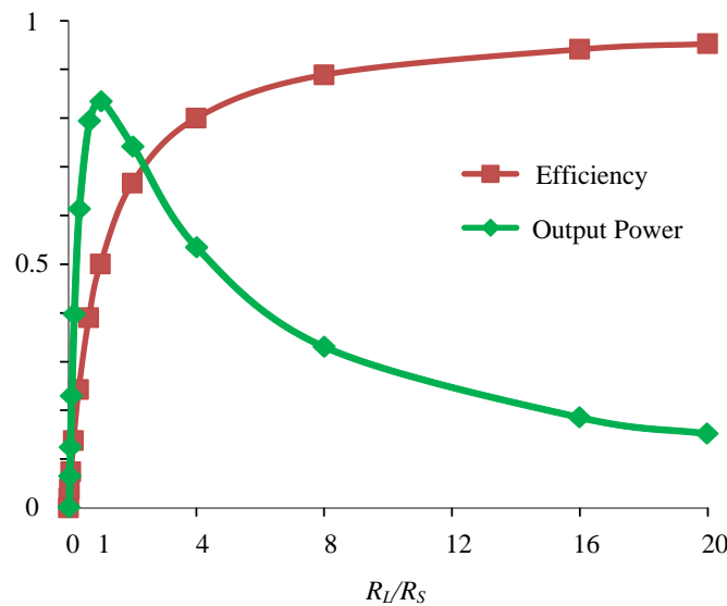
Fig.3b Variations of energy efficiency and output power as a ratio of R_L and R_S for the equivalent circuit in Fig.3a [Y-axis: Per-unit scale]
