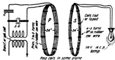
Fig.1 A diagram of one of Tesla’s wireless power experiments [25]
