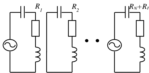
Fig.5 Equivalent circuit of a wireless power transfer based on multiple magnetically coupled resonators
