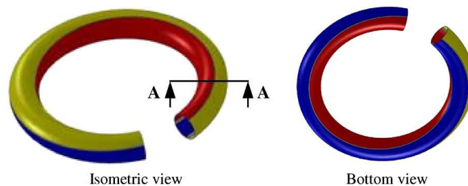
Fig.11 Winding based on surface spiral winding design [62] – copyright IEEE
