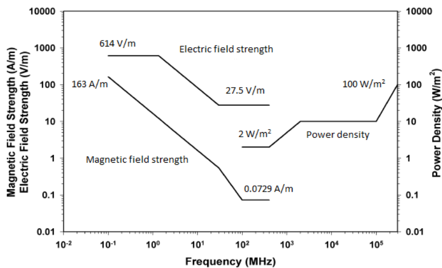
Fig.13 IEEE Reference levels for exposure to time-varying electric and magnetic fields – Copyright IEEE
