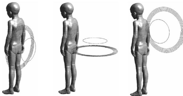
Fig.16 Orientations of the resonator coil at 10mm distance to the body (and the test loop for providing corresponding power information) (from left to right: coronal, axial and sagittal planes) [71] –Copyright IEEE
