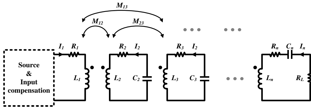
Fig.2 Schematic of a system with n resonators
