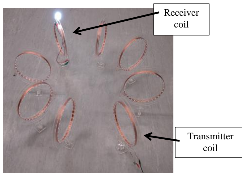
Fig.10 A photograph showing a circular domino-resonator system powering a 18W compact fluorescent lamp [59] – copyright IEEE
