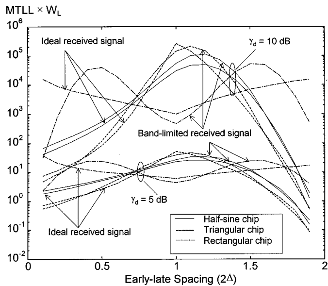
Fig. 5. MTLT against the early-late spacing.
