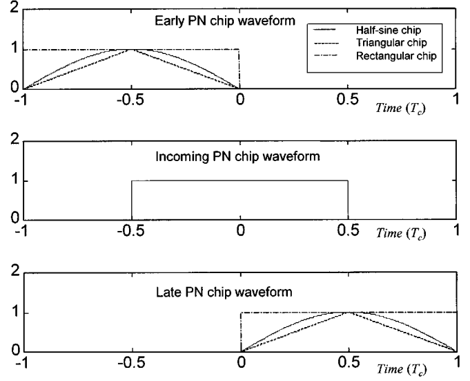
Fig. 2. Early, late, and incoming PN pulses.
