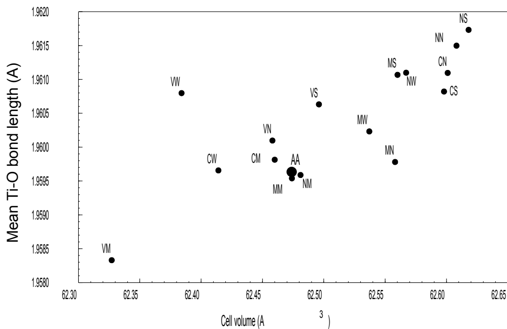
Fig. 10. Rutile cell volume versus mean Ti-O bond length in the octahedral site.
