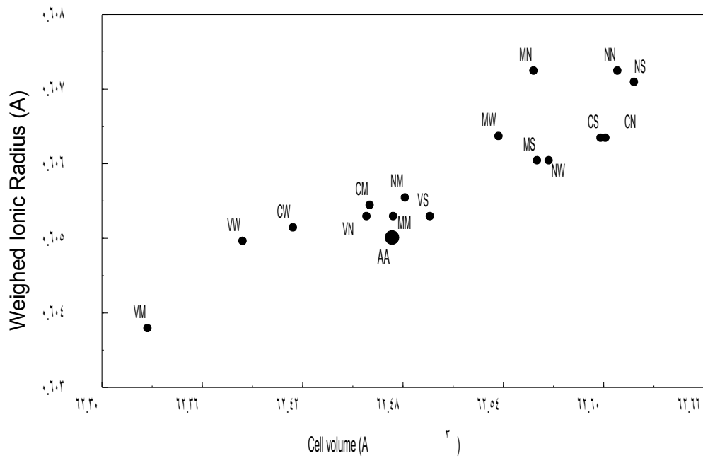
Fig. 9. Rutile cell volume versus weighed ionic radius calculated by titanium, chromophore and counterion occupancy of octahedral site.
