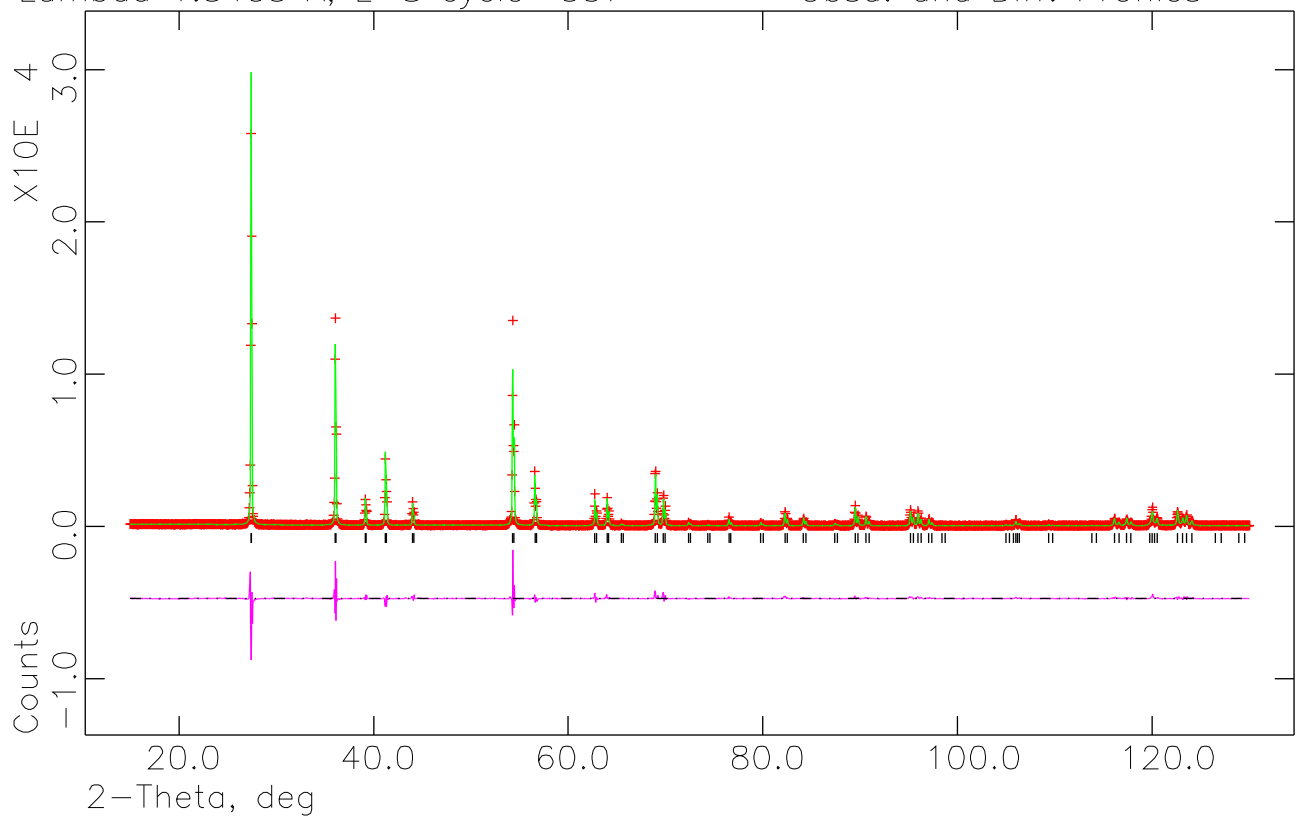
Fig. 1. Rietveld refinement plot of the X-ray powder diffraction data NW11. In the figure the continuous lines represents calculated pattern, while cross points shows observed patterns. The difference curves between observed and calculated profiles is plotted below.
