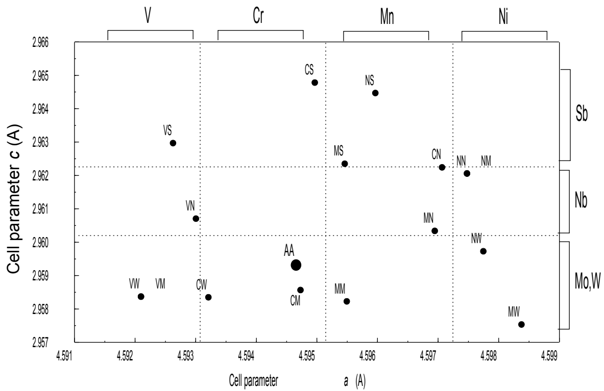
Fig. 8. Cell parameters a versus c of rutile pigments synthesised at 1100 °C.
