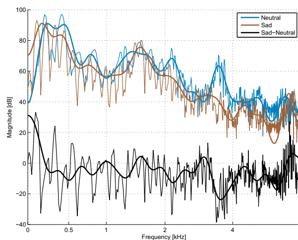
Figure 1: Spectral envelopes and DFT of a pair of corresponding frames (sad and neutral) and their difference (sad-neutral). x -axis is in warped frequency scale. Thin lines represent the short-term spectrum (DFT), while bold lines represent the mel-cepstral spectral envelopes.
