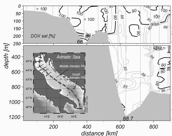
Fig. 2. Vertical distribution of dissolved oxygen along the NW-SE longitudinal section of the Adriatic Sea.
