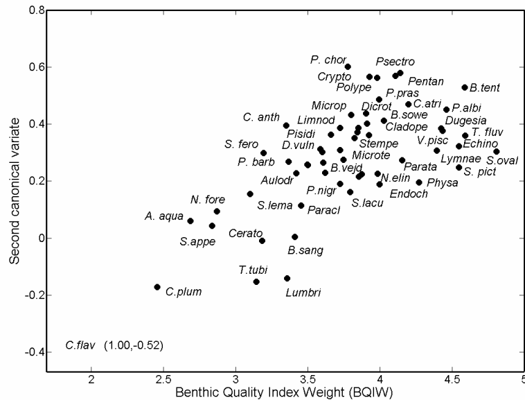
Fig. 3. Plot of BQIW against the factor loadings of the second canonical variate.
