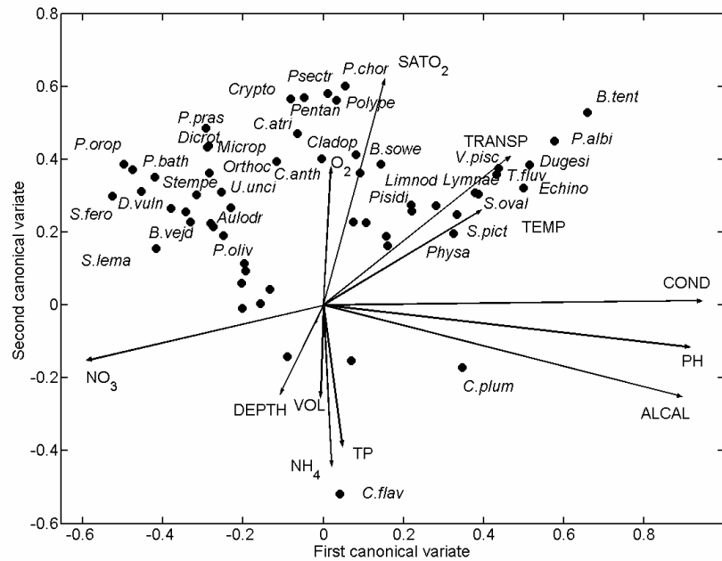
Fig. 1. Biplot of the factor loadings of environmental variables (arrows) and taxa (circles) of the canonical correlation analysis, in the plane defined by the two first axes. Taxa names with absolute values < 0.3 in both axes were not evidenced.
