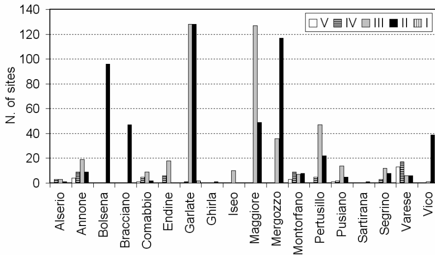
Fig. 5. Frequency of quality classes into which stations of different lakes were assigned according to BQIL values.
