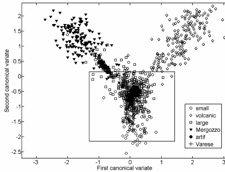
Fig. 2. Factor scores of sites in the plane of the first two axes in the canonical correlation analysis.
