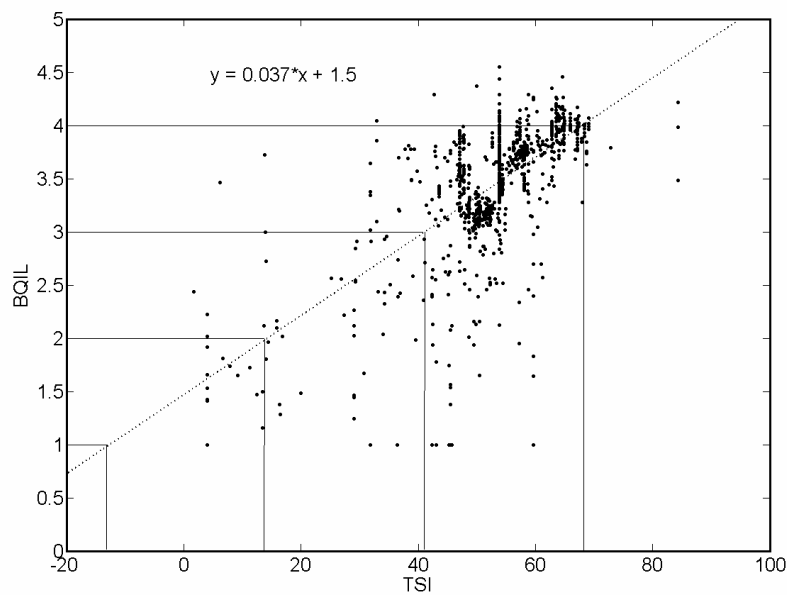
Fig. 4. Plot of the TSI value against the BQIL value calculated for each site. Minimum square line and linear correlation equation are reported.
