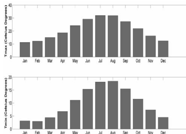
Figure 3. Maximum (upper panel) and minimum temperature (bottom panel) averaged in Foggia Podere 124 station for each month.
