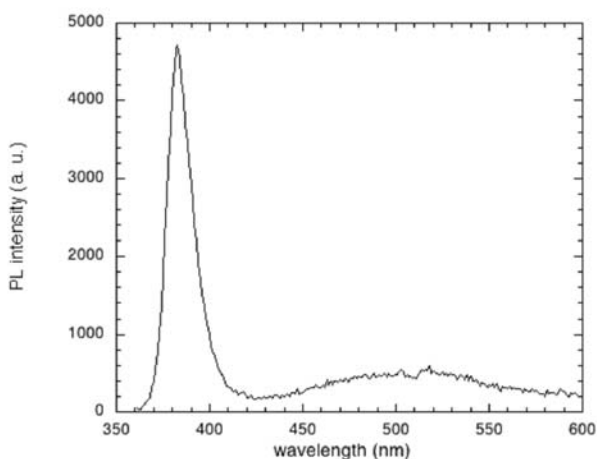
Figure 2. Room temperature PL spectrum of ZnO tetrapods
