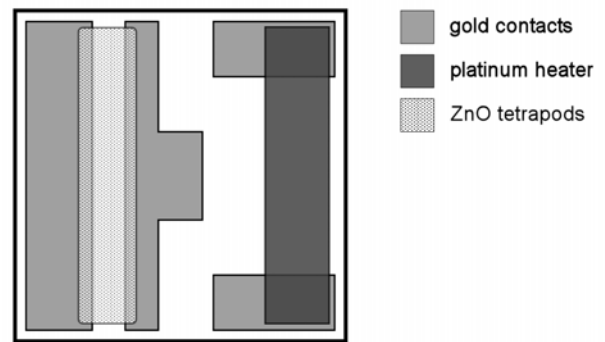
Figure 3. Schematic draw of the sensor contacts and heater geometry.
