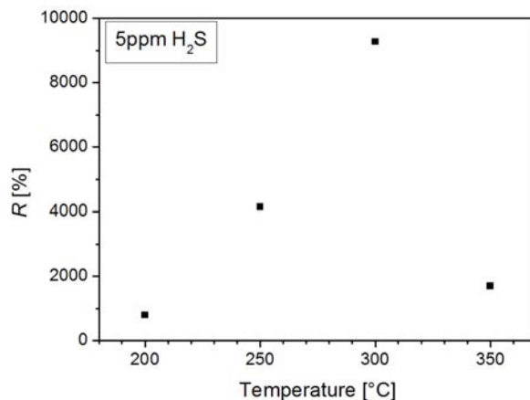
Figure 6. Response to 5 ppm of H 2 S as a function of temperature, measured in dry air condition (0% relative humidity) with a 500ml/min flow.
