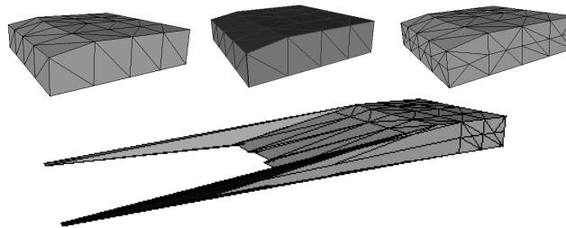
Figure 7: In the top row the chamfer edges (middle) of an initial model (left) were split without moving the new vertices (right). The model in the bottom was obtained by skipping the edge-length check.
