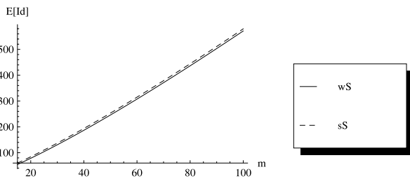
Fig. 5. Expected number of identities needed to successfully perform a weak or strong Sybil attack for increasing values of m . Parameters are max = 100 and \lambda = 10 .
