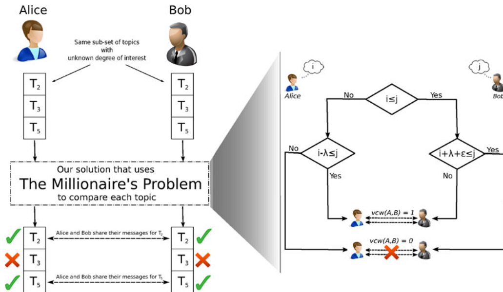
Fig. 1. Privacy-preserving interest-based forwarding.
