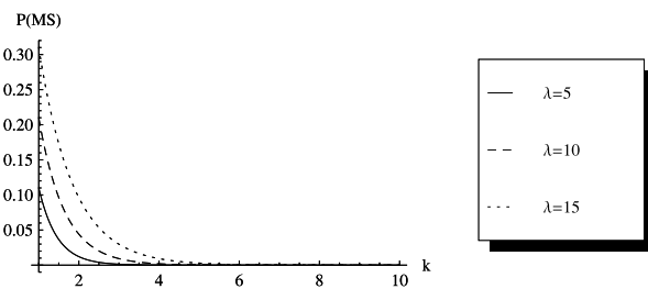
Fig. 4. Probability of mis-forwarding for increasing values of k and different values of \lambda . Parameter max is set to 100 and m is set to 15.
