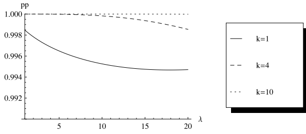
Fig. 2. Value of the expected privacy preservation metric for increasing values of \lambda and different values of k . Parameter max is set to 100 and m is set to 15.
