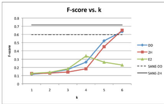
Fig. 7. F-score of the different forwarding protocols for increasing values of k .
