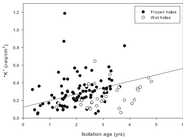
Figure 5e. Scatterplot of the mass of ^*K^+ ( \mu\text{eq}/\text{cm}^2 ) versus isolation age (years) for frozen and wet cryoconite holes on Canada Glacier. The best fit linear regression line for frozen holes is also shown: ^*K^+ = 0.073 \cdot \text{Isolation Age} + 0.12 ( r^2 = 0.1873 , n = 89 ).
