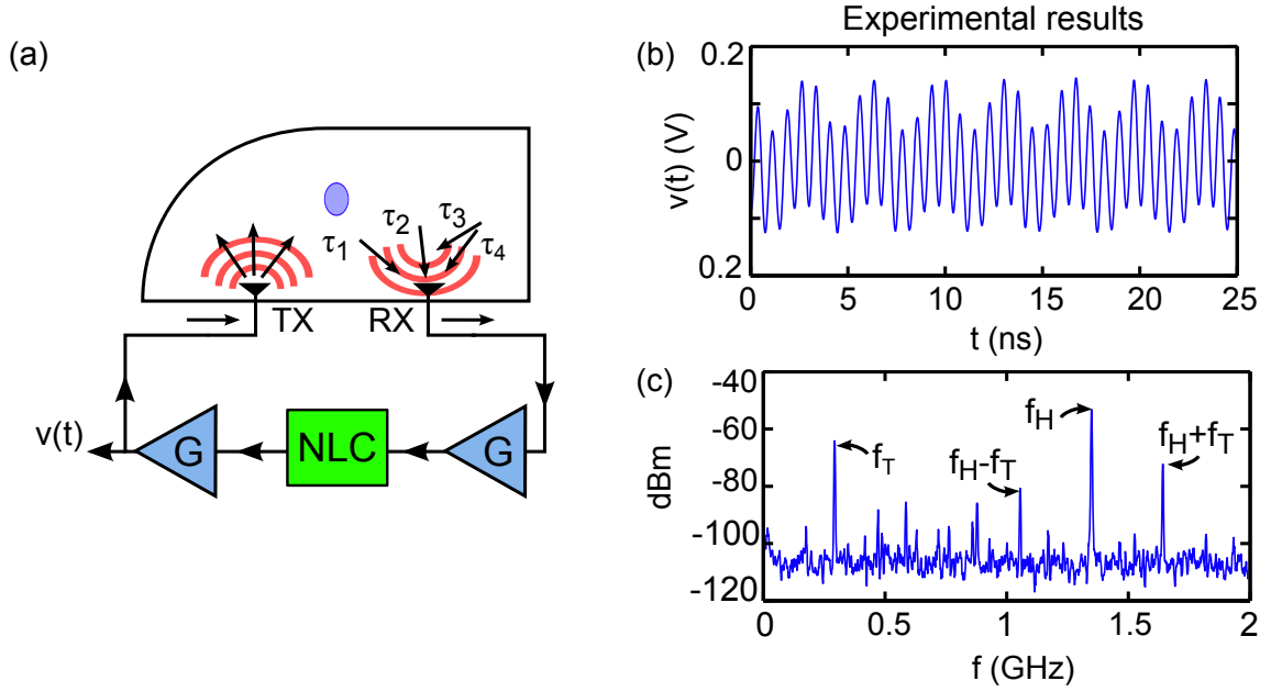
Figure 1.7: Full experimental setup (a) showing the combination of the time-delayed nonlinear feedback system with the wave-chaotic cavity to form the cavity-feedback system. The propagation delays of a scattered signal in the cavity \tau_i through the cavity are the time delays of the nonlinear feedback system. The time-evolving voltage v(t) represents a measurement of the EM oscillations in the feedback loop. The nonlinear element of the feedback loop is a nonlinear circuit (NLC) whose input and output are amplified. (b) Experimental time series of the quasiperiodic oscillations of v(t) while the scatterer's position is fixed. (c) Experimental power spectral density (PSD) of the quasiperiodicity with primary frequencies f_H , f_T , and linear combinations f_H \pm f_T .
