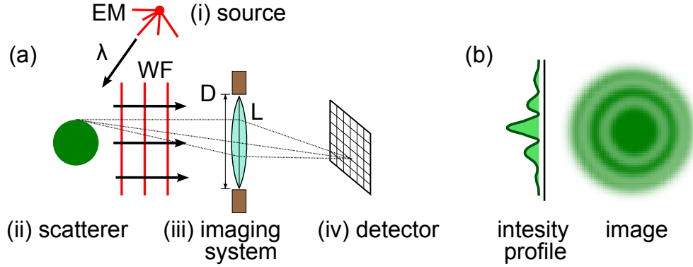
Figure 1.1: Typical imaging system (a) consisting of a (i) a source that produces electromagnetic radiation of wavelength \lambda , (ii) a scatterer that reflects the incident radiation as wavefronts (WF), (iii) an imaging system with a circular aperture of diameter D and lens (L), and (iv) an array detector with light sensitive pixels. (b) For a point-like scatterer, the intensity profile of the light on the detector shows oscillations with primary and secondary maxima and the resulting image or (diffraction pattern) is blurred with concentric rings.
