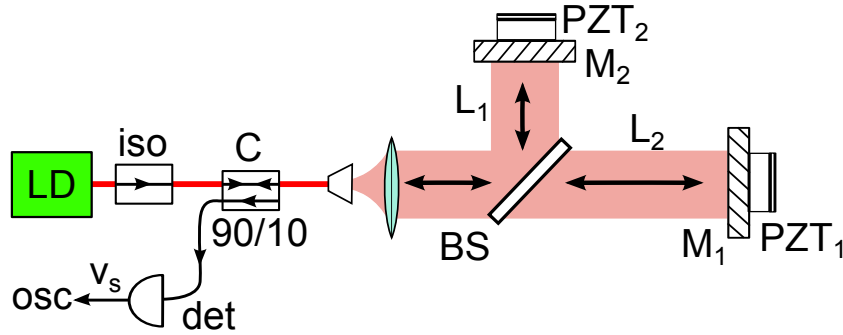
Figure D.2: Interferometer for calibrating the piezoelectric transducers. The output of the laser diode (LD) is fed through a unidirectional isolator (iso) that prevents feedback to the laser cavity. The optical signal is coupled to free space where it is directed along two paths via a beam splitter (BS), where it is reflected off of mirrors ( M_1 and M_2 ) that are attached to the piezoelectric transducers ( PZT_1 and PZT_2 ). The reflected signals interfere along a common path and are coupled (C) to a detector (det), where the voltage v_s is measured on an oscilloscope (osc).
