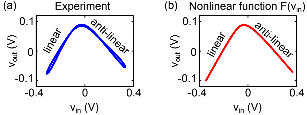
Figure 4.1: Review of circuit operation. (a) Input-output characteristics of the experimental circuit measured at a driving frequency f = 270 MHz with v_b = 0.7 V and with its linear and anti-linear regimes labeled accordingly. (b) Functional fit of the experimental data using the nonlinear function F(v_{in}) = v_o - \sqrt{A^2(v_{in} + v_b - v_T)^2 - a_o^2} , where A = A_L (slope of the linear regime), if (v_{in} + v_b) \leq v_T , and A = A_R (the slope of the anti-linear regime) if (v_{in} + v_b) > v_T .
