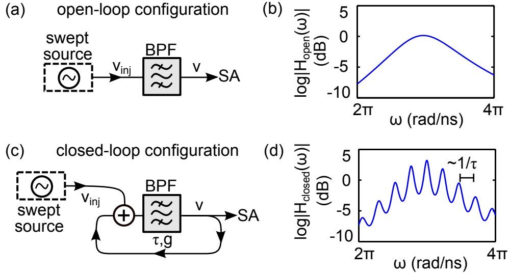
Figure 5.2: Measuring open-loop and closed-loop transfer functions of a band-pass filter using a swept source and spectrum analyzer (SA). (a) Open-loop configuration for measuring (b) |H_{\text{open}}(\omega)| and (c) closed-loop configuration with time delay \tau and gain coefficient g = 0.3 for measuring (d) |H_{\text{closed}}(\omega)| .
