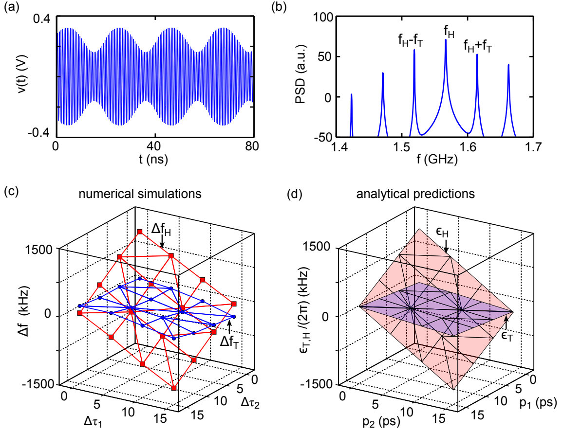
Figure 6.5: Simulated and predicted spectral shifts in a two-delay system. (a) Typical quasiperiodic time series for v(t) from integrating the simplified model. (b) Power spectral density of the simulated v(t) with f_H and f_H \pm f_T labeled accordingly. (c) Simulated spectral shifts \Delta f_T (blue dots) and \Delta f_H (red squares) for the delay shifts (\Delta\tau_1, \Delta\tau_2) associated with the delays \tau_1 = 7 ns and \tau_2 = 12 ns. (d) Analytically-predicted values of the planar spectral shifts \epsilon_H/(2\pi) (blue) and \epsilon_T/(2\pi) (red) calculated using Eq. (6.31) for the delay shifts (p_1, p_2) .
