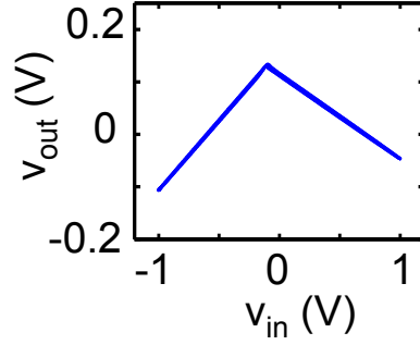
Figure A.7: Input versus output voltages of the RLC model. The output voltage v_{\text{out}} plotted as a function of v_{\text{in}} for a input driving frequency of f = 270 MHz with v_b = 0.65 V, v_T = 0.72 V and V_{CC} = 1.3 V. The parameters of the model are R_{\text{in}} = 50 \Omega , R_{\text{NL}} = 30 \Omega , R_1 = 5.1 \Omega , R_2 = 68 \Omega , R_L = 50 \Omega , R_{\text{on}} = 500 \Omega , C_1 = 47 nF, C_2 = 100 nF, L_1 = 4 nH, and \beta = 60 with the depletion capacitances C_{\text{BE}} = 500 fF and C_{\text{BC}} = 500 fF.
