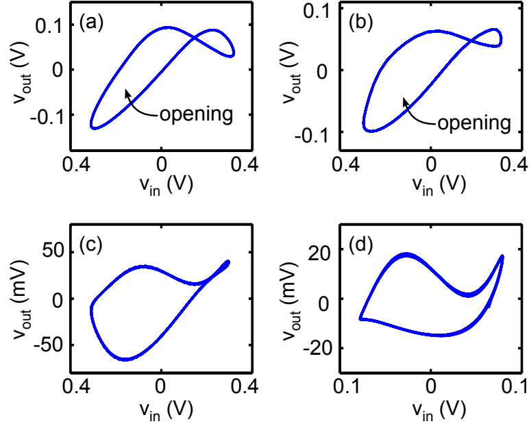
Figure 4.2: Experimental high-frequency distortions. Experimental distortions of v_{\text{out}} for sinusoidal driving signals v_{\text{in}} at frequencies (a) f = 500 MHz with v_b = 0.65 V, (b) f = 1.1 GHz with v_b = 0.65 V, (c) f = 1.5 GHz with v_b = 0.7 V, and (d) f = 1.9 GHz with v_b = 0.74 V. The frequencies used to create Fig. 4.2 are chosen to highlight the progression of these distortions for various bias voltages v_b . In (a) and (b), the opening of the tent-like shape is labeled accordingly. For all measurements, the paths to the oscilloscope for v_{\text{in}} and v_{\text{out}} are approximately balanced with equal propagation times. The error of each voltage measurement is estimated as \pm 2 mV based on the standard deviation of the oscilloscope noise floor.
