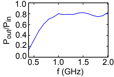
Figure B.5: Antenna far-field efficiency calculated by measuring P_{out}/P_{in} .
