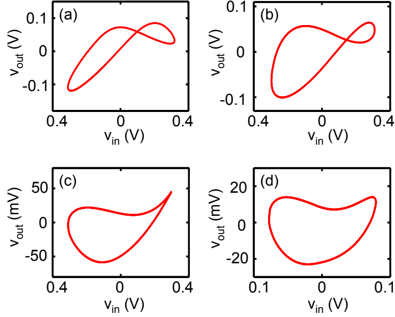
Figure 4.7: Simulated high-frequency distortions. Simulated v_{\text{out}} plotted as a function of v_{\text{in}} using the full model of the NLC and the experimental input sinusoidal signals v_{\text{in}} at frequencies and bias voltages of (a) f = 500 MHz with v_b = 0.65 V, (b) f = 1.1 GHz with v_b = 0.65 V, (c) f = 1.5 GHz with v_b = 0.7 V, and (d) f = 1.9 GHz with v_b = 0.74 V. The RMS errors between the data at f = (0.5, 0.7, 1.1, 1.5) GHz and the respective fits are (12.3, 18.5, 10.4, 6.8) mV, which represent (6.0, 11.2, 6.3, 18.4)% errors for the given experimental ranges.
