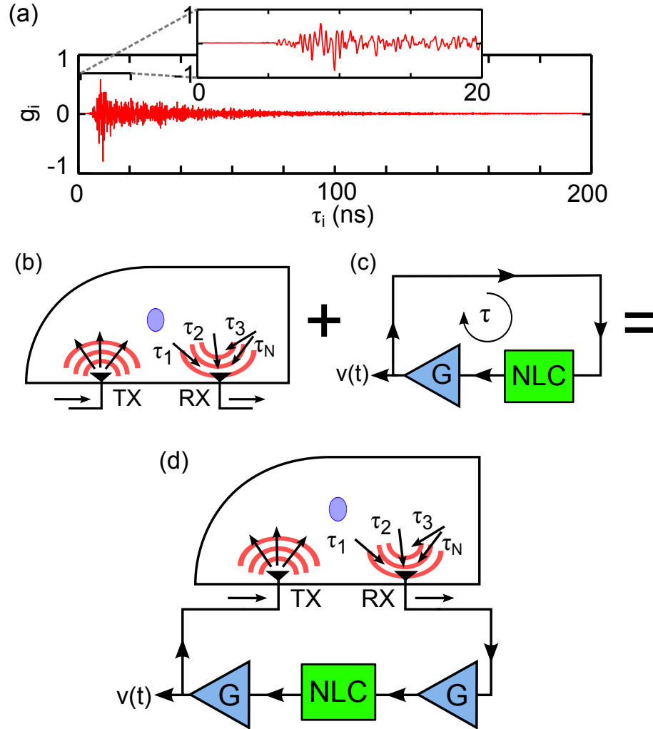
Figure 3.1: Conceptual overview of the subwavelength sensing system (a) Delay distribution of the wave-chaotic cavity with a zoom of the region between \tau_i = 0 and \tau_i = 20 ns. The data is collected using 100 averaged waveforms. The spacing between data points ( \tau_i, g_i ) is \Delta\tau = \tau_{i+1} - \tau_i = 0.025 ns. (b) The delays \tau_i labeled in a schematic representation of the wave-chaotic cavity. (c) A schematic representation of the basic ingredients for a time-delayed nonlinear feedback system. (d) Schematic representation of the combined wave-chaotic cavity and time-delayed nonlinear feedback system. The propagation delays \tau_i of the delay distribution are now the time delays of the nonlinear feedback loop.
