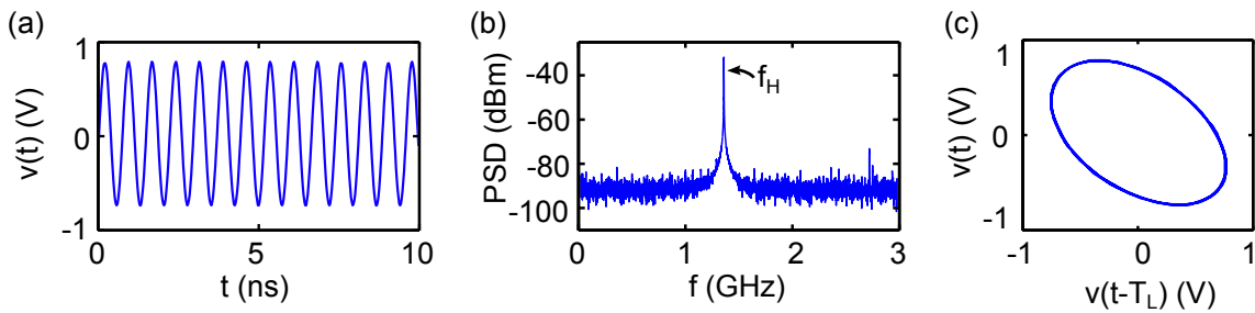
Figure 3.8: Periodic dynamics used for sensing. (a) Periodic time series, (b) power spectral density, and (c) phase space projection with lag time T_L = 1 ns.
