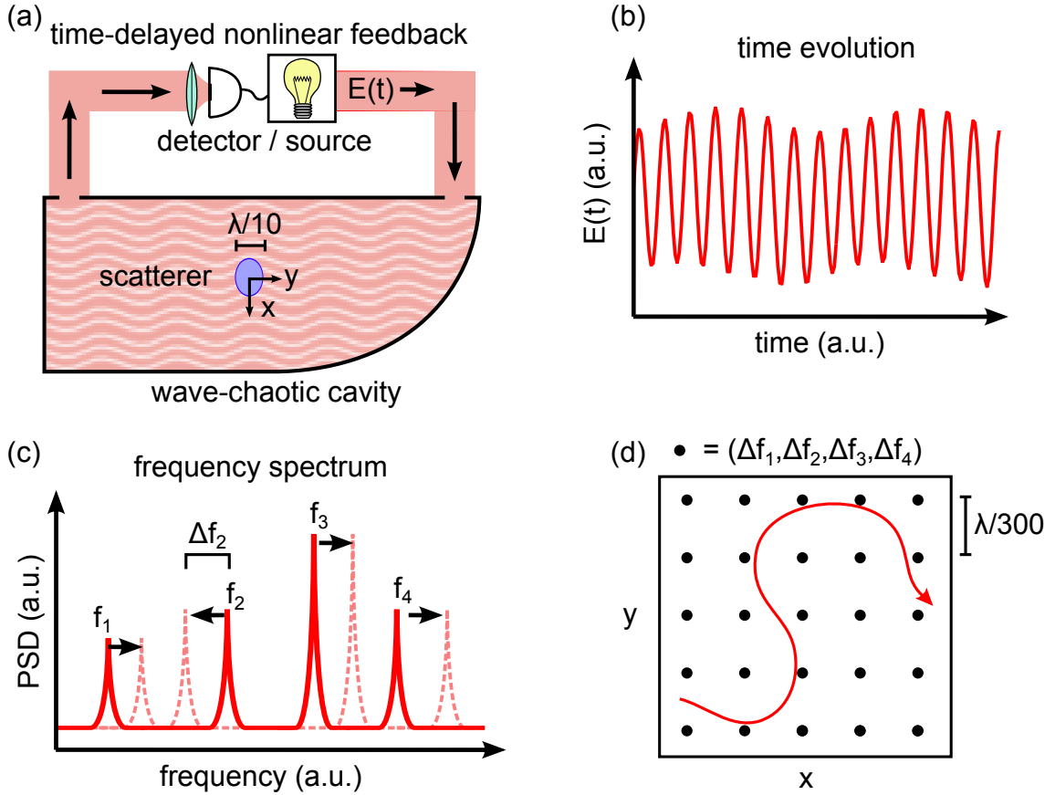
Figure 1.5: Time delayed nonlinear feedback through a wave-chaotic cavity. (a) A source floods EM radiation into a wave-chaotic cavity, where it scatters and diffracts off of a subwavelength object ( \sim\lambda/10 ), exits the cavity to a detector, and recirculates through the feedback loop. (b) The measured EM radiation as a function of time. (c) The power spectral density of the detected field E(t) with primary frequencies that shift as a function of scatterer position. (d) Calibration grid (black dots) for interpolating and tracking the scatterer’s location (red curve) in a 2D plane (x, y) with subwavelength resolution.
