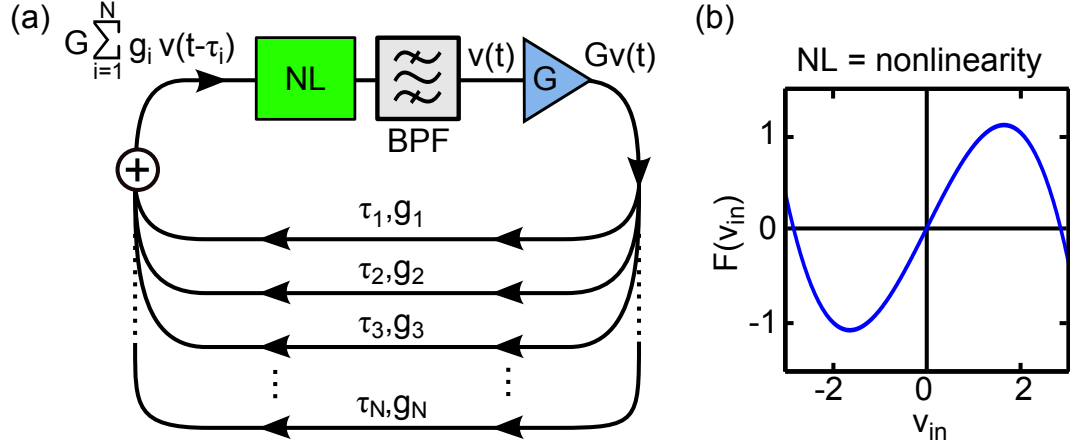
Figure 5.1: Band-pass filter with nonlinear feedback. (a) The output of a band-pass filter v(t) is split among N time-delays, each with propagation delay \tau_i and gain coefficient g_i . The delayed outputs of each feedback loop are summed and amplified with linear gain G before passing through a nonlinearity (NL). The output of the NL drives the band-pass filter, forming a closed loop feedback system. (b) Cubic nonlinearity using the third-degree polynomial F(v_{in}) with \alpha_1 = 1 , \alpha_2 = 0.5 and v_b = 0 .
