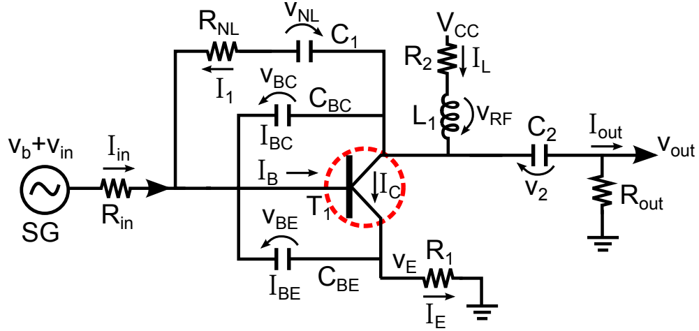
Figure A.6: Circuit schematic of an RLC model for the NLC with depletion capacitances. For simplicity, rather than including the bias-T components from Fig. A.1d, the bias voltage v_b is added directly to v_{in} . Arrows indicate the directions of positive voltage changes and positive current flows. An input resistance R_{in} and output resistance R_{out} model the impedances of the experimental signal generator (SG) and oscilloscope (osc). The transistor T_1 is highlighted by the red dotted circle.
