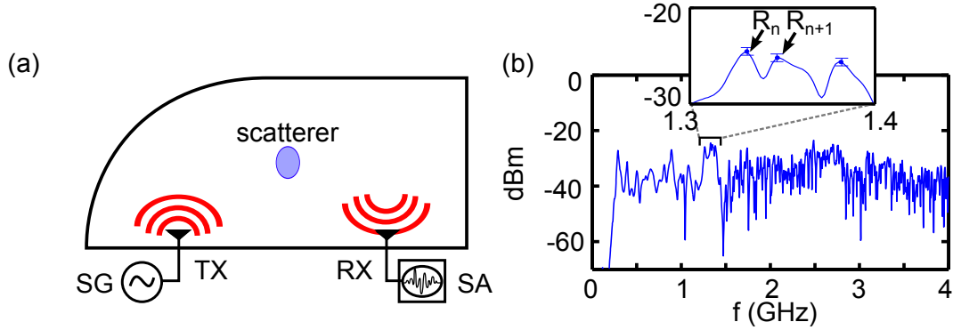
Figure 2.13: Measuring the experimental resonances of the cavity. (a) Experiment setup for measuring the resonances (with and without the scatterer) using a swept-frequency signal generator (SG) and a spectrum analyzer (SA). (b) The experimental resonances of the cavity with the scatterer as a function of frequency f . A zoom of the boxed region shows an example of two resonances R_n and R_{n+1} . Errors indicate the accuracy \pm 0.4 dBm of the SA. Resonances are located using MATLAB's findpeaks algorithm, which locates local maxima, where the parameters of the algorithm are specified such that consecutive local maxima must be spaced by at least 3 MHz (mean spacing between resonance peaks is 13.4 MHz) and must be greater than -70 dBm (mean resonance peak height is -44 dBm).
