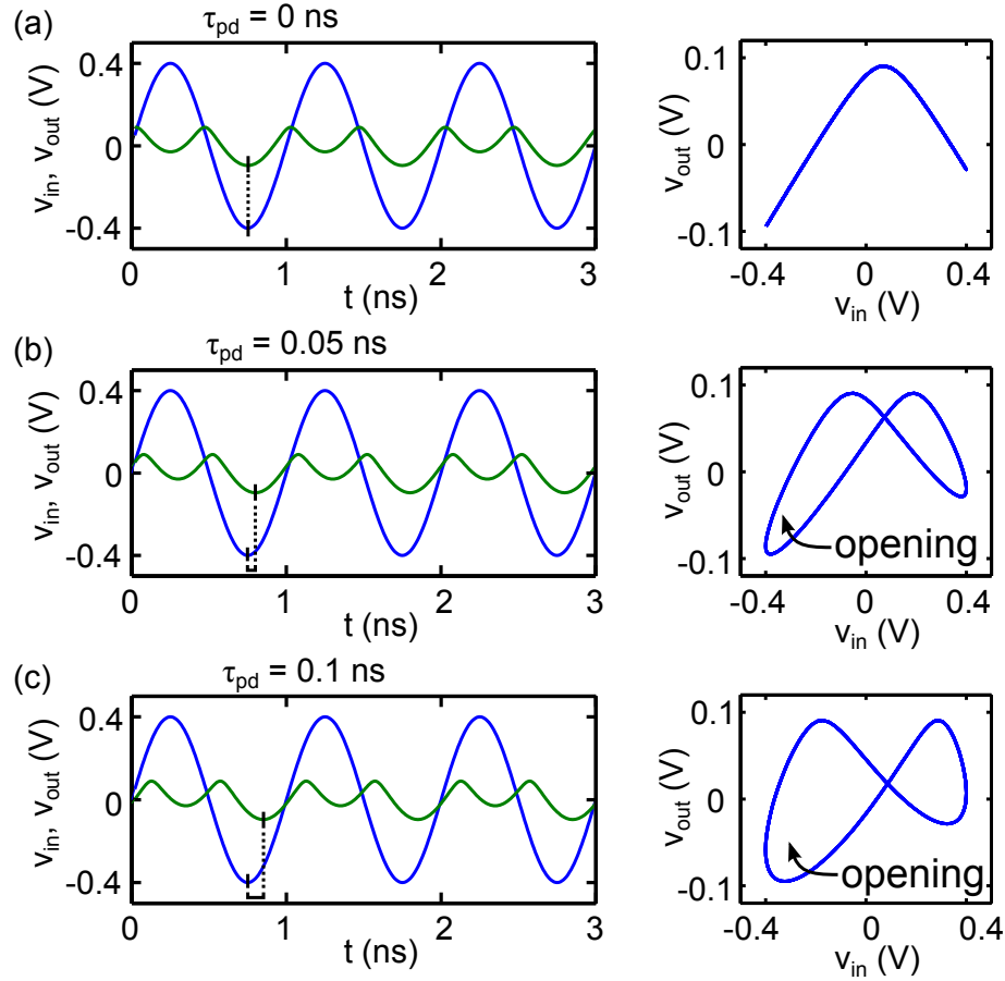
Figure 4.4: Simulated effects of an increasing propagation delay. A simulated input sinusoidal v_{in} at frequency f = 1 GHz drives nonlinear function F(v) with bias voltage v_b = 0.65 V. The output v_{out} (green curve) plotted alongside v_{in} and plotted versus v_{in} for output propagation delays (a) \tau_{pd} = 0 ns, (b) \tau_{pd} = 0.05 ns, and (c) \tau_{pd} = 0.1 ns. Vertical lines with an arrow mark the increase in the propagation delays and the opening of the tent-like shapes are labeled in (a) and (b), accordingly.
