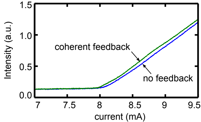
Figure D.1: Laser threshold with coherent feedback. Output intensity of the laser as a function of input current near the laser threshold with (green curve) and without (blue curve) coherent feedback.
