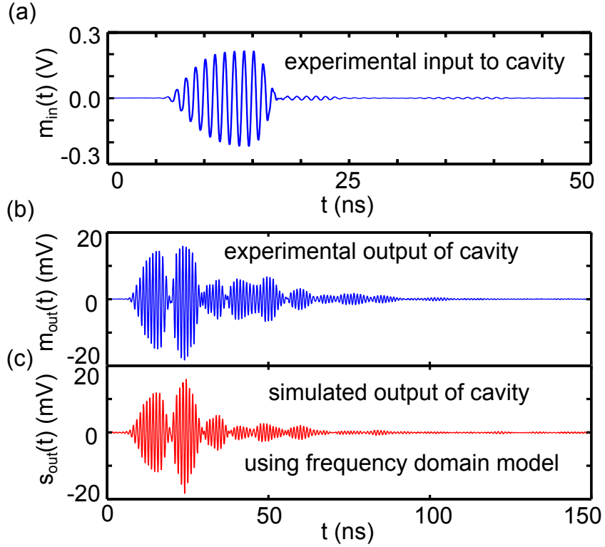
Figure 4.10: Test signal to demonstrate the frequency domain model. Temporal evolution of (a) the cavity input test signal m_{in}(t) (created using the signal generator E8267D), (b) the experimental response of the cavity m_{out}(t) , and (c) the simulated cavity output s_{out} . In the figures, I have scaled the amplitudes of the waveforms by a constant factor to normalize the power in m_{in}(t) to match that of r_{in}(t) . Also, note the change of the horizontal scales between (a) and (b)-(c).
