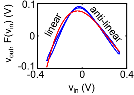
Figure C.2: Simplified model of the system’s nonlinearity. Experimental data from the NLC (blue) where v_{\text{in}} is a sinusoidal driving signal at frequency f = 260 MHz with the numerical fit (red) of Eq. (C.2).
