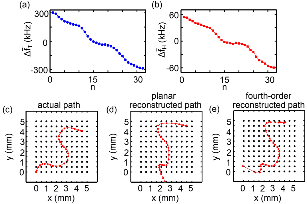
Figure 3.18: 2D predicted positions using quasiperiodicity. Frequency shifts (a) \Delta\bar{f}_T and (b) \Delta\bar{f}_H as a function of n different scatterer positions along (c) the 2D arbitrary path (red curve) within the calibrated grid (black dots). Using the calibrated grid and the measured frequency shifts, the scatterer path is reconstructed using (d) a planar first-order map and (e) a fourth-order map (red curves).
