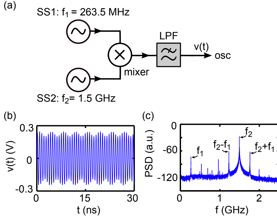
Figure B.2: Calibration setup and signal generated for quantifying the measurement errors of frequency shifts. (a) The frequency f_1 is generated by signal source 1 (SS1), a Hewlett Packard network analyzer (8753E), and the frequency f_2 is generated by signal source 2 (SS2), an Agilent Technologies signal generator (E8267D). I use the same low-pass filter (cascaded Mini-Circuits LFCN-1400, LFCN-2000) at the output of a mixer (Mini-Circuits ZFM-2000) that cuts all frequencies above 2 GHz and appears in the feedback loop of the cavity-feedback system. The resulting output voltage is (b) an artificially-generated quasiperiodic signal and with (b) power spectral density (PSD) that contains four prominent frequencies f_1 , f_2 , f_2 - f_1 , and f_2 + f_1 .
