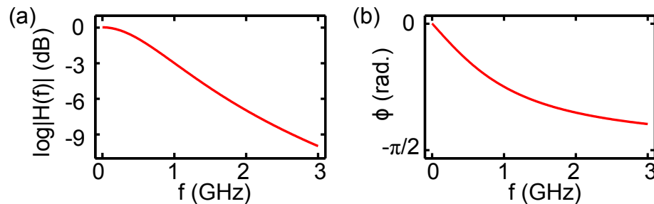
Figure 4.3: First-order low-pass filter. (a) Magnitude of the low-pass filter transfer function H_{\text{LP}}(f) = \tilde{v}_{\text{out}}/\tilde{v}_{\text{in}} and (b) output phase \phi of the filter with respect to input frequency f .
