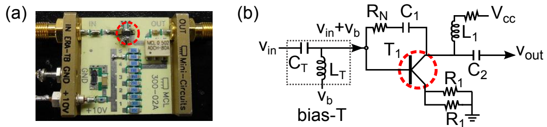
Figure A.3: Illing et al. nonlinear circuit. (a) Photograph of the previous circuit (from Ref. [22]), where the transistor is highlighted in the red dotted circle. (b) Circuit diagram of the original nonlinear circuit with transistor T_1 , where R_N = 68 \Omega , R_1 = 4.75 \Omega , R_2 = 47 \Omega , C_1 = 47 nF, C_2 = 0.39 \mu\text{F} , and L_1 is a radio-frequency choke (MCL Model AdcH-80A). The capacitor C_T and inductor L_T represent the bias-T (grey dotted box) that adds the voltages v_{in} and v_b .
