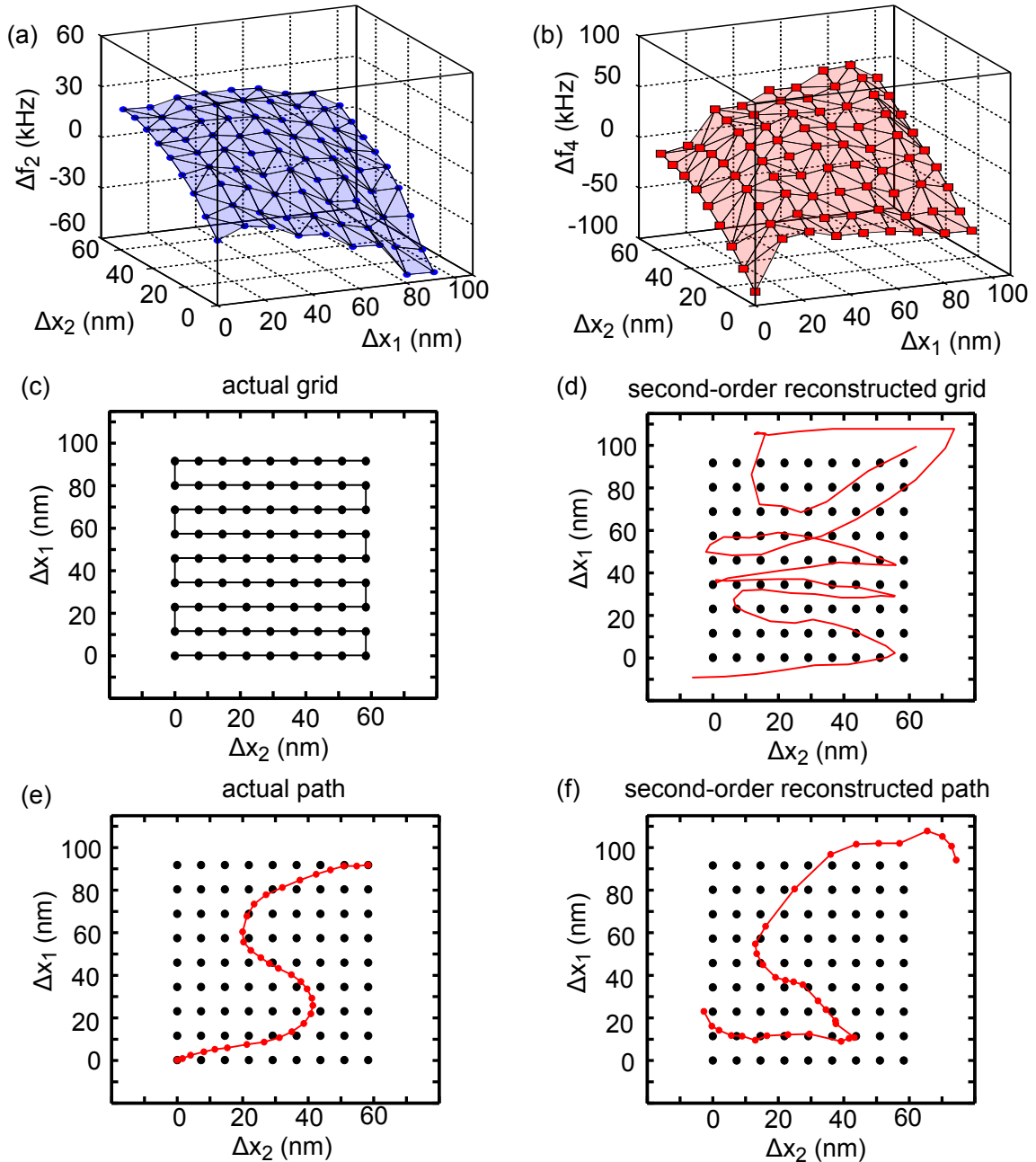
Figure 7.4: Quasiperiodic frequency shifts used for subwavelength sensing. Observed frequency shifts (a) \Delta f_2 and (b) \Delta f_4 as a function of the relative positions \Delta x_1 and \Delta x_2 . (c) Calibration grid path (black curve) and (d) reconstructed grid path (red curve). (e) Actual path (red curve) of (\Delta x_{1,n}, \Delta x_{2,n}) positions to test the 2D grid (black dots) of the frequency shifts. (f) Reconstructed path (red curve) of the relative length shifts using the 2D grid (black dots).
