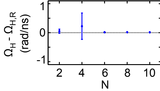
Figure 5.5: Resonance sweep method for dynamical systems with multiple time-delays. For each simulation with N = 2 to N = 10 feedback loops, \tau_i and g_i are sampled from uniform distributions such that 5 \text{ ns} < \tau_i < 50 \text{ ns} and -1 < g_i < 1 . Once the gains are chosen, they are renormalized using the condition \sum_{i=1}^N |g_i| = 1 . The bandwidth parameters are chosen to be \omega^{(+)} = 9.4 and \omega^{(-)} = 6.3 . When implementing the R method, G = 0.95 . The predictions are tested by calculating the mean \mu(N) (blue dots) and standard deviation \sigma(N) (error bars) of (\Omega_H - \Omega_{H,R}) for each N .
