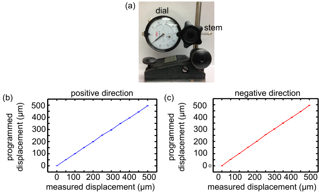
Figure B.6: Scatterer displacement measurements. (a) Dial drop indicator. (b) Measurements of the scatterer displacements in the positive direction and (c) the negative direction as a function of the programmed positions of the translation stage.
