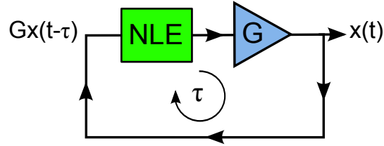
Figure 2.1: Time-delayed nonlinear feedback system. (a) General time-delayed nonlinear feedback system with a nonlinear element (NLE), net time delay \tau , gain G , and state variable x(t) .
