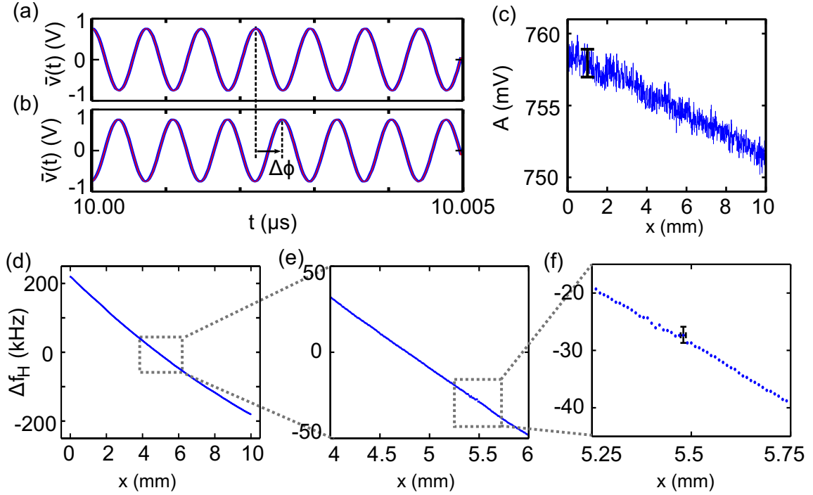
Figure 3.10: 1D sensing with periodic dynamics. Time series \bar{v}(t) (blue curve) with overlaid fitted function (red curve) at (a) x_{\text{rel}} = 0 mm and (b) x_{\text{rel}} = 1 mm. The apparent phase shift \Delta\phi (from the large trigger skew t_s = 10 \mu\text{s} ) on of the time series is marked with dash lines. (c) Amplitude of the periodic signal as a function of x . The error bar indicates the standard deviation \sigma = 2 mV of the noise floor of the oscilloscope after 100 averages. (d)-(f) Successive zooms of the frequency shift \Delta f_H . The mean of the overall shift has been subtracted from (d) for easier relative comparisons. The error bars in (f) indicate the frequency measurement error of the fitting method ( \sim 3 kHz) and the translational stage position error ( \pm 5 \mu\text{m} ).
