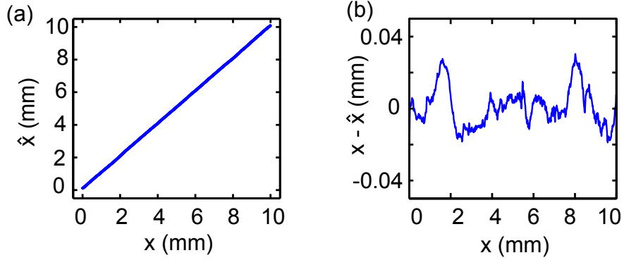
Figure 3.11: 1D predicted positions using periodicity. (a) Predicted position \hat{x} versus actual position x using the inverted map. (b) Errors (x - \hat{x}) of the mapping as a function of x .
