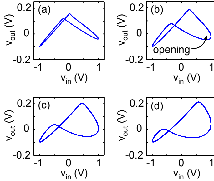
Figure A.9: Distortions in the RLC model with high depletion capacitances. Input voltages v_{in} versus output voltages v_{out} in the RLC circuit model for sinusoidal driving signals at frequencies (a) f = 100 MHz, (b) f = 300 MHz, (c) f = 500 MHz, and (d) f = 700 MHz with the depletion capacitances C_{BE} = 5 pF and C_{BC} = 5 pF.
