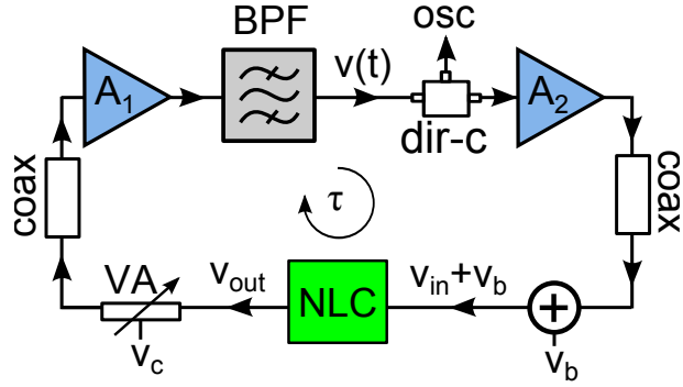
Figure 2.3: Ultra-high-frequency system. The nonlinear circuit (NLC) drives a variable attenuator (VA, Mini-Circuits ZX73-2500+) with a control voltage ( v_c ), the amplifier A_1 (Mini-Circuits ZX60-3018G+), a band-pass filter (BPF, Mini-Circuits ZBFV-925+), a directional coupler (dir-c, Mini-Circuits ZX30-9-4+), the amplifier A_2 (comprised of two amplifiers in series: Mini-Circuits ZX60-3018G+ and Picosecond Pulse Labs 5828-108), and a bias-T (Mini-Circuits ZFBT-6G+) with bias voltage v_b . Coaxial cables (coax) connect these components and act as a propagation delay. The net time-delay of a signal through the feedback loop is \tau .
