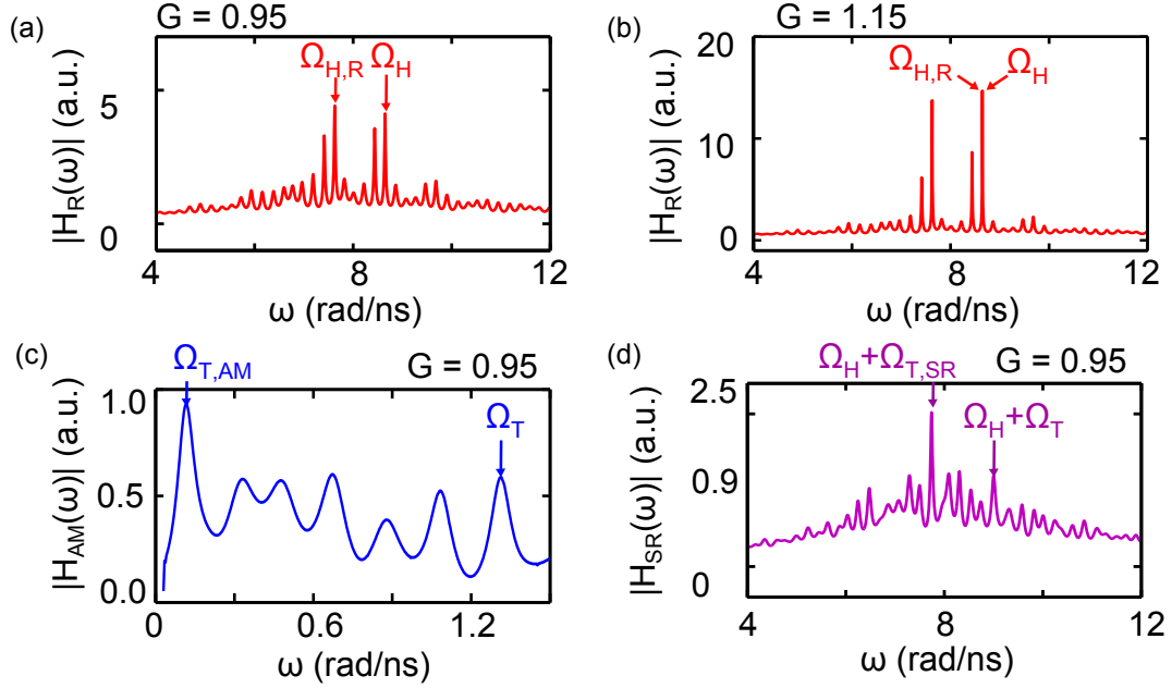
Figure C.6: Special cases of the frequency estimation methods. (a) |H_R(\omega)| for N = 4 and G = 0.95 where \Omega_{H,R} \sim 7.6 rad/ns and \Omega_H = 8.6 rad/ns. (b) |H_R(\omega)| for N = 4 and G = 1.15 where \Omega_{H,R} \sim \Omega_H \sim 8.6 rad/ns. (c) |H_{AM}(\omega)| for N = 10 and G = 0.95 where \Omega_{T,AM} \sim 0.1 rad/ns and \Omega_T \sim 1.4 rad/ns. (d) |H_{SR}(\omega)| for N = 10 and G = 0.95 where \Omega_H + \Omega_{T,SR} \sim 7.7 rad/ns and \Omega_H + \Omega_T \sim 9.0 rad/ns.
