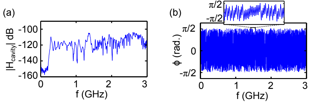
Figure 4.9: Transfer function of the wave-chaotic cavity calculated using the experimental data from r_{\text{in}}(t) and r_{\text{out}}(t) . (a) Magnitude of the transfer function H_{\text{cavity}}(f) and (b) output phase \phi of the cavity with respect to input frequency f . The zoom shows \phi for 1.5 \text{ GHz} < f < 1.6 \text{ GHz} .
