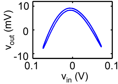
Figure A.4: Illing et al. circuit characterization. Characterization of v_{\text{out}} for a given v_{\text{in}} at 13 MHz with v_{\text{b}} = 0.7 V. In addition to the tent-like properties of v_{\text{out}} , the output voltage of the previous circuit is ac-coupled and therefore centered around v_{\text{out}} = 0 V.
