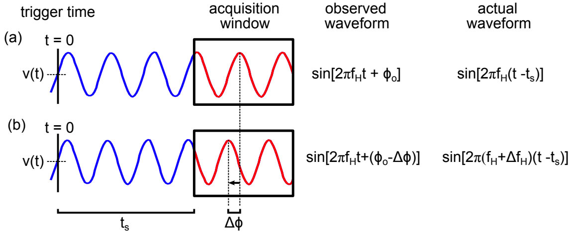
Figure 3.9: Trigger skew technique for measuring small frequency shifts. (a) The periodic sine wave v(t) with frequency f_H triggers the oscilloscope at the trigger time t = 0 , which then displays the observed waveform after a trigger skew time t_s in red on the acquisition window. (b) After a small frequency shift \Delta f_H , the sine wave triggers the oscilloscope and, within the acquisition window, there appears an observed phase shift \Delta\phi that can be used with t_s and f_H to recover the value of the frequency shift \Delta f_H with high precision.
