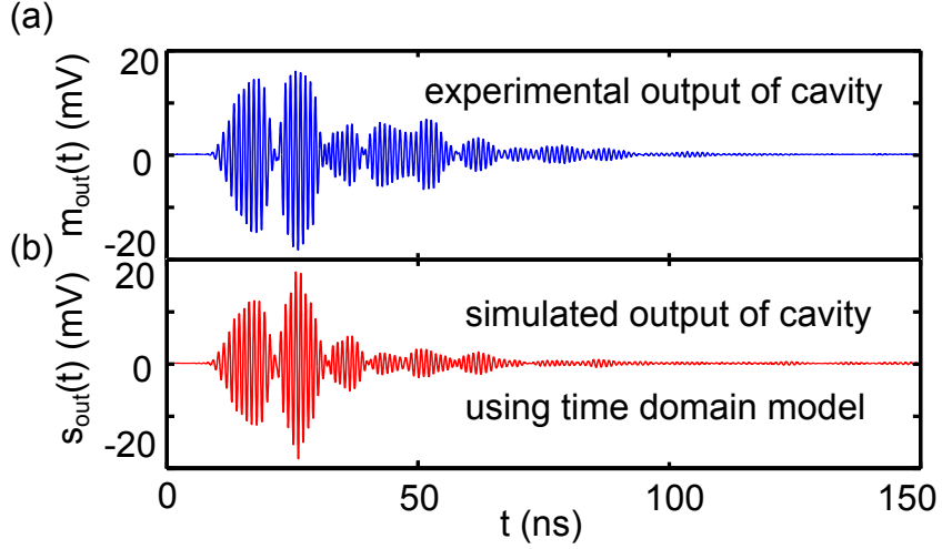
Figure 4.12: Time domain simulations of the cavity. (a) Experimental output m_{\text{out}}(t) and (b) time-domain simulation of s_{\text{out}}(t) using \tau_{\text{max}} = 200 ns.
