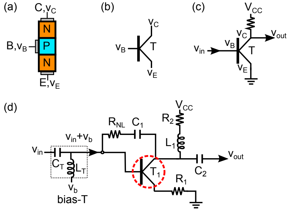
Figure A.1: Bipolar junction transistor in the nonlinear circuit. (a) Bipolar junction transistor with NPN junctions. The base (B), emitter (E), and collector (C) plates each have applied voltages v_B , v_E , and v_C , respectively. (b) The circuit symbol for a transistor (T) with the corresponding voltages labeled. (c) Transistor circuit illustrating how the output voltage v_{out} can change as a function of the input voltage v_{in} . (d) Circuit schematic for the NLC with the transistor T_1 highlighted by the red dotted circle (see Ch. 2 for details). The capacitor C_T and inductor L_T represent the bias-T (grey dotted box) that adds the voltages v_{in} and v_b
