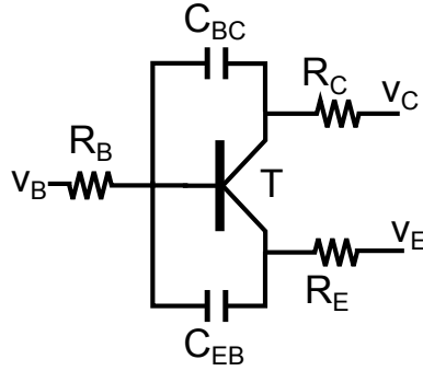
Figure A.2: Schematic of a transistor with capacitive and resistive effects to simulate charge storage in the junctions.
