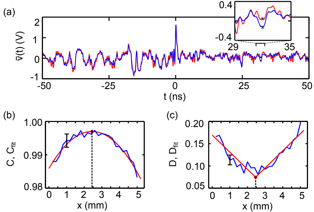
Figure 3.7: 1D sensing with chaos. (a) Chaotic time series \bar{v}(t) acquired from the oscilloscope with a high level trigger and the scatterer at x_{\text{rel}} = 0 mm (blue curve) and x_{\text{rel}} = 5 mm (red curve). The error bars represents the standard deviation of the waveform \pm 20 mV for 50 consecutive measurements at a fixed scatterer location. (b) Normalized cross-correlation coefficients C(\bar{v}(x_n, t), \bar{v}(x^*, t)) as a function of x (blue curve) with the curve C_{\text{fit}}(x) indicating the position of the fitted maximum of the data (red curve). (c) Difference coefficients D(\bar{v}(x_n, t), \bar{v}(x^*, t)) as a function of x (blue curve) with the curve D_{\text{fit}}(x) indicating the position of the fitted minimum of the data (red curve). The errors bars in (b) and (c) represent the standard deviations of C and D for 50 consecutive measurements at fixed scatterer position. The position error in x is \pm 5 \mu\text{m} given by the translation stage (Zaber Technologies TLR150B).
