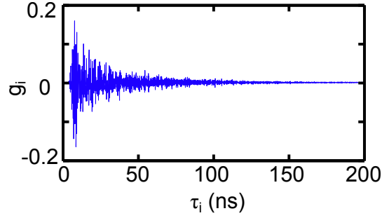
Figure 4.18: Delay-gain distribution of the cavity-feedback system. The pulse response g_i = r_{\text{out}}(\tau_i) with \tau_{\text{max}} = 200 ns.
