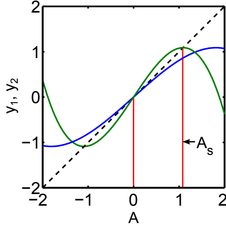
Figure 5.6: Steady-state solutions of the amplitude equation. (a) Intersections of the curve y_1 = F(\bar{G}A) (blue for \bar{G} = 0.9 and green for \bar{G} = 1.5 ) and y_2 = A (dotted line) give the steady state solution A_s for a stable limit cycle of the system.
