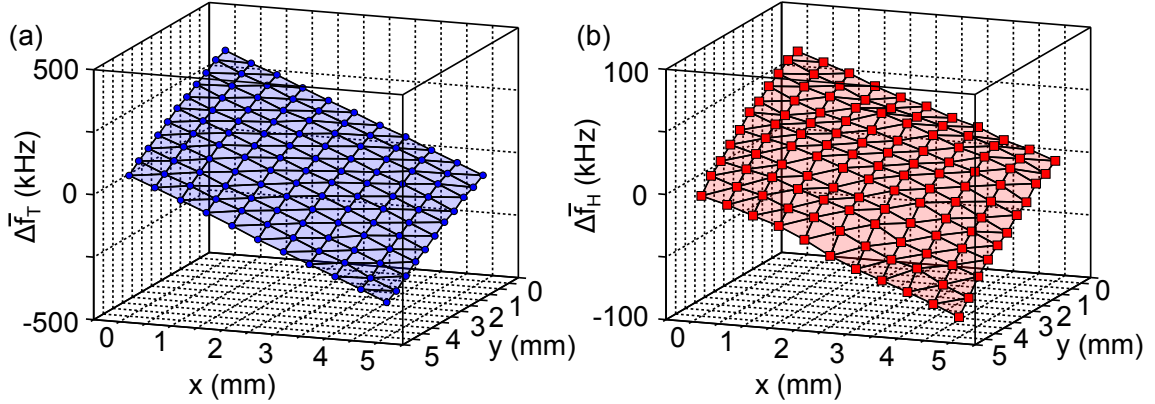
Figure 3.16: 2D sensing with quasiperiodicity. Frequency shifts (a) \Delta\bar{f}_T and (b) \Delta\bar{f}_H as a function of scatterer locations (x, y) in a 5 mm \times 5 mm grid of positions. The mean of each of the frequency shifts has been subtracted for easier comparison.
