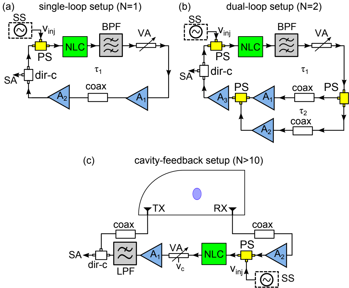
Figure 5.12: Experimental setups for measuring the closed-loop transfer functions in the (a) single-loop feedback system ( N = 1 ), (b) dual loop feedback system ( N = 2 ), and (c) cavity-feedback system ( N > 10 ). In the setups, the following components are used: band-pass filter (BPF, Mini-Circuits ZBFV-925+), low-pass filter (LPF, Mini-Circuits ZBFV-925+ and Mini-Circuits ZBFV-925+), amplifier A_1 (Mini-Circuits ZX60-3016E+), amplifier A_2 (Mini-Circuits ZX60-3016E+), amplifier A_3 (Mini-Circuits ZX60-4018G+ and Picosecond Pulse Labs 5828-108), directional coupler (dir-c, Mini-Circuits ZX30-9-4+), power splitters PS_1 and PS_2 (PS, Picosecond Pulse Labs 5331-104), power splitter PS_2 (Mini-Circuits ZFRSC-42+), variable attenuator (VA, Mini-Circuits ZX73-2500+), swept source (SS, Agilent E8267D), and a spectrum analyzer (SA, Agilent E4440A). In the AM method, a second source (Tektronix AFG 3251) and a mixer (Mini-Circuits ADEX-10L) is used for the modulation.
