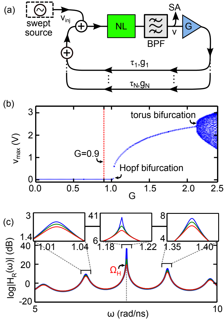
Figure 5.3: Implementing the resonance method. (a) General setup for measuring the magnitude of H_R(\omega) . (b) Bifurcation diagram illustrating the Hopf and torus bifurcation points with respect to the gain G . (c) H_R(\omega) for G = 0.9 (red), G = 0.95 (green), and G = 0.99 (blue). In each of these three cases, the global maximum occurs at approximately the same frequency labeled by \Omega_{H,R} .
