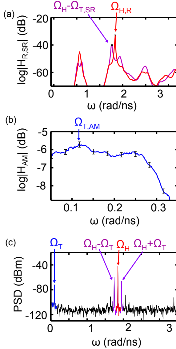
Figure 5.14: Experimental tests of the prediction methods in the cavity-feed-back system. (a) The resonance (R) and shifted resonance (SR) methods, (b) the amplitude modulation (AM) method, and (c) the frequency spectrum of the experiment after the Torus bifurcation. In all of the plots, the relevant \Omega_H , \Omega_T , predictions, and linear combinations are labeled. The frequency resolution in (a) is 0.018 rad/ns, in (b) is 0.002 rad/ns, and in (c) is 0.002 rad/ns. The error bars in (a) indicate the accuracy \pm 0.4 dBm of the spectrum analyzer and in (b) indicate the standard deviation in |H_{AM}(\omega)| for a given \omega .
