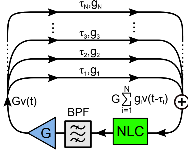
Figure 4.16: Pictorial representation of the cavity-feedback system model. The model for the nonlinear circuit (NLC) drives the band-pass filter (BPF) model of the external loop. The BPF output v(t) drives the delay-gain distribution (\tau_i, g_i) , which is summed at the input of the NLC.
