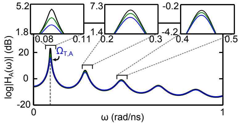
Figure 5.7: Scaling of the closed-loop transfer function magnitude for the amplitude equation. (a) H_A(\omega) for G = 0.9 (blue), G = 0.95 (green), and G = 0.99 (black). In each of these three cases, the global maximum occurs at approximately the same frequency labeled by \Omega_{T,A} .
