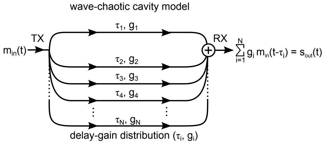
Figure 4.11: Representation of the cavity model in the time domain. The signal m_{\text{in}}(t) is divided among the delay-gain distribution through paths with propagation delays \tau_i and gain coefficients g_i = r_{\text{out}}(\tau_i) . The result is summed at the output of the cavity. The points representing the TX and RX antennas are labeled accordingly.
