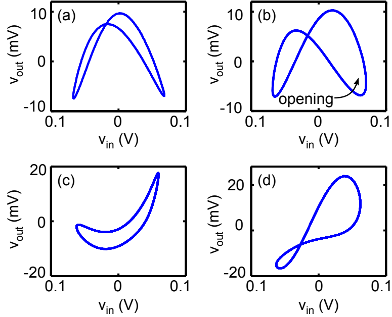
Figure A.5: Distortions from the Illing et al. circuit. Input voltages v_{in} versus output voltages v_{out} in the circuit from Ref. [22] for sinusoidal driving waveforms at frequencies (a) f = 50 MHz, (b) f = 100 MHz, (c) f = 500 MHz, and (d) f = 800 MHz. The opening of the tent-like function is highlighted in (b).
