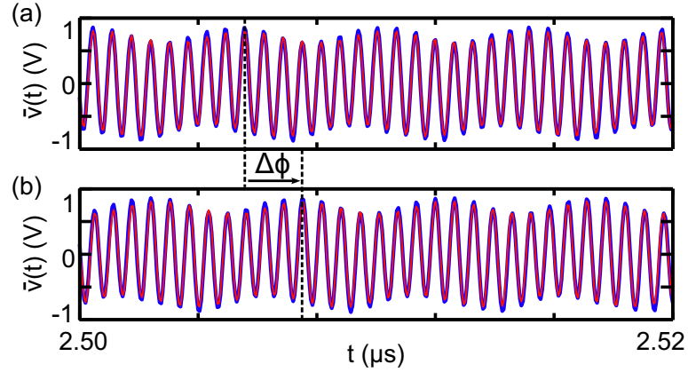
Figure 3.13: Fitted quasiperiodic dynamics on the delayed acquisition window of the oscilloscope with trigger skew t_s = 2.5 \mu s . The averaged signals \bar{v}(t) (blue curves) and fitted function (red curves) for scatterer positions (a) x_{\text{rel}} = 0 \text{ mm} and (b) x_{\text{rel}} = 2 \text{ mm} . The phase shift of the amplitude modulation is marked by \Delta\phi .
