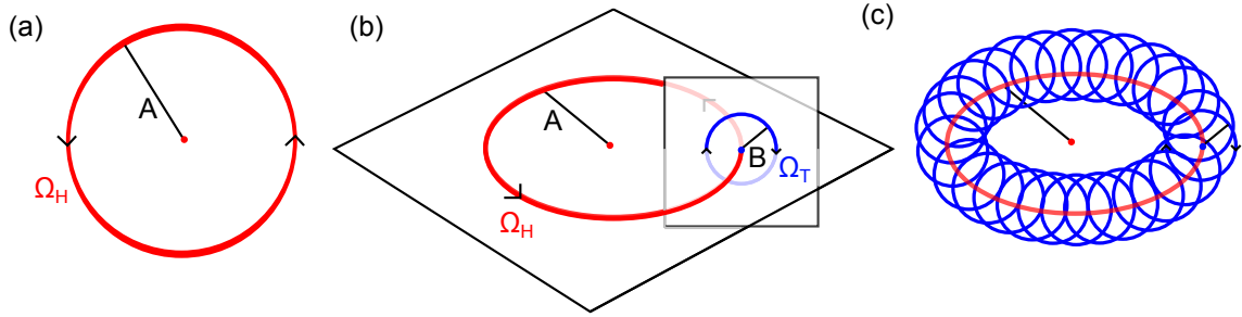
Figure C.3: Phase-space illustrations of Hopf and torus bifurcations. (a) Representation of a super-critical Hopf bifurcation to a limit cycle with Hopf frequency \Omega_H and amplitude A . (b) Representation of a torus bifurcation with torus frequency \Omega_T and amplitude B with (c) the resulting torus.
