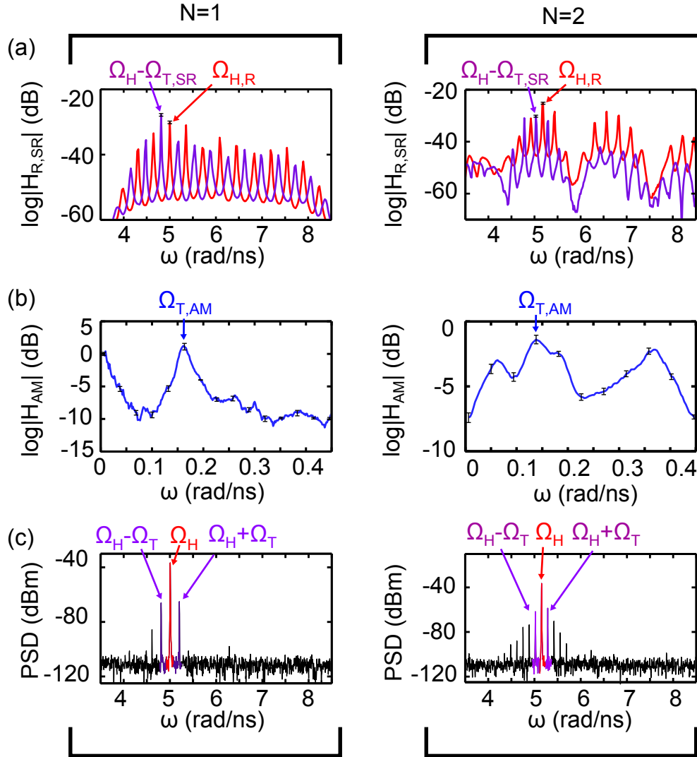
Figure 5.13: Experimental tests of the prediction methods in systems with one and two feedback loops. The N = 1 and N = 2 cases for (a) the resonance (R) and shifted resonance (SR) method, (b) the amplitude modulation (AM) method, and (c) the quasiperiodic frequency spectra of the experiments for the N = 1 and N = 2 cases after their respective Torus bifurcations. In all of the plots, the relevant \Omega_H , \Omega_T , and linear combinations are labeled. The frequency resolution in (a) is 0.025 rad/ns for N = 1 and 0.016 rad/ns for N = 2 , in (b) is 0.002 rad/ns for N = 1 and 0.003 rad/ns for N = 2 , and in (c) is 0.003 rad/ns for N = 1 and N = 2 . The error bars in (a) indicate the accuracy \pm 0.4 dBm of the spectrum analyzer and in (b) indicate the standard deviation in |H_{AM}(\omega)| for a given \omega .
