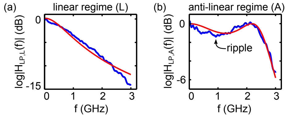
Figure 4.5: Magnitudes of the transfer functions through the nonlinear circuit in its (a) linear regime using v_b = 0.65 V and v_{in} with amplitude of 20 mV, and (b) in its anti-linear regime using v_b = 0.85 V and v_{in} with amplitude of 20 mV. The experimental data (blue curves) in (a) and (b) are fitted with the magnitudes of the transfer functions H_{LP,L}(f) and H_{LP,A}(f) (red curves), respectively. The largest discrepancies between the fits and the respective data occur at f = 3.0 GHz with a difference of 2.3 dB for H_{LP,L}(f) and at f = 0.42 GHz with a difference of 0.8 dB for H_{LP,A}(f) , which present possible sources of error in the NLC model.
