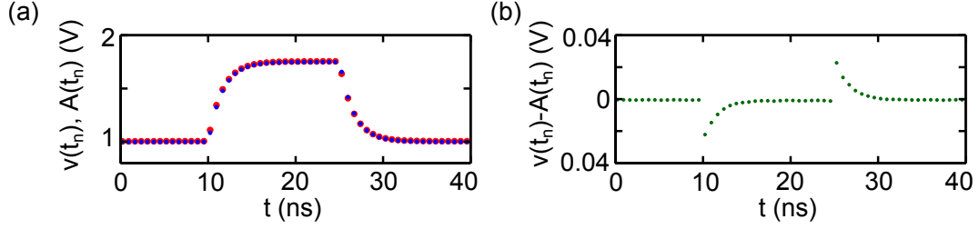
Figure C.5: Comparison of band-pass filter and low-pass filter outputs. (a) Sampled points v(t_n) (blue) and A(t_n) (red) at times t_n , where v(t_n) are the local maxima of v(t) . (b) The differences (v(t_n) - A(t_n)) at each of the times t_n . Note the vertical axis change from (a) to (b).
