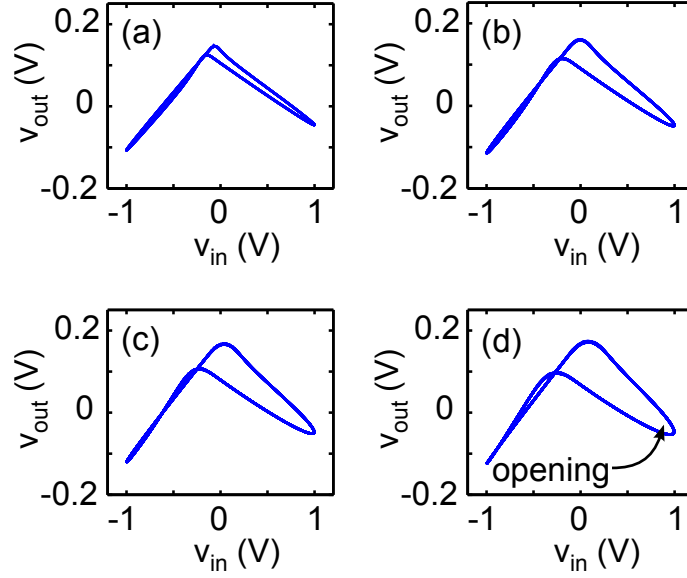
Figure A.8: Distortions in the RLC model for low depletion capacitances. Input voltages v_{in} versus output voltages v_{out} in the RLC circuit model for sinusoidal driving signals at frequencies (a) f = 500 MHz, (b) f = 1.1 GHz, (c) f = 1.5 GHz, and (d) f = 1.9 GHz with the depletion capacitances C_{BE} = 500 fF and C_{BC} = 500 fF.
