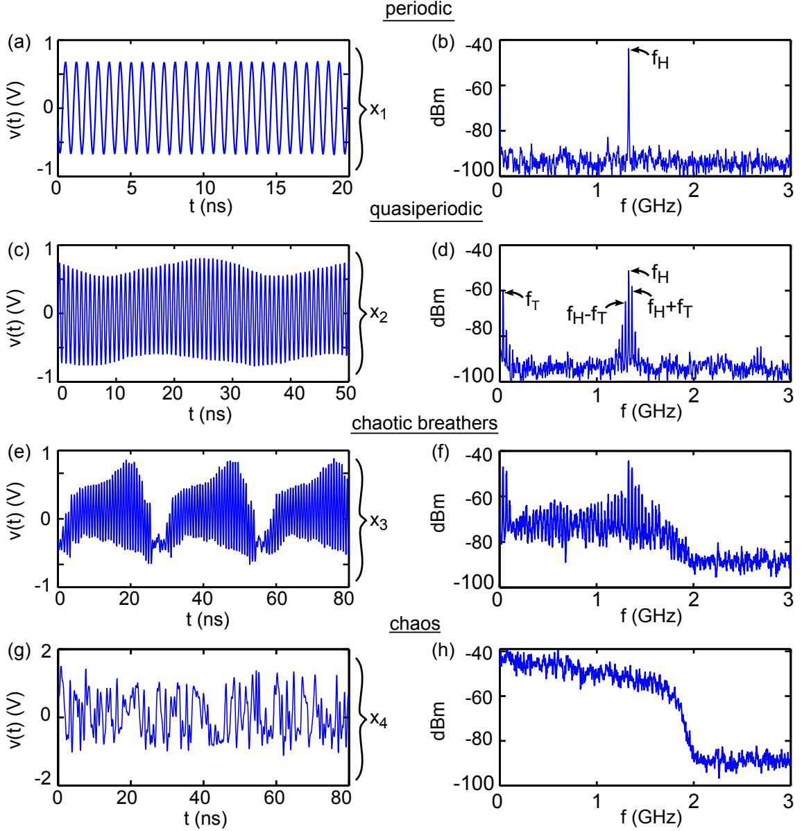
Figure 3.3: Dynamics of the cavity-feedback system. (a), (c), (e), (g) Time series v(t) and (b), (d), (f), (h) power spectral densities (PSDs) with the scatterer at the relative positions x_1 = 1 mm, x_2 = 2 mm, x_3 = 9.5 mm, and x_4 = 11 mm. The noise level in each time series is approximately \sigma_N = 1.2 mV, which is given by the standard of the noise floor of the oscilloscope during the time series acquisition.
