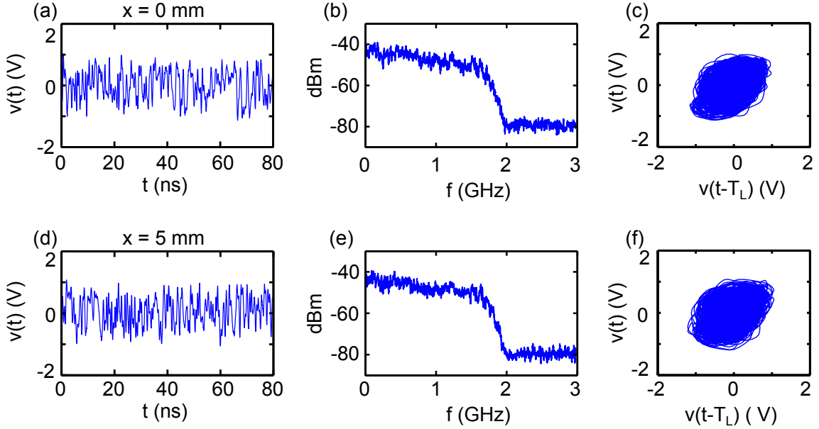
Figure 3.5: Broadband chaos for two different scatterer positions. (a) Chaotic time series, (b) power spectral density (PSD), and (c) phase space projection (PSP) when the scatterer is at position x_{\text{rel}} = 0 mm. (d) Chaotic time series (d) PSD, and (f) PSP when the scatterer is at position x_{\text{rel}} = 5 mm. In the PSPs, the time lag T_L = 0.3 ns.
