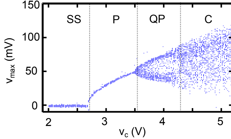
Figure 2.5: Single-loop bifurcation diagram. The local maxima v_{\max} plotted as a function of the control voltage v_c . Vertical grey dashed lines separate steady-state (SS), periodic (P), quasiperiodic (QP), and chaotic (C) regions of the dynamics. For these measurements, the discretization error of v_{\max} from the digital oscilloscope is approximately 100 \mu\text{V} , the noise floor standard deviation is approximately 1.2 \text{ mV} , and the control voltage v_c is varied in steps of 20 \pm 2 \text{ mV} .
