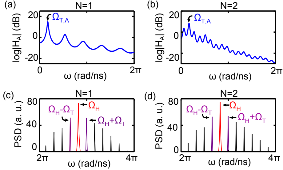
Figure 5.8: Predicting the torus bifurcation frequencies using the closed-loop transfer function of the amplitude equation. (a) Simulated |H_A(\omega)| for the case of N = 1 with parameters \omega^{(+)} = 10.7 rad/ns, \omega^{(-)} = 8.2 rad/ns, G = 0.9 , g_1 = 1 , and \tau_1 = 5 . (b) Simulated |H_A(\omega)| for the case of N = 2 with parameters \omega^{(+)} = 10.7 rad/ns, \omega^{(-)} = 8.2 rad/ns, G = 0.9 , g_1 = 0.2 , g_2 = 0.3 , and \tau_1 = 5 , and \tau_2 = 12 . PSD of the quasiperiodic solutions to Eq. (6.3) when the gain is tuned up to G = 2.4 for the (c) N = 1 case and G = 4.8 for the (d) N = 2 case.
