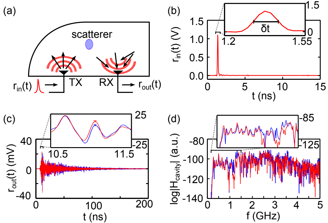
Figure 2.15: Pulse response. (a) Experimental measurement of the pulse response r_{out}(t) of the cavity using a short EM pulse r_{in}(t) . (b) Input pulse r_{in}(t) with full width at half maximum of \sim 100 ps (generated using the error performance analyzer Agilent 70843). (c) Pulse responses r_{out}(t) with (red curve) and without (blue curve) the scatterer. Error bars indicate the standard deviation of the noise floor ( \pm 1 mV) of the oscilloscope for each measurement. (d) Cavity spectra |H_{cavity}(f)| with (red curve) and without (blue curve) the scatterer. In the zoom of (d), the horizontal axis is from 0.2 GHz to 1.5 GHz. In (c) and (d), zooms of the waveforms highlight some of the small quantitative changes in the system when the scatterer is added.
