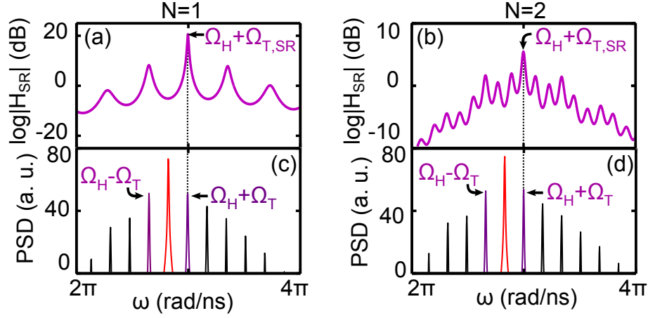
Figure 5.10: Shifted resonance method for predicting the torus frequencies. (a) Simulated |H_{SR}(\omega)| for the case of N = 1 with parameters \omega^{(+)} = 10.7 rad/ns, \omega^{(-)} = 8.2 rad/ns, G = 0.9 , g_1 = 1 , and \tau_1 = 5 . (b) Simulated |H_{SR}(\omega)| for the case of N = 2 with parameters \omega^{(+)} = 10.7 rad/ns, \omega^{(-)} = 8.2 rad/ns, G = 0.9 , g_1 = 0.2 , g_2 = 0.3 , \tau_1 = 5 ns, and \tau_2 = 12 ns. (c)-(d) Repeat of Figs. 5.8c-d.
