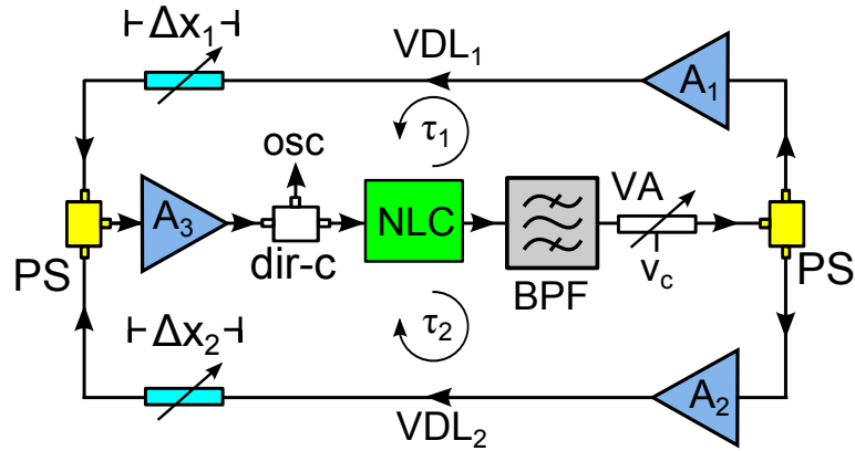
Figure 1.10: Two-delay nonlinear feedback system with time delays \tau_1 and \tau_2 . The dual-delay nonlinear system uses a nonlinear circuit (NLC), power splitters (PS), a variable attenuator (VA) with control voltage v_c , amplifiers A_i , two variable delay lines (VDLs), a band-pass filter (BPF), and a directional coupler (dir-c) in its feedback, where the feedback signal is measured using an oscilloscope (osc). The values of the time-delays \tau_1 and \tau_2 are adjusted using coaxial waveguides of tunable lengths \Delta x_1 and \Delta x_2 , respectively.
