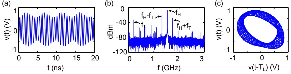
Figure 3.12: Quasiperiodic dynamics used for imaging. (a) Temporal evolution v(t) of a typical quasiperiodic state used for position sensing. In the time series, the signal-to-noise ratio is \text{RMS}_S/\text{RMS}_N \sim 150 , where \text{RMS}_S ( \text{RMS}_N ) is the root-mean-square of the signal (noise) (b) Power spectral density (PSD) of this signal with Hopf and torus frequencies labeled f_H and f_T , respectively, as well as the harmonics f_H \pm f_T (c) Phase space projection with time lag T_L = 1.55 ns.
