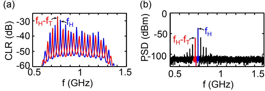
Figure 1.9: Closed-loop resonances (CLR) of the nonlinear feedback system with a single time delay showing (a) the predicted values for f_H \sim 796 MHz and f_H - f_T \sim 766 MHz. The blue and red resonances are measured for specific configurations of the nonlinear circuit based on the theory. (b) Power spectral density (PSD) of the quasiperiodic signal with actual f_H \sim 797 MHz and f_H - f_T \sim 767 MHz labeled in blue and red, respectively.
