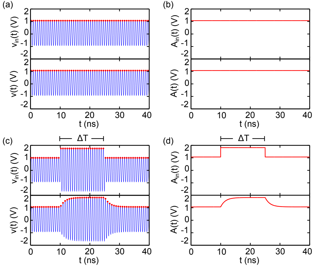
Figure C.4: Example of the dynamics from the amplitude equation in an open-loop configuration. (a) The oscillatory waveform v_{in}(t) with constant amplitude drives an open-loop band-pass filter (Eq. C.34) with parameters \omega^{(-)} = 8.2 rad/ns, \omega^{(+)} = 9.4 rad/ns and central frequency \omega_o = 8.8 rad/ns. The output of the band-pass filter shows an oscillatory v(t) with a constant amplitude. (b) A constant input waveform A_{in}(t) drives an open loop low-pass filter (Eq. C.35) with bandwidth \Delta/2 , where \Delta = \omega^{(+)} - \omega^{(-)} = 1.3 rad/ns to produce a constant output A(t) . (c) Input waveform v_{in}(t) drives the band-pass filter with a square wave amplitude (of width \Delta T ) to produce the response v(t) . (d) The square wave A_{in}(t) drives the low-pass filter to produce the response A(t) . The local maxima in v_{in}(t) and v(t) are labeled with red dots.
