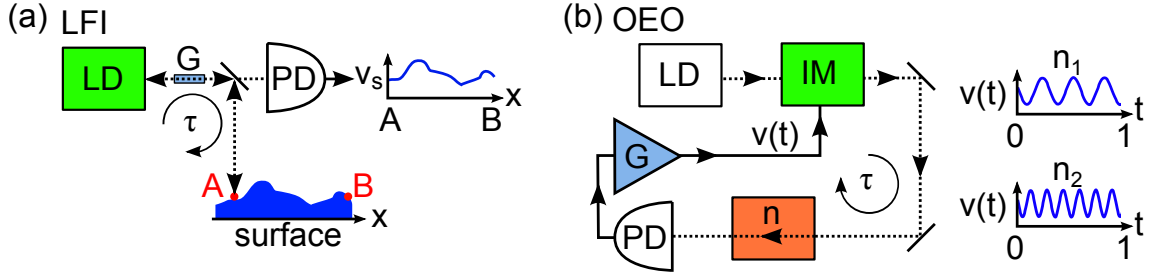
Figure 2.9: Time-delayed nonlinear feedback sensors. (a) Laser feedback interferometry (LFI) system. The gain of the feedback loop G is determined by an attenuator at the output of the LD. As the point of reflection on the surface scans from A to B , the time-delay \tau of the nonlinear feedback system changes such that v_s reveals the surface profile when plotted as a function of x . (b) Index of refraction sensor using an opto-electronic oscillator (OEO) with a LD, interference modulator (IM), and photodetector (PD). The gain of the feedback loop is determined by an amplifier ( G ). As the index of refraction changes from n_1 to n_2 , the net delay \tau of the nonlinear feedback loop decreases ( n_2 < n_1 ) and thus the frequency of oscillation in v(t) increases. The position x and time t are in arbitrary units.
