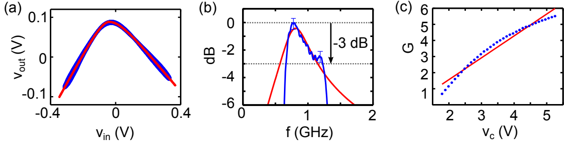
Figure 2.6: Model parameters. (a) Numerical fitting of the nonlinear function F(v) (red curve) to the experimental nonlinearity of the nonlinear circuit (blue curve). (b) Bandwidth of experimental system (blue curve) used for determining the model parameters f^{(+)} and f^{(-)} of the fitted transfer function magnitude |H_{BP}(f)| (red curve). The error bar indicates the accuracy of \pm 0.4 dB for the spectrum analyzer (Agilent E4440A), and the resolution of the frequency sweep is approximately 4 MHz. (c) Linear fit (red curve) of the experimental gain G as a function the control voltage v_c . The error bars for each measurement of G represent the fluctuations in the measured waveforms but do not extend beyond the data points, and the control voltage v_c is varied in steps of 100 \pm 2 mV.
