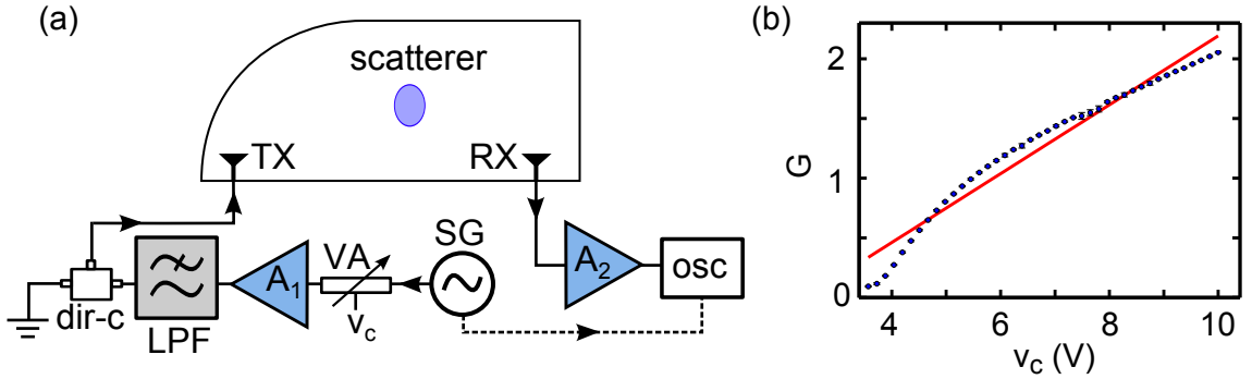
Figure 4.15: Measurements of the net gain of the feedback loop. (a) Experimental setup for measuring the gain of the entire feedback loop. (b) The net gain G as a function of v_c , which is measured using a sinusoidal waveform with frequency f = 1.35 GHz, the dominant frequency in the dynamics (see next subsection). The error bars for each measurement of G represent the fluctuations in the measured waveforms and the control voltage v_c is varied in steps of 160 \pm 2 mV.
