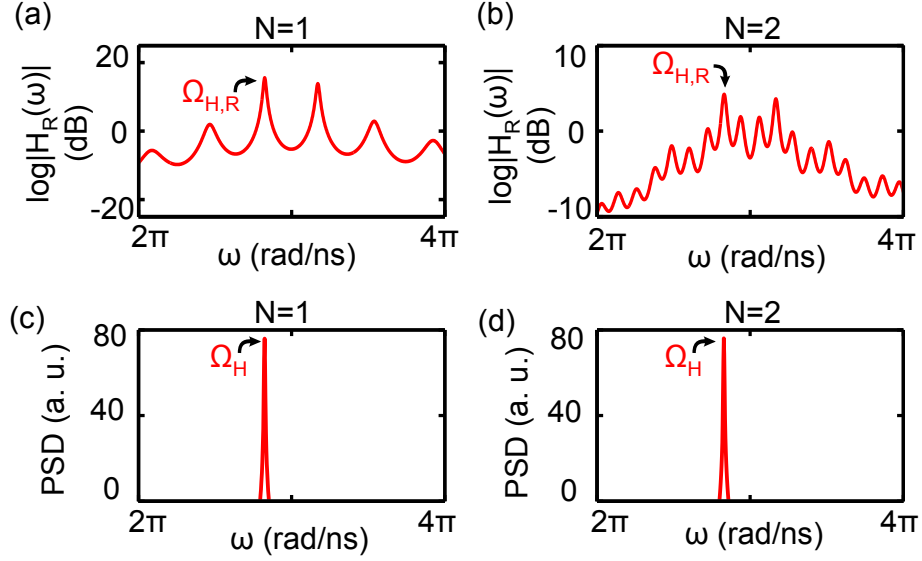
Figure 5.4: Predicting the first Hopf bifurcation frequency using the resonance method. (a) Simulated |H_R(\omega)| for the simplest case of N = 1 with parameters \omega^{(+)} = 10.7 rad/ns, \omega^{(-)} = 8.2 rad/ns, G = 0.9 , g_1 = 1 , and \tau_1 = 5 ns. (b) Simulated |H_R(\omega)| for the case of N = 2 with parameters \omega^{(+)} = 10.7 rad/ns, \omega^{(-)} = 8.2 rad/ns, G = 0.9 , g_1 = 0.2 , g_2 = 0.3 , \tau_1 = 5 ns, and \tau_2 = 12 ns. Power spectral density (PSD) of the periodic solutions to Eq. (6.3) when the gain is tuned up to G = 1.45 for the (c) N=1 case and G = 2.6 for the (d) N = 2 case.
