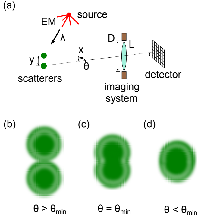
Figure 1.2: Limitations of imaging due to diffraction. (a) The incident EM radiation of wavelength \lambda from a source interacts with two point-light scatterers that are separated by a distance y . An imaging system with a circular aperture of diameter D (and lens L ) and an array detector is placed a distance x from the scatterers, forming a scattering angle defined by \theta . (b) For \theta > \theta_{\min} , the diffraction patterns of from the scatterers are well resolved, (c) for \theta = \theta_{\min} , the diffraction patterns are partially resolved, and (d) for \theta < \theta_{\min} , the patterns are indistinguishable, where \theta_{\min} is defined by Eq. (1.1).
