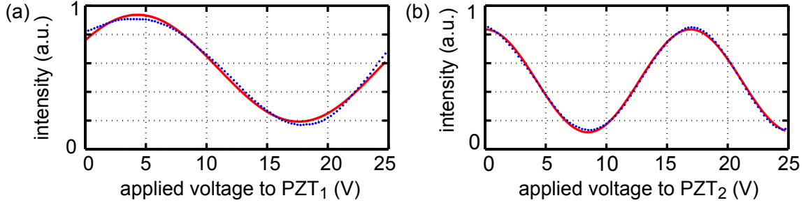
Figure D.3: Piezoelectric transducer calibration. (a) Output intensity of the interferometer (a) for a fixed PZT 2 while a voltage is applied to PZT 1 and (b) for a fixed PZT 1 while a voltage is applied to PZT 2 . The experimental data (blue dots) are fitted (red curves) to yield conversion factors of K_1 = 29.2 \pm 0.1 nm/V for PZT 1 and K_2 = 45.8 \pm 0.2 nm/V for PZT 2 .
