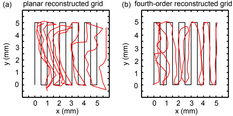
Figure 3.17: Reconstructed calibration grids (a) using a planar mapping and (b) a fourth-order mapping between frequency shifts ( \Delta f_T, \Delta f_H ) and the scatterer position (x, y) . The reconstructed grids are shown in red and the actual path used for the calibration grid is shown in black.
