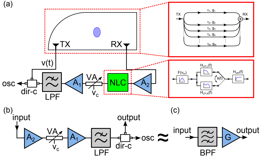
Figure 4.13: Review of cavity-feedback system. (a) Experimental setup for the cavity-feedback system with the cavity and nonlinear circuit (NLC) highlighted in red and their corresponding graphical representations. In addition, a variable attenuator (VA) is added to the external feedback loop to control the gain of the system for a fixed scatterer position. (b) All of the elements of the external feedback loop, except for the NLC, can be modeled as a single lumped element with properties similar to each of the components in series. (c) The lumped element in (b) can be modeled as a band-pass filter (BPF) with gain G .
