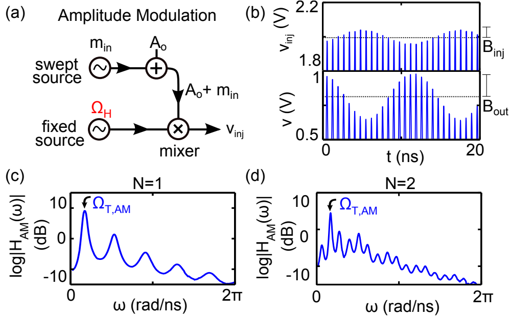
Figure 5.9: Amplitude modulation method for predicting the torus frequencies. (a) AM source produces an amplitude modulated waveform v_{inj} at carrier frequency \Omega_H and tunable modulation frequency \omega . (b) Typical modulation amplitudes in v_{inj} and v from the system with linearized feedback about A_o . The modulation amplitudes B_{inj} and B_{out} are labeled with vertical bars. Closed-loop transfer functions for the amplitude equation using A_o = 2 , B_{inj} = 0.05 , G = 0.9 for the previous (c) N = 1 and (d) N = 2 cases. Note that each point in these plots is the result of a separate simulation.
