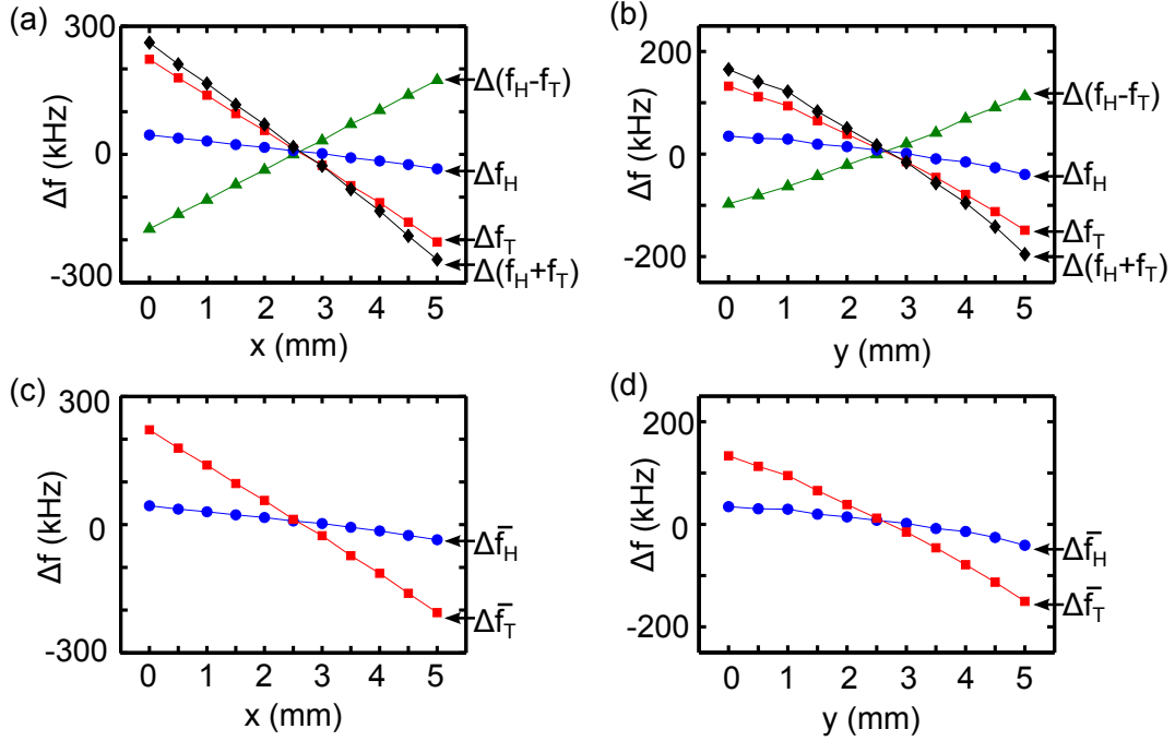
Figure 3.14: 1D sensing with quasiperiodicity. Frequency shifts \Delta f_T (red squares), \Delta(f_H - f_T) (green triangles), \Delta f_H (blue circles), and \Delta(f_H + f_T) (black diamonds) as a function of scatterer position in the (a) x and (b) y directions. The mean of each frequency shift is removed for easier comparison. Averaged frequency shifts \Delta \bar{f}_T (red squares) and \Delta \bar{f}_H (blue circles) as a function of (c) x direction, where the fit from Eq. (3.8) yields a_1 = 2.8 mm/kHz, a_2 = -8.7 mm/kHz, c_0 = 27,113.0 mm, c_1 = -439.2 and c_2 = 1.5 mm ^{-1} , and (d) along the y direction, where the fit from Eq. (3.9) yields b_1 = 0.8 mm/kHz, b_2 = -0.5 mm/kHz, d_0 = -73,452.0 mm, d_1 = 242.0 , and d_2 = -2.0 mm ^{-1} . The error in the measurement of each frequency is \sim 3 kHz, which is smaller than the size of the data points.
