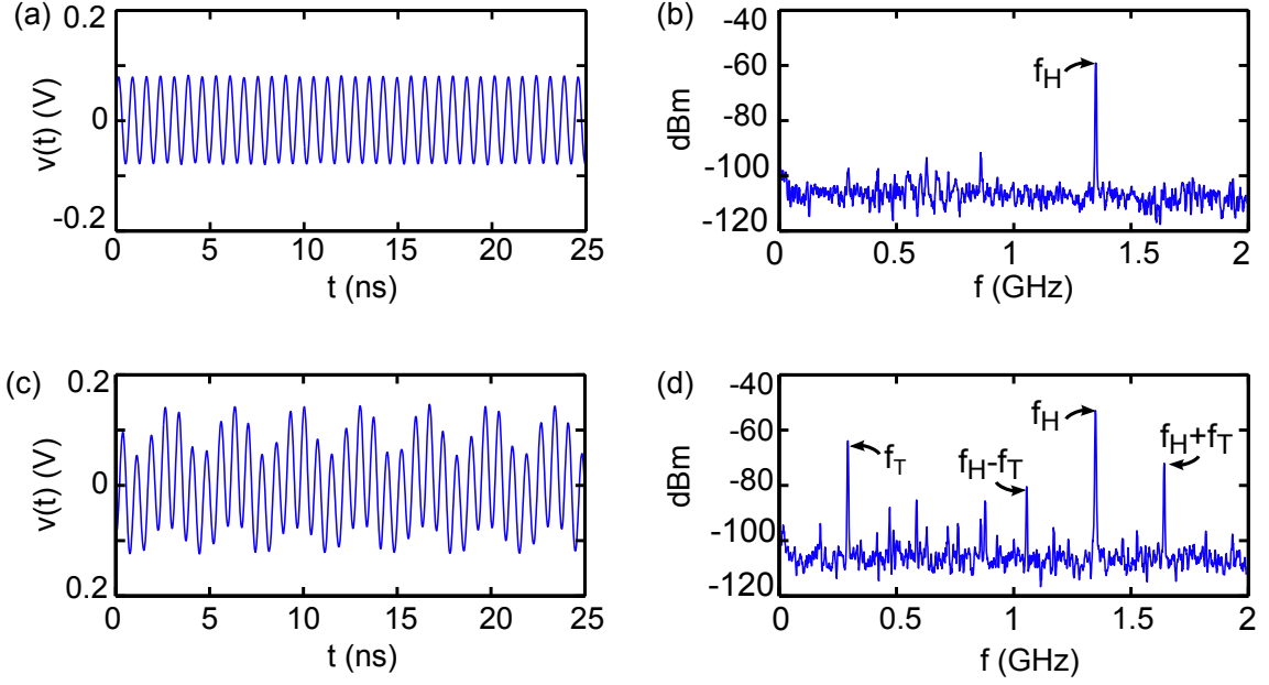
Figure 4.17: Experimental cavity-feedback system dynamics. (a) Periodic time series and (b) power spectral density (PSD) of v(t) for G \sim 1.5 . (c) Quasiperiodic time series and (d) PSD for G \sim 2 . In the experiment, the bias voltage in the nonlinear circuit is v_b = 0.9 V.
