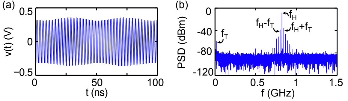
Figure 6.3: Two-delay experimental quasiperiodic dynamics. (a) Temporal evolution and (b) power spectral density (PSD) of typical quasiperiodic dynamics. In the time series, the signal-to-noise ratio is \text{RMS}_S/\text{RMS}_N \sim 80 , where \text{RMS}_S ( \text{RMS}_N ) is the root-mean-square of the signal (noise). See Ch. 3 for a comparison of this value. In the PSD, the angular frequencies associated with the Hopf and Torus bifurcations and their linear combinations are labeled accordingly.
