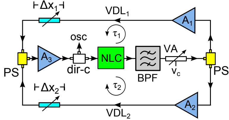
Figure 6.2: Two-delay experimental feedback system. The output of the nonlinear circuit (NLC) drives a band-pass filter (BPF, Mini-Circuits ZBFV-925+), a variable attenuator (VA, Mini-Circuits ZX73-2500+), a power splitter (PS, Picosecond Pulse Labs 5331-104), amplifiers A_1 and A_2 (both are Mini-Circuits ZX60-3016E+), variable delay-lines VDL_1 and VDL_2 , a second PS, a third amplifier A_3 (Mini-Circuits ZX60-4018G+ and Picosecond Pulse Labs 5828-108), a directional coupler (dir-c, Mini-Circuits ZX30-9-4+), and the input of the NLC. The VDLs are comprised of coaxial waveguides known as line stretchers (Microlab/FXR SR-05B) that are attached to linear translation stages (each are Zaber Technologies TLSR150B) with relative length changes \Delta x_i . A portion of the signal in the feedback loop is measured as the voltage v(t) on the oscilloscope (osc).
