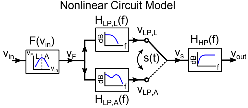
Figure 4.6: Schematic representation of the NLC model. The input voltage v_{in} drives the nonlinear function F(v_{in}) = v_F and the low-pass filters H_{LP,L}(f) and H_{LP,A}(f) in parallel. The continuous switching function s(t) switches v_s between the output voltages of these two filters ( v_{LP,L} and v_{LP,A} ), which is then high-pass filtered (by transfer function H_{HP}(f) ) to yield the output voltage v_{out} of the nonlinear circuit. The various blue curves represent the input-output tent-like shape of the nonlinear function F(v_{in}) (with linear (L) and anti-linear (A) regimes labeled) as well as the magnitudes of the different transfer functions as a function of frequency.
