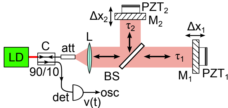
Figure 7.2: Two-delay all-optical feedback system for subwavelength sensing. The output of a laser diode (LD, Sumitomo SLT4416-DP) passes through a collimating lens (L) in free space, separates using a beam splitter (BS), is time-delayed along two separate paths with propagation delays \tau_1 and \tau_2 , and feeds back to itself. Mirrors M_1 and M_2 at the end of these paths are attached to piezoelectric transducers (PZT 1 and PZT 2 , Burleigh PZO-015) to make small adjustments to \tau_1 and \tau_2 , respectively. Using an attenuator (att) and a 90/10 coupler (C), the feedback gain is controlled and the feedback signal is routed to a photodetector (det, New Focus 1544-B) and a high-speed oscilloscope (osc, DSO90804A).
