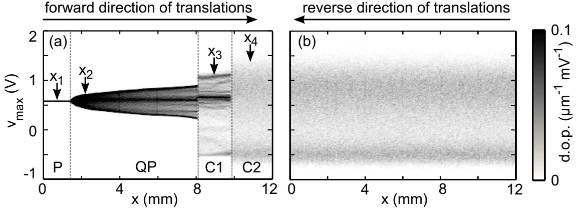
Figure 3.4: Bifurcation diagrams. Density of local maxima v_{\max} plotted as a function of scatterer position x for the (a) forward direction from x_{\text{rel}} = 0 mm to x_{\text{rel}} = 12 mm and the (b) reverse direction from x_{\text{rel}} = 12 mm to x_{\text{rel}} = 0 mm. The color bar indicates the density of points (d.o.p) with a minimum value of 0 \mu\text{m}^{-1} \text{mV}^{-1} indicated in white and the saturation value of 0.1 \mu\text{m}^{-1} \text{mV}^{-1} indicated in black. The positions x_1 , x_2 , x_3 , and x_4 are labeled to indicate the density of the v_{\max} for the dynamics presented in Fig. 3.3.
