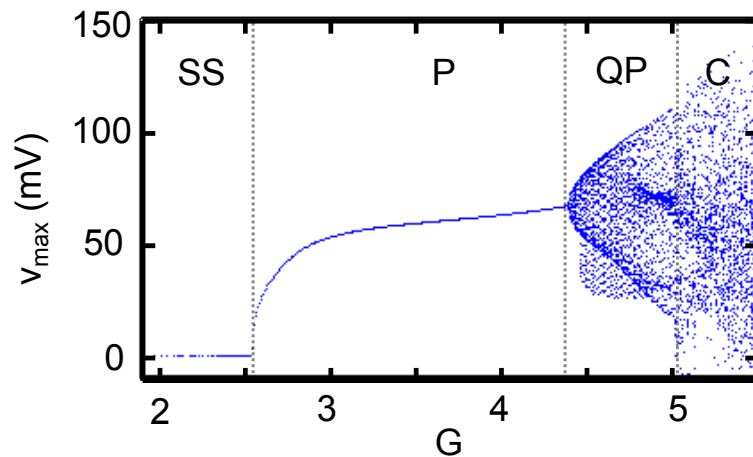
Figure 2.8: Simulated bifurcation diagram. The simulated local maxima v_{\max} plotted as a function of the feedback loop gain G . Vertical grey dashed lines separate steady-state (SS), periodic (P), quasiperiodic (QP), and chaotic (C) regions of the dynamics.
