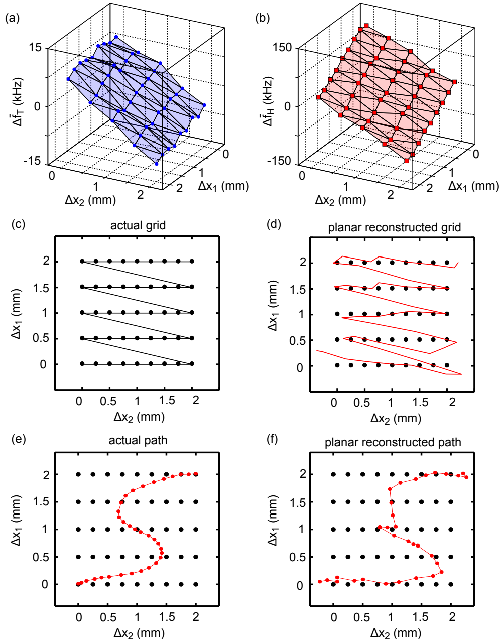
Figure 6.4: Two-delay experimental quasiperiodic frequency shifts. Frequency shifts (a) \Delta\bar{f}_T and (b) \Delta\bar{f}_H as a function of (\Delta x_1, \Delta x_2) . (c) Calibration grid of (\Delta x_1, \Delta x_2) and (d) reconstructed calibration grid (red curve). (e) Test path of (\Delta x_1, \Delta x_2) (red curve) in the 2D grid of points (black dots). (f) Reconstructed path of (\Delta x_1, \Delta x_2) (red curve) using the numerical map in the 2D grid of points (black dots).
