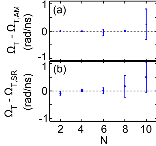
Figure 5.11: Amplitude modulation and shifted resonance methods for determining the torus frequency in cases with multiple delays. For each simulation with N = 2 to N = 10 feedback loops, \tau_i and g_i are sampled from uniform distributions such that 5 \text{ ns} < \tau_i < 50 \text{ ns} and -1 < g_i < 1 . The chosen gains g_i are the renormalized using the condition \sum_{i=1}^N |g_i| = 1 . The bandwidth parameters are chosen to be \omega^{(+)} = 9.4 \text{ rad/ns} and \omega^{(-)} = 6.3 \text{ rad/ns} . The predictions are tested by calculating the torus frequency \Omega_T from the simulated dynamics. The results from the AM method are shown in (a) using G = 0.95 , A_o = 2 and B_{inj} = 0.05 , and the results from the SR method are shown in (b) using G = 0.95 . The predictions are tested by calculating the mean \mu(N) (blue dots) and standard deviation \sigma(N) (error bars) of (\Omega_T - \Omega_{T,AM}) and (\Omega_T - \Omega_{T,SR}) for each N . Note that AM and SR methods use \Omega_H in the predictions of \Omega_{T,AM} and \Omega_{T,SR} . Using \Omega_{H,R} increases the prediction errors.
