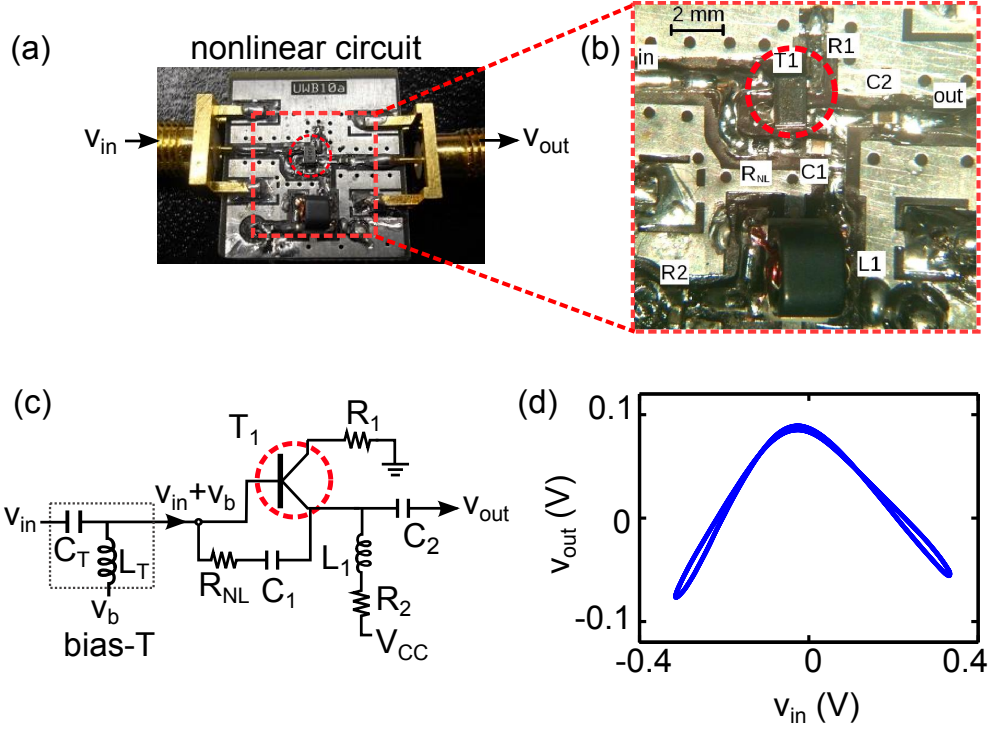
Figure 2.2: Nonlinear circuit. (a) Photograph of the circuit board showing its input and output connectors for voltages v_{in} and v_{out} , respectively. (b) Zoom of the nonlinear circuit indicating the relative locations of the transistor, supply voltage V_{CC} = 1.6 V and the passive components: R_{NL} = 30 \Omega , C_1 = 47 nF, L_1 = 1 \mu\text{H} , R_1 = 5.1 \Omega , R_2 = 68 \Omega , and C_2 = 0.1 \mu\text{F} . The capacitor C_T and inductor L_T represent the bias-T (grey dotted box) that adds the voltages v_{in} and v_b . In (a), (b), and (c), the transistor is highlighted with a red-dotted circle. (d) Tent-like nonlinear operation of the circuit between the voltages v_{in} and v_{out} , where v_{in} is generated using a signal generator (Agilent E8267D) and v_{out} is measured on an oscilloscope (DSO80804A with noise floor standard deviation \sigma \sim 1.2 mV).
