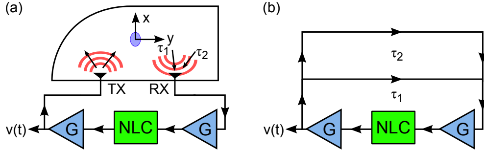
Figure 6.1: Two-delay simplification of the cavity-feedback system. (a) The cavity is approximated as having only two relevant propagation paths with time delays \tau_1 and \tau_2 . In this case, consider that the scatterer's position in x and y determines \tau_1 and \tau_2 , respectively. (b) Schematic representation of a two-delay cavity-feedback system with feedback delays \tau_1 and \tau_2 .
