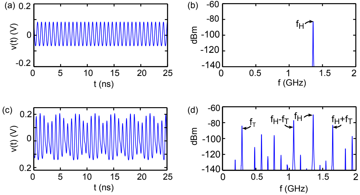
Figure 4.19: Simulated cavity-feedback system dynamics. (a) Periodic time series and (b) power spectral density (PSD) of v(t) for G = 1.5 . (c) Quasiperiodic time series and (d) PSD for G = 2 . The bias voltage in the model for the nonlinear circuit is v_b = 0.9 V.
