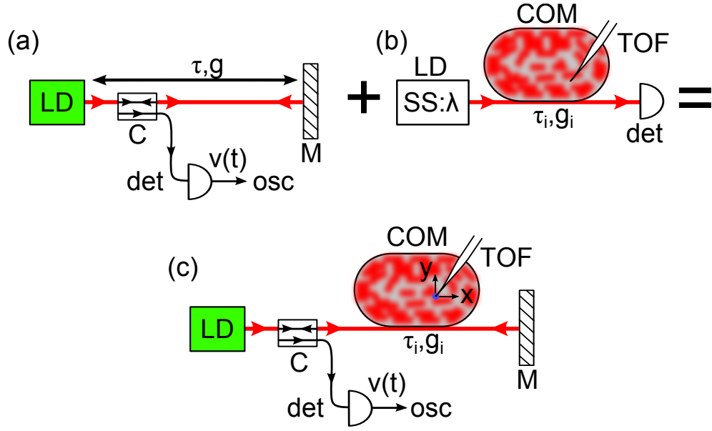
Figure 7.1: Conceptual overview of the all-optical cavity-feedback system. (a) Time-delayed nonlinear feedback in a semiconductor laser diode (LD). The output of LD is reflected by a mirror (M) and fed back to the laser cavity. A portion of the output power drives a coupler (C) for detection (det), which is then recorded as the voltage v(t) on an oscilloscope (osc). (b) The output of LD is coupled to a chaotic optical microcavity (COM). The wavelength of the laser \lambda is varied using a swept source (SS) while the output power is detected and recorded. The resonances of the cavity can be used to detect the presence of a tapered optical fiber (TOF). (c) The emitted light of LD is coupled into COM, reflected by a mirror and fed back to itself. The LD output also passes through a coupler (C) to a detector and oscilloscope, where it is recorded as a time-varying voltage v(t) . The quasiperiodic frequency content of v(t) is used to reconstruct the position (x, y) of TOF.
