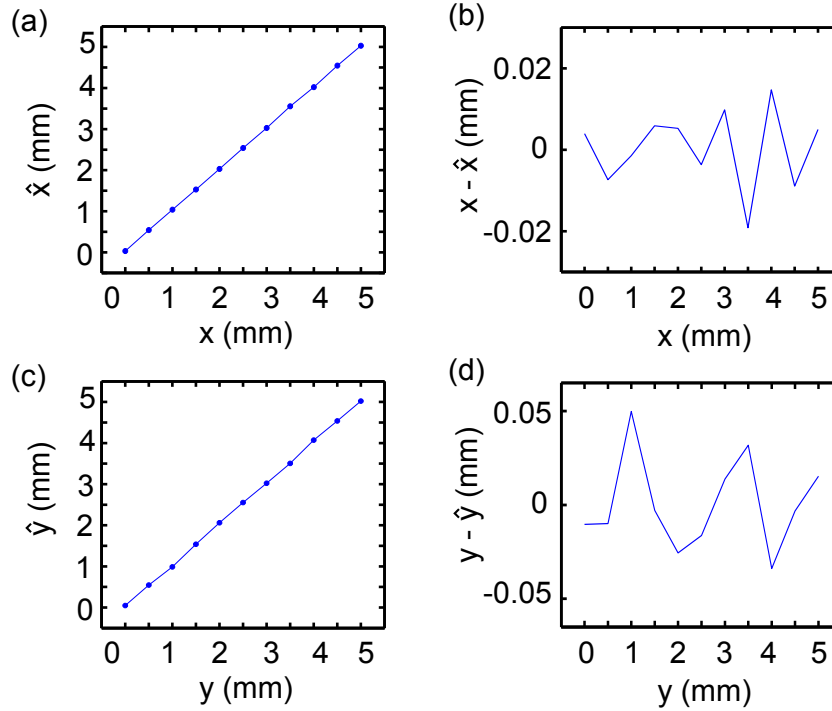
Figure 3.15: 1D predicted positions using quasiperiodicity. (a) Predicted position \hat{x} versus actual position x using the inverted map. (b) Errors of the \hat{x} mapping as a function of x . (c) Predicted position \hat{y} versus actual position y using the inverted map. (d) Errors of the \hat{y} mapping as a function of y .
