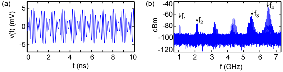
Figure 7.3: Quasiperiodic dynamics of the two-delay optical feedback system. (a) Temporal evolution of v(t) , which represents the laser intensity oscillations: v(t) \propto I(t) = |E(t)|^2 , where I(t) is the intensity of the electric field with amplitude E(t) . (b) Power spectral density (PSD) of the oscillations.
