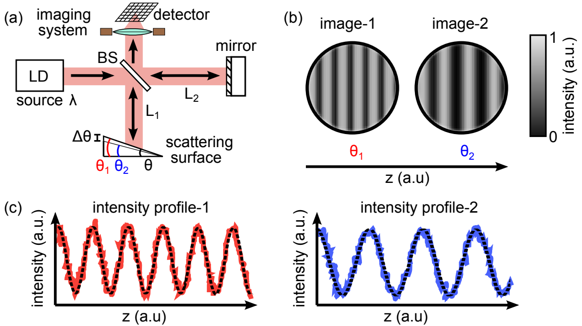
Figure 1.3: Resolving subwavelength features using interferometry. Coherent light of wavelength \lambda from a laser-diode (LD) source is separated using a beam splitter (BS) along two paths, an imaging arm of length L_1 with a reflecting scattering surface and a reference arm of length L_2 with a mirror. The reflected light from each path is focused through the circular aperture of an imaging system and forms an interference pattern on an array detector. (b) Interference patterns of image-1 and image-2 for the scattering angles \theta_1 and \theta_2 , respectively. (c) Cross sections of the interference patterns along the z direction give intensity profile-1 (red) and intensity profile-2 (blue), which are fitted with periodic functions of frequencies f_1 and f_2 (black dashed-curves), respectively, where f_1 > f_2 .
