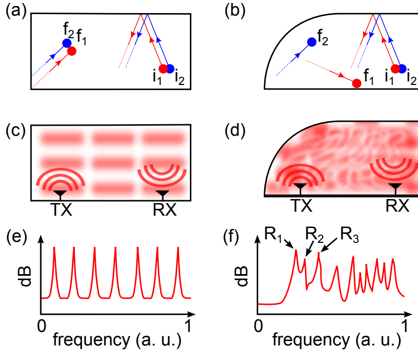
Figure 2.10: Ray and wave chaos. (a) Rectangular and (b) quarter-stadium (QS) 2D billiards with identical particles (red and blue) and their trajectories from initial positions i_1 and i_2 to final positions f_1 and f_2 . Illustrations of the interference patterns from the (c) rectangular and (d) QS cavity. The rectangular cavity contains large nodes or blind spots, indicated in white, when compared to the complex interference pattern in the QS cavity. (e)-(f) Typical frequency resonances of a rectangular and QS wave-chaotic cavities, respectively. The frequency is given in arbitrary units (a. u.).
