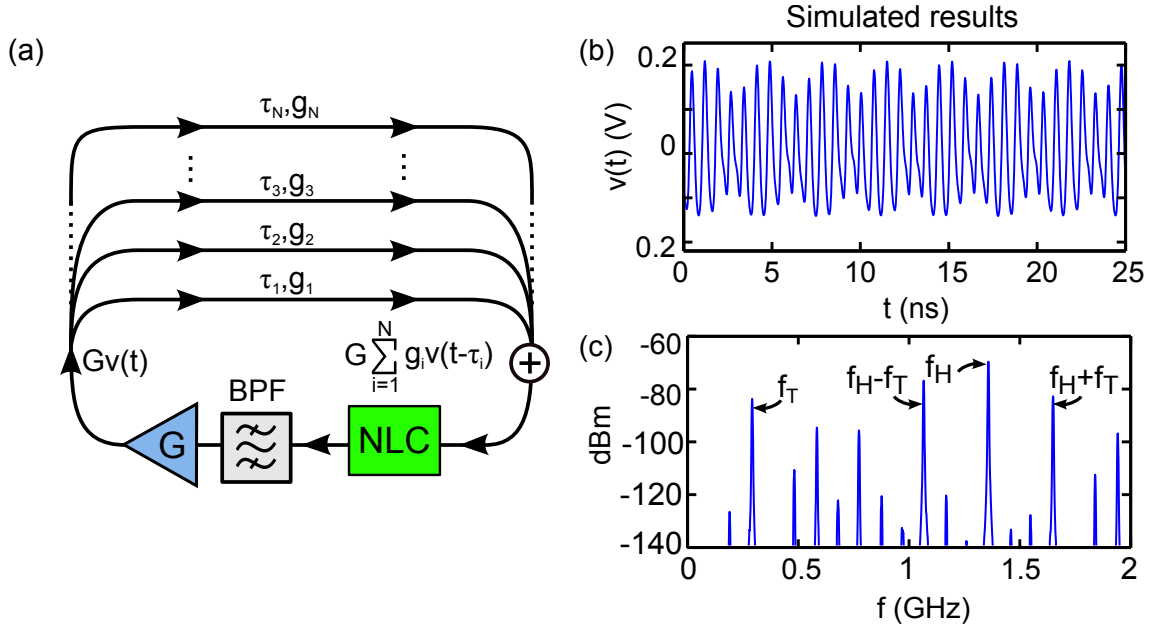
Figure 1.8: Cavity-feedback system model. (a) Pictorial representation of the model. The output voltage of the nonlinear circuit passes through a band-pass filter (BPF) with output v(t) that is amplified with gain G , split among (\tau_i, g_i) , summed, and reinjected into the NLC. (b) Simulated time series of the quasiperiodic oscillations of v(t) while the scatterer's position is fixed. (c) Simulated power spectral density (PSD) of the quasiperiodicity with primary frequencies f_H , f_T , and linear combinations f_H \pm f_T .
