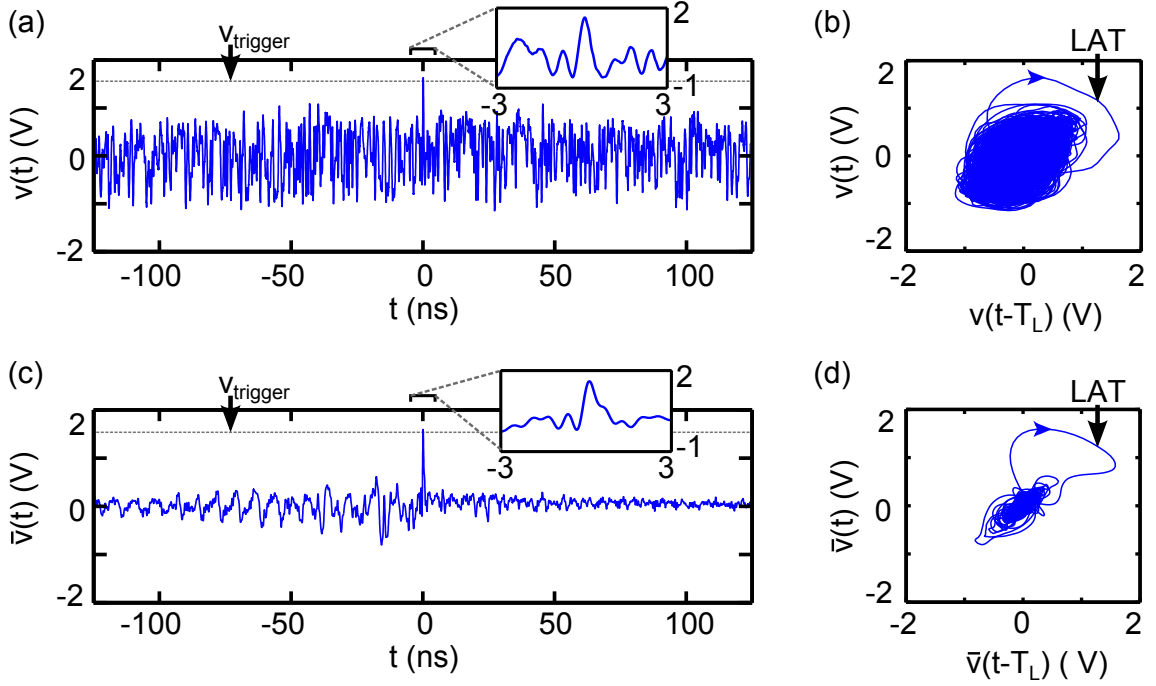
Figure 3.6: Large-amplitude spike event and trajectory using a high level trigger. (a) Chaotic time series v(t) acquired from the oscilloscope with v_{\text{trigger}} \sim 1.6 V. (b) Phase space projection (PSP) of the high-level triggered chaos. (c) Averaged time series and (d) PSP for \bar{v}(t) with v_{\text{trigger}} \sim 1.6 V. In the PSPs of (b) and (d), the time lag T_L = 0.3 ns and the large amplitude trajectories (LATs) are labeled with arrows to indicate the direction of the flow.
