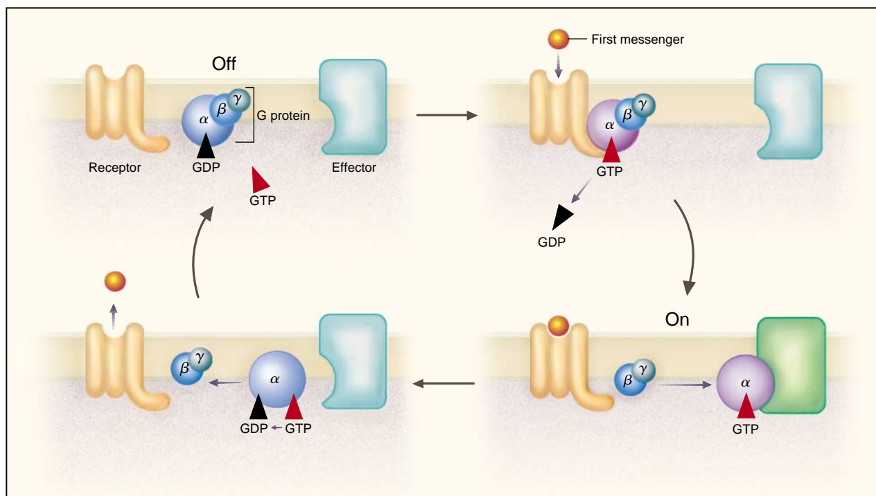
Figure 1. Mechanism of Activation and Action of G Proteins.
