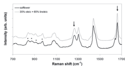
Figure 2 – Raman spectra obtained from the safflower oil analysis and a mixture of oleic and linoleic acid, suggesting that these two compounds are the main constituents of safflower oil in the concentrations shown in the plot. The arrows indicate the peaks at 1655 cm^{-1} and 1265 cm^{-1} attributed to the unsaturated fatty acids. The Raman peaks marked with stars in the region between 800-1000 cm^{-1} represent the characteristic peaks of linoleic acid.
