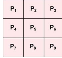
Figure 1. Geometric interpretation of the differential operator \delta_i at vertex i = 5 . It measures the deviation between x_5 and its center of mass \frac{1}{d_5} \sum_{j \in N(5)} w_{ij} x_j .
