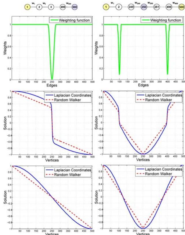
Figure 2. Comparison between the solution obtained from Laplacian Coordinates and the classical Random Walker algorithm under the same initial conditions. Line graphs are shown in the top row with seeded vertices in yellow and purple while the corresponding edge weights are shown in the second row. The solution with and without the mentioned weights are given in the third and fourth rows.
