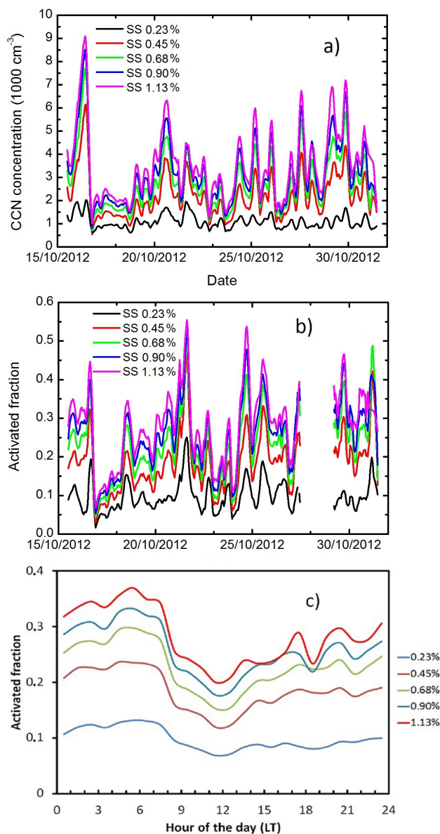
Figure 2. Time series of (a) CCN number concentration, (b) the activated fraction ( \#\text{CCN}/\text{N}_{10-500} ) and (c) the mean hourly average over the whole period. The different colours represent the different SS.
