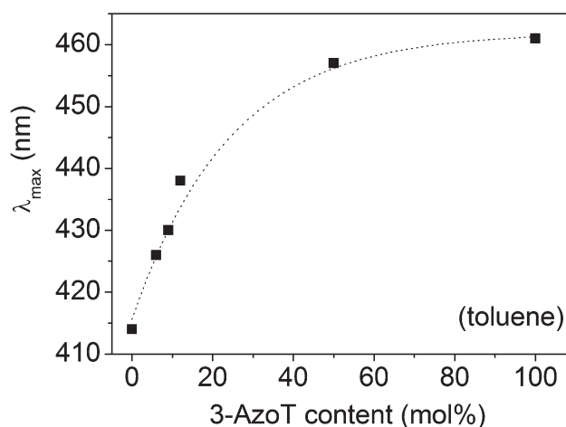
Figure 8 Wavelength of maximum absorbance of toluene solutions for different 3-AzoT contents in the copolymers. The values for 0 and 100% were taken from the literature. 15,34
