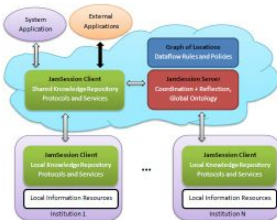
Figure 4. OpenMuseum's architecture.
