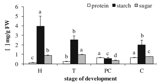
Figure 4. Total protein, starch, and sugar levels ( \text{mg g}^{-1}\text{ FW} ) at different stages of A. sellowiana somatic embryos (mean±standard deviation, n=3 ). H heart, T torpedo, PC precotyledonary, CT cotyledonary. Different letters indicate differences according to the SNK test ( P<.05 ).
