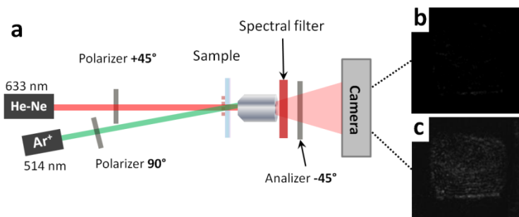
Fig. 2. (a) Experimental setup used to observe the optically induced birefringence in microscopic samples. (b) Image observed in the CCD camera before the writing beam irradiation and (c) after writing beam exposure (one minute).
