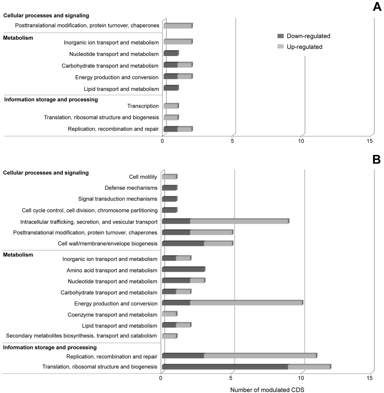
Figure 2. Functional classification of R. rickettsii genes modulated by exposure to a 10°C increase in incubation temperature (A) or to blood feeding (B).
