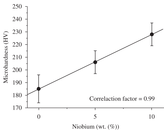
Figure 3. Microhardness of the Ti-5 wt. (%) Nb and Ti-10 wt. (%) Nb alloys.
