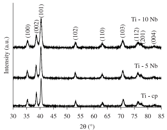
Figure 2. X-ray diffraction for the Ti-5 wt. (%) Nb and Ti-10 wt. (%) Nb alloys.
