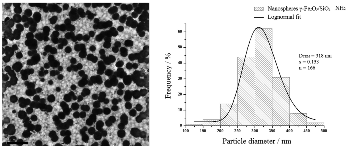
Figure 3. TEM image of \gamma\text{-Fe}_2\text{O}_3/\text{SiO}_2\text{-NH}_2 nanospheres and particle size histogram ( D_{TEM} : average diameter).
