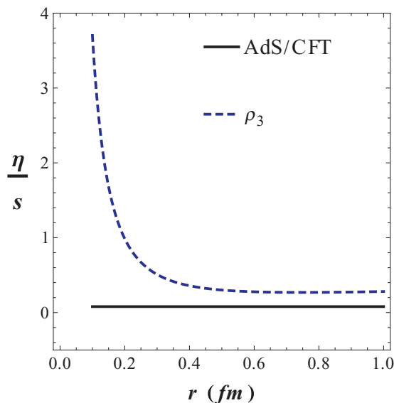
FIG. 7. (Color online) The ratio \eta/s (dashed blue line) as a function of the excluded volume radius computed via (15) using the density of states \rho_3 in Eq. (10) and T = 155 MeV. The black line denotes the viscosity lower bound \eta/s = 1/(4\pi) .
