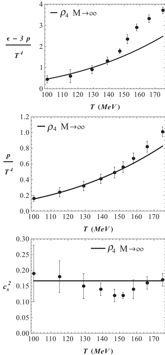
FIG. 5. Trace anomaly, pressure, and speed of sound squared for the hadron resonance model with density of states \rho_4 . The black solid curves denote the result obtained by taking the mass integrals in Eqs. (4)–(7) to infinity. The data points correspond to the N_t = 10 lattice data published in Ref. [15] (obtained from Table 5 in that paper).
