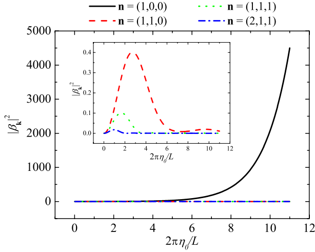
FIG. 2 (color online). The expectation value of created particles |\beta_{\mathbf{k}}|^2 with quantum numbers \mathbf{k} = 2\pi\mathbf{n}/L is exhibited as a function of \eta_0 , where we have assumed that for some time interval the star becomes dense enough such that -V_{\text{eff}} - (\omega_{\mathbf{k}}^{\text{min}})^2 > 0 , while for \omega_{\mathbf{k}} > \omega_{\mathbf{k}}^{\text{min}} we always have -V_{\text{eff}} - \omega_{\mathbf{k}}^2 < 0 (see Fig. 1). Here, we have chosen V_0(L/2\pi)^2 = 1.6 .
