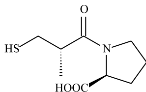
FIGURE 1 – Molecular structure of captopril.
