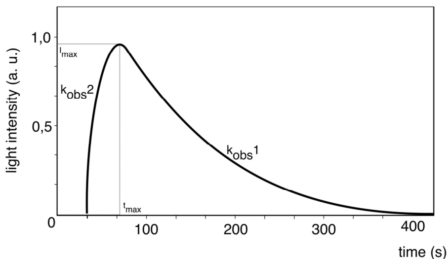
Figure 3. Emission intensity time course of peroxyoxalate chemiluminescence. [TCPO] = 0.1 mM, [H 2 O 2 ] = 10.0 mM, [IMI-H] = 1.0 mM and [DPA] = 1.0 mM, in anhydrous ethyl acetate at 25°C.
