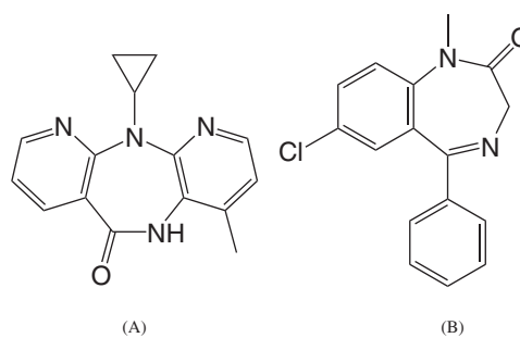
Figure 1. Chemical structures of nevirapine (A) and diazepam (B).
