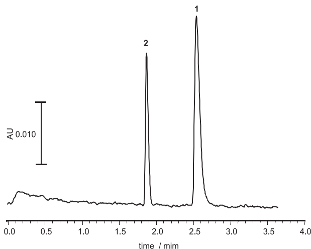
Figure 2. Electropherogram of nevirapine (peak 1; 100.0 \mu\text{g mL}^{-1} ) and diazepam (peak 2; 50.0 \mu\text{g mL}^{-1} ) standard drugs. Conditions: silica-fused capillary with 75 \mu\text{m} i.d. and a total length of 27 cm (19.4 cm to the detector), electrolyte constituted of 10 mmol \text{mL}^{-1} phosphate buffer at pH 2.5, hydrodynamic injection 0.5 psi for 5 s, UV detection at 200 nm, applied voltage +25 kV.
