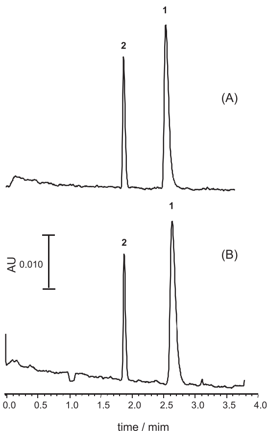
Figure 3. Electropherograms of: A) nevirapine (peak 1; 100.0 \mu\text{g mL}^{-1} ) and diazepam (peak 2; 50.0 \mu\text{g mL}^{-1} ) standard solutions. B) Typical pharmaceutical sample (tablet from laboratory A). Conditions: capillary of silica-fused with 75 \mu\text{m} i.d. and a total length of 27 cm (19.4 cm to the detector), electrolyte: 10 \text{ mmol mL}^{-1} phosphate buffer at \text{pH} = 2.5 , injection: 0.5 psi for 5 s, detection at 200 nm, voltage: +25 kV.
