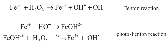
Scheme 1. Hydroxyl radical generation from Fenton and photo-Fenton reactions
