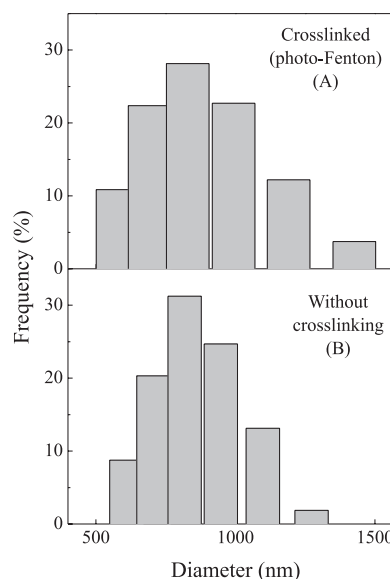
Figure 4. Diameter distribution of soy lecithin vesicles containing PVP. (A) vesicles submitted to photo-Fenton reaction and (B) vesicles prior to crosslinking reaction
