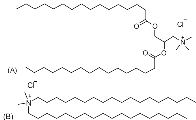
Figure 2. Structures of (A) DPTMA and (B) DODAC
