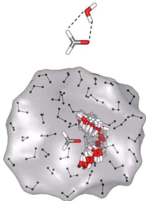
Figure 4. Illustration of the hydrogen bonded structures obtained from the MC simulation. Top is for the optimized formaldehyde-water complex. Bottom is for the configurations extracted from the MC simulations and in addition includes the electrostatic field of the solvent. Superposition of all formaldehyde-water is made to emphasize the configuration space spanned by the hydrogen bonds. Each QM calculation uses only one water molecule that is hydrogen-bonded to the formaldehyde molecule.
