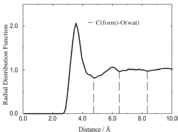
Figure 1. The radial distribution function between the carbon atom of formaldehyde and the oxygen atom of water.
