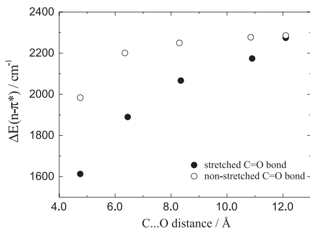
Figure 3. Solvatochromic shift of the n \rightarrow \pi^* transition of formaldehyde in water, as a function of the solute-solvent distance. Results obtained using TD-DFT/6-311++G(d,p) with the stretched and non-stretched C=O distances. The points are the results obtained with the inclusion of 15, 35, 80, 180 and 210 water molecules represented by simple point charges.
