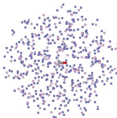
Figure 2. Illustration of one MC configuration of the formaldehyde molecule in the environment of the solvent liquid water.
