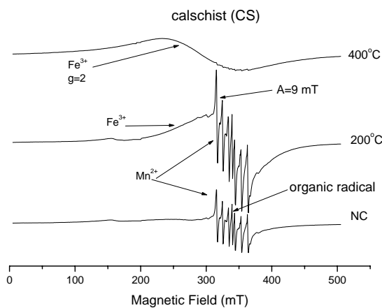
FIG. 1: EPR signals for the calcschist sample with variation of magnetic field (B) 500 mT at non calcined (NC) 200^\circ\text{C} and 400^\circ\text{C} . The Fe^{3+} signal for the three calcination temperatures. At 400^\circ\text{C} the gain in signal is lower, however, the intensity of Fe^{3+} signal is higher.
