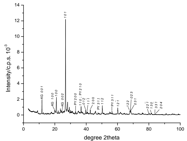
FIG. 4: XRD analysis of the non-calcined RS sample showing quartz as principal mineral and respective peaks indicated with hkl indexes, kaolin group (label: KG) and pyrite (PY) indicated with label and indexes hkl .
