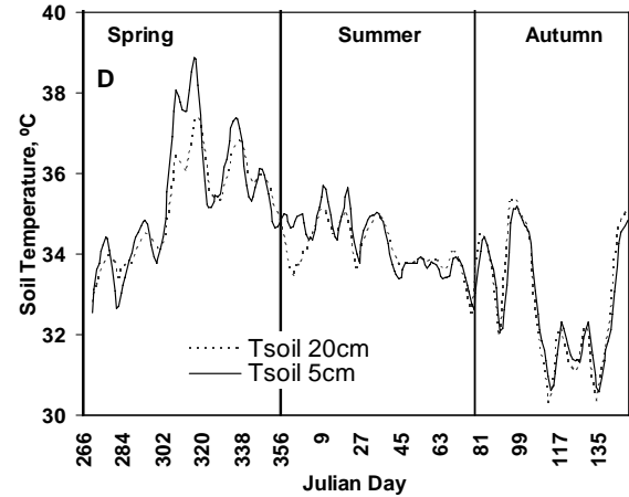
Figure 1 - Five-day moving averages of measured meteorological variables inside the canopy (3/4 of canopy height) and at the reference level (2 meters above canopy): A) Temperature, B) Relative humidity and accumulated rain, C) Wind speed, D) Soil temperature (5 and 20cm below the surface).
