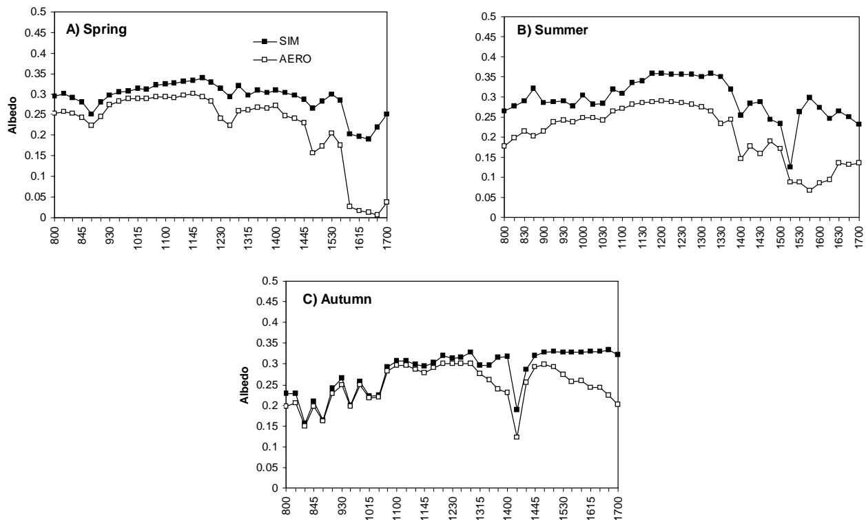
Figure 5- Hourly average albedo simulated by Deardorff (1978) model (SIM) and calculated by aerodynamic method (AERO) during spring (A), summer (B) and autumn (C) seasons.
