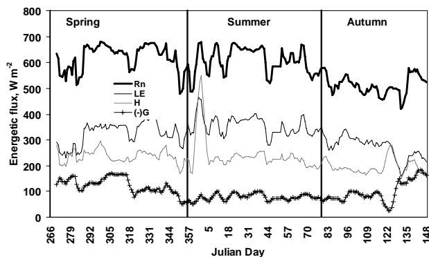
Figure 2 - Five-day moving average of maximum hourly values of energy balance components (Rn – Net radiation, LE – Latent heat flux, H – Sensible heat flux at the atmosphere and G – Sensible heat flux in the soil) estimated by the aerodynamic method.
