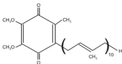
FIGURE 1 - Structure of coenzyme Q 10 (2,3-dimethoxy-5-methyl-6-decaprenyl-1,4-benzoquinone). Source: Shinde, Patil, Tendolkar, 2005.
