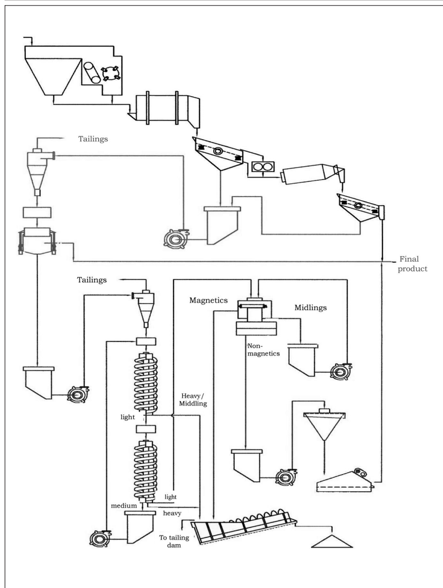
Figure 4 - Present flowsheet.
