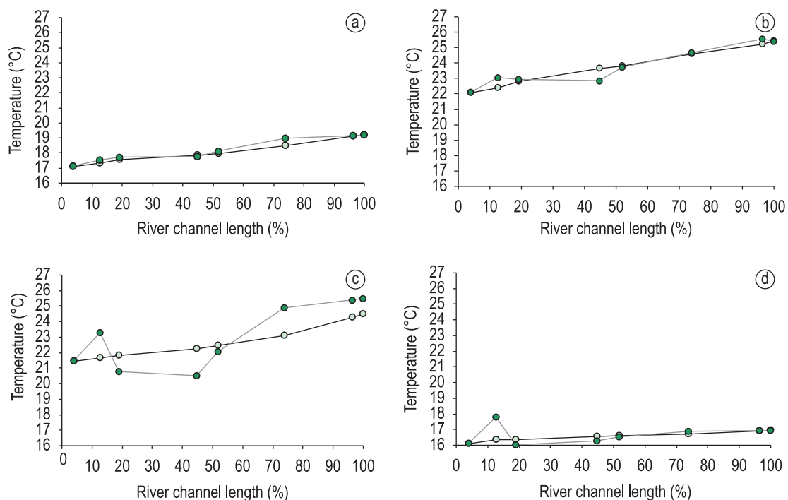
Figure 4. Water temperature variation (°C) in Canha River, during the spring (a - September), summer (b - January), autumn (c - April) and winter (d - July) periods, respectively. ○: observed water temperature; ●: simulated water temperature.
