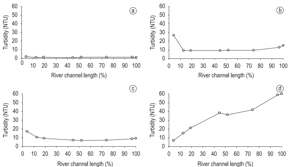
Figure 8. Turbidity variation (NTU) in Canha River, during the spring (a - September), summer (b - January), autumn (c - April) and winter (d - July) periods, respectively. ○: observed turbidity.
