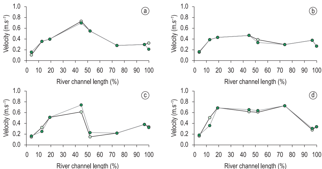
Figure 3. Velocity variation (m/s) in Canha River, during the spring (a - September), summer (b - January), autumn (c - April) and winter (d - July) periods, respectively. ○: observed velocity; ●: simulated velocity.
