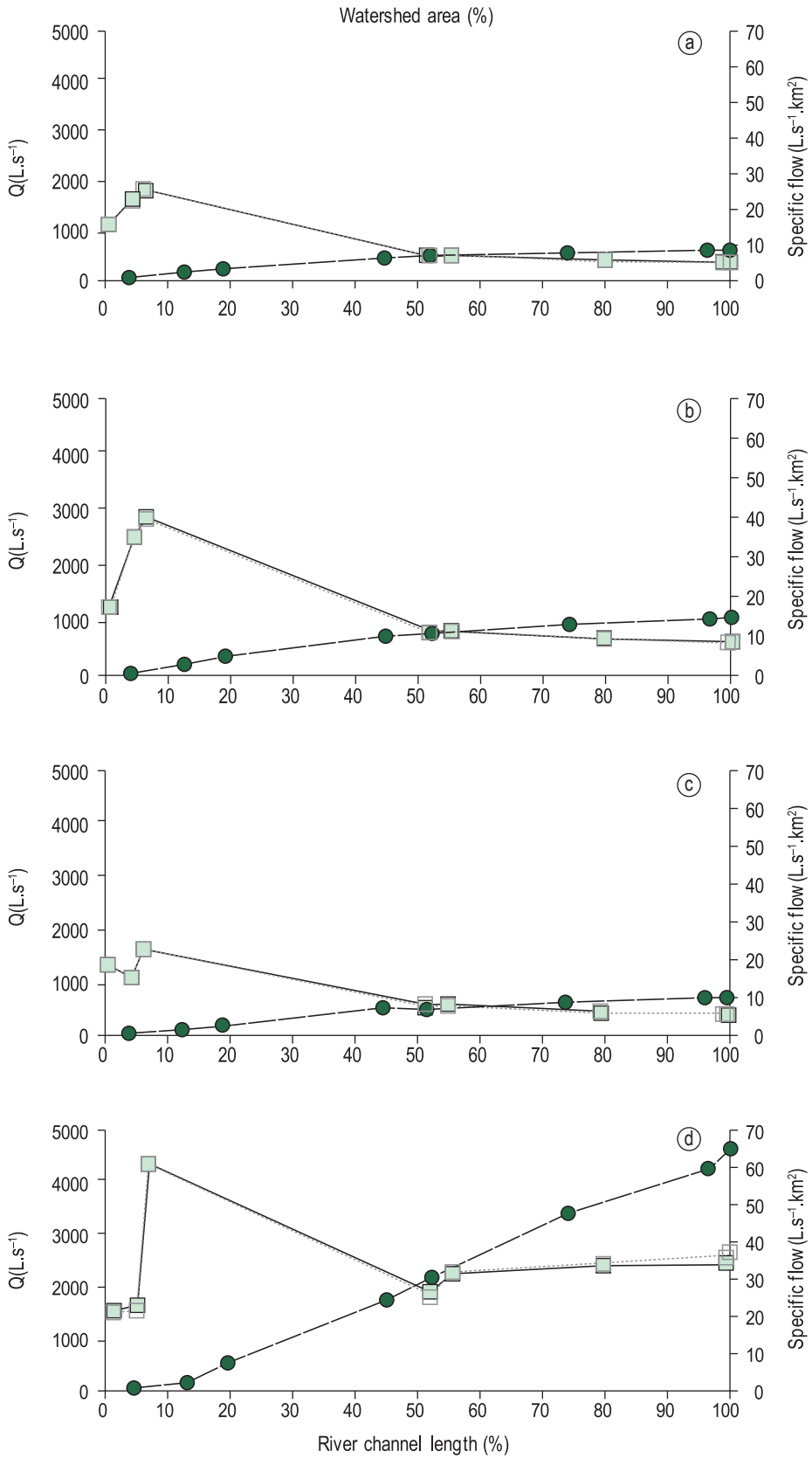
Figure 2. Flow variation in Canha River (inferior abscissa, left ordinate) and specific flow variation in the watershed increment (superior abscissa, right ordinate), during the spring (a - September), summer (b - January), autumn (c - April) and winter (d - July) periods, respectively. ●: observed flow; □: observed specific flow; □: simulated specific flow.
