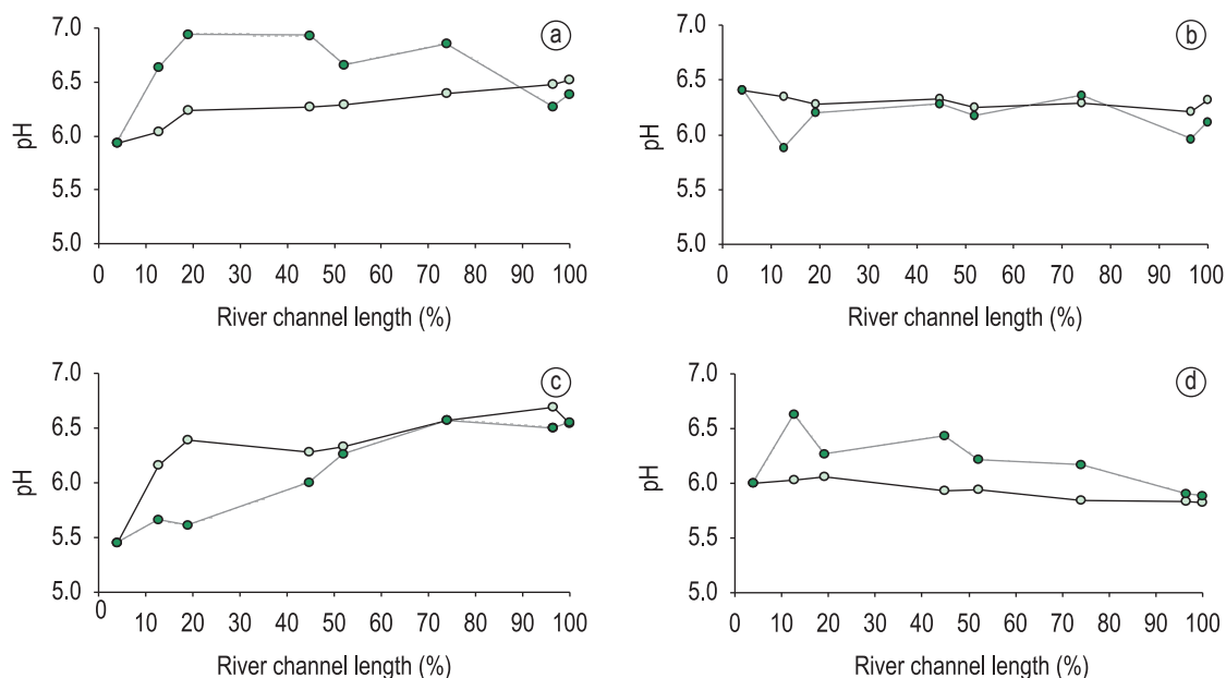
Figure 7. pH variation in Canha River, during the spring (a - September), summer (b - January), autumn (c - April) and winter (d - July) periods, respectively. ○: observed pH; ●: simulated pH.
