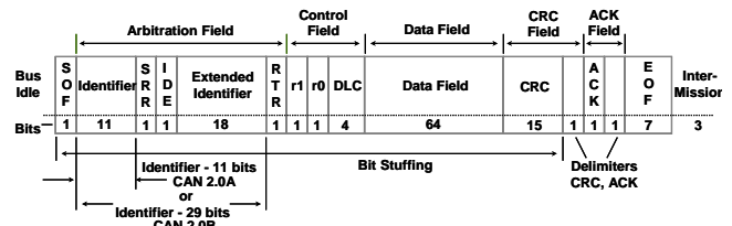
Figure 1. Message frame formats defined by the CAN protocol (Godoy, 2007).
