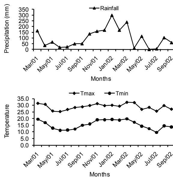
Figure 1 – Climatic data for maximum and minimum temperature and rainfall during the first sugarcane growing season (plant cane cycle-2001, 2002).
