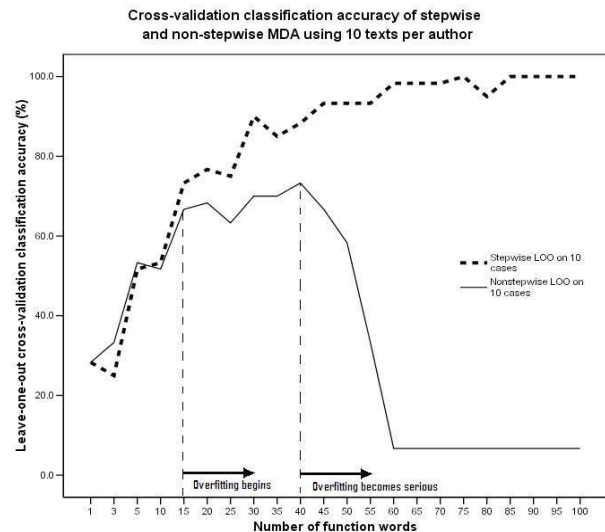
Figure 3b: LOO cross-validation classification accuracy (y-axis) of both stepwise and non-stepwise MDA using ten texts per author as the training data set (randomly sampled from corpus) varying the number of function words used (x-axis).
