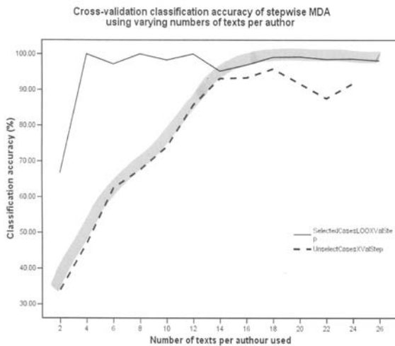
Figure 2: The effect on classification accuracy (y-axis) of changing training data size (x-axis) using stepwise MDA.
