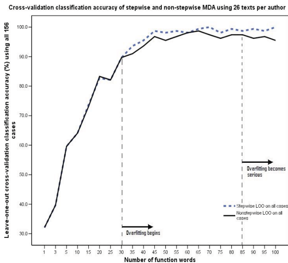
Figure 3a: LOO cross-validation classification accuracy (y-axis) of both stepwise and non-stepwise MDA using 26 texts per author as the training data set (the entire corpus) varying the number of function words used (x-axis).
