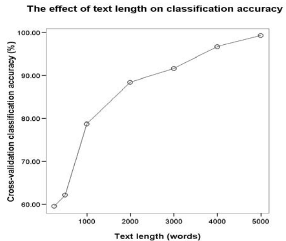
Figure 3: The effect of text length (x-axis) on classification accuracy (y-axis).
