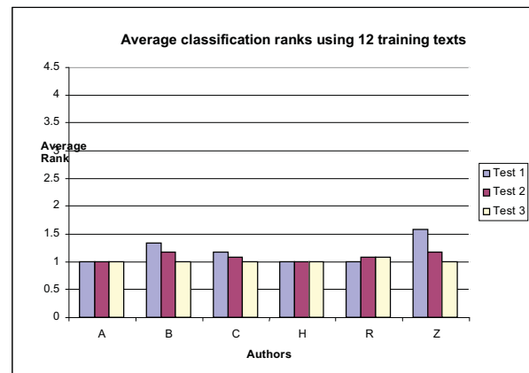
Figure 2b: Average classification rank (y-axis) of texts by each of six authors (x-axis) using 12 texts from each author as model training data.
