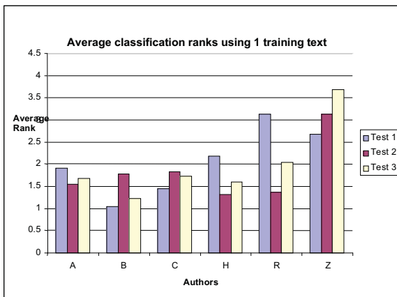
Figure 2a: Average classification rank of texts (y-axis) by each of six authors (x-axis) using a single text from each author as model training data.
