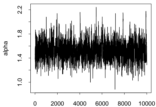
Figure 1.2: Sampled Path for alpha
