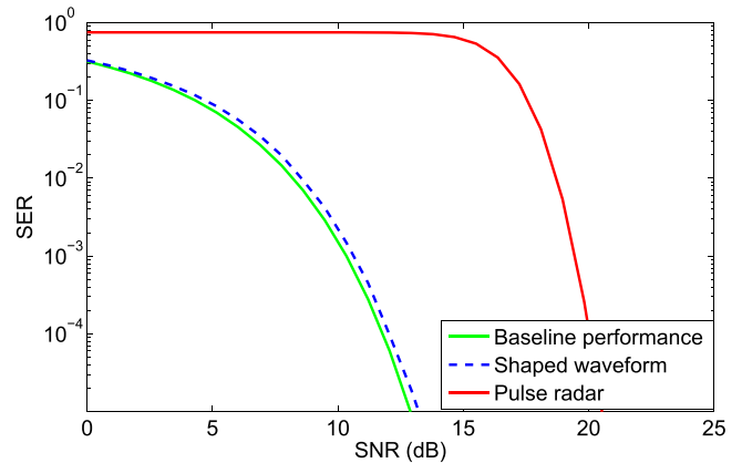
FIGURE 10. SER performance curves for QPSK receiver with 9 dB radar-to-noise ratio for a single narrowband communication system.
