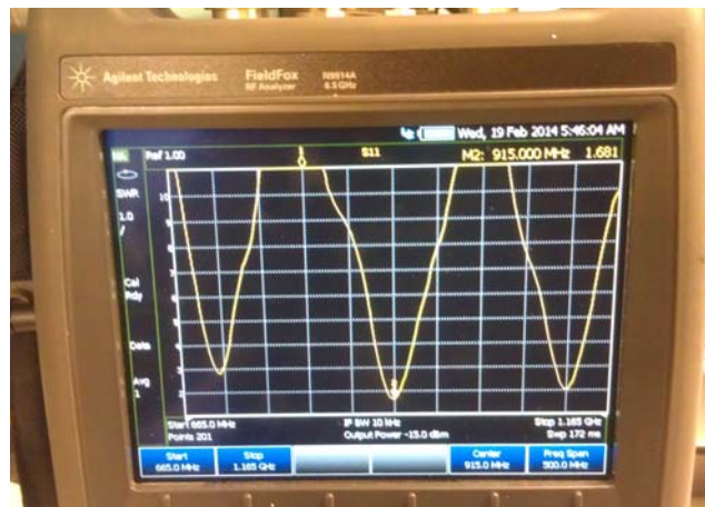
Figure 31. Spectrum analyzer test of final UHF feed antenna
