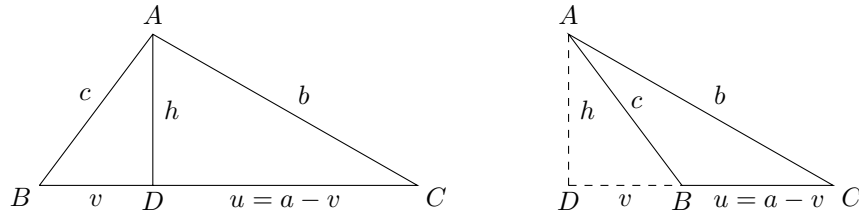
Figure 1: Heron triangle with fixed height h .
