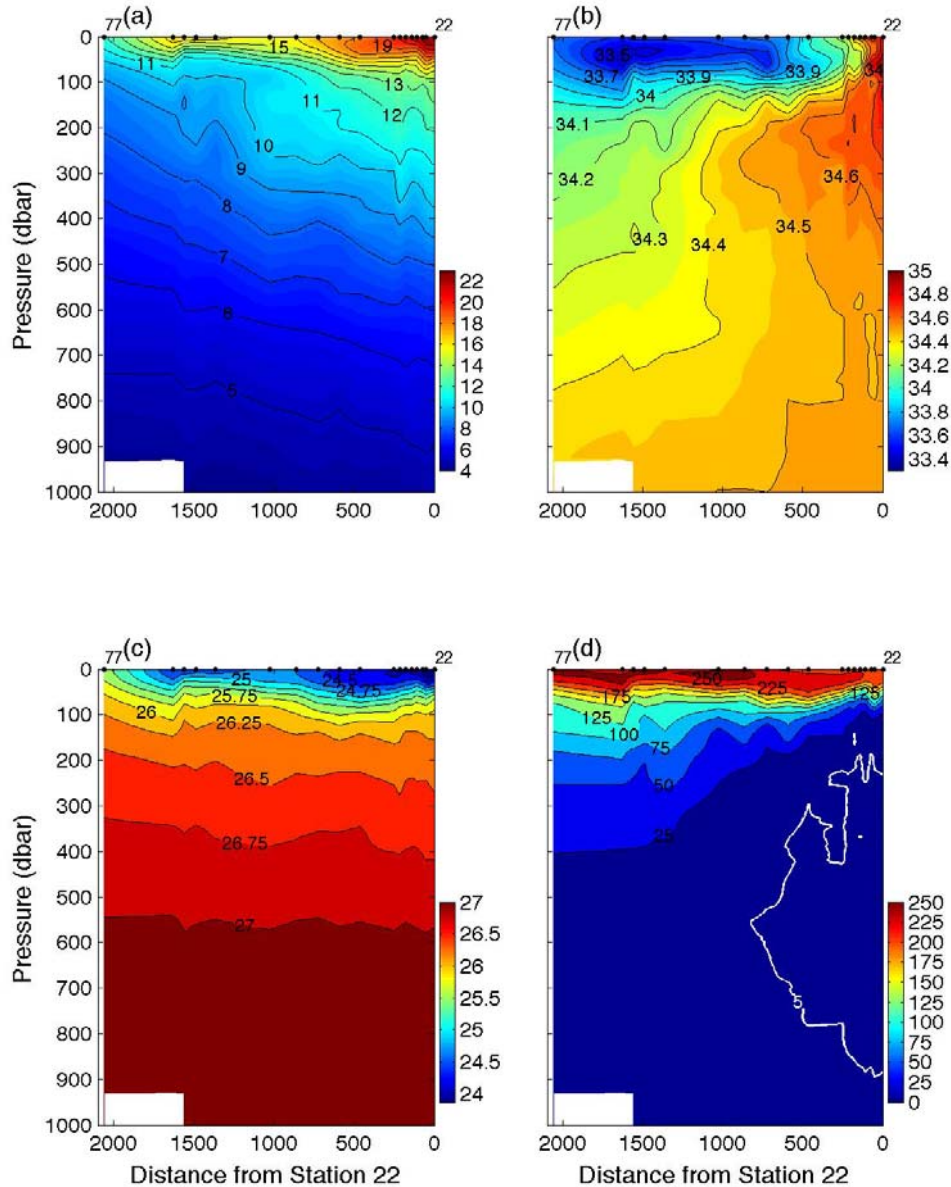
Figure 8. Water properties along the 1000 m isobath from Pescadero Basin (Station 22) to San Diego (Station 77). (a) Temperature, °C. Contour interval is 1°C. (b) Salinity. Contour interval is 0.1. (c) Density anomaly, kg/m 3 . Contour interval is 0.25 kg/m 3 . (d) Dissolved oxygen, µmol/kg. Contour interval is 25 µmol/kg, except 5 µmol/kg is white.
