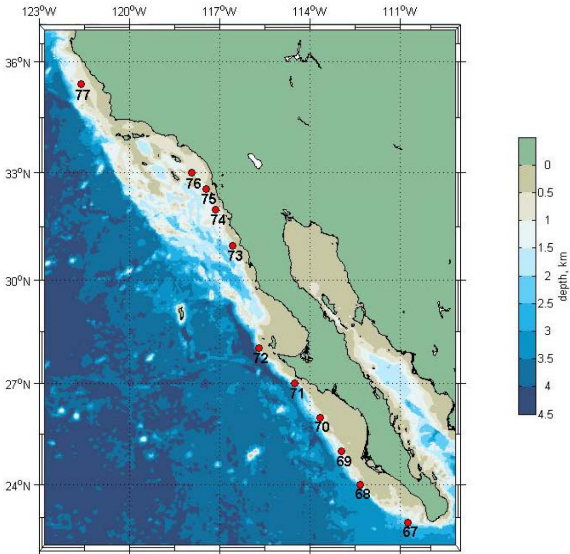
Figure 2: Hydrographic stations occupied during April 2013 near the 1000 m isobath between the Entrance to the Gulf of California and southern California.
