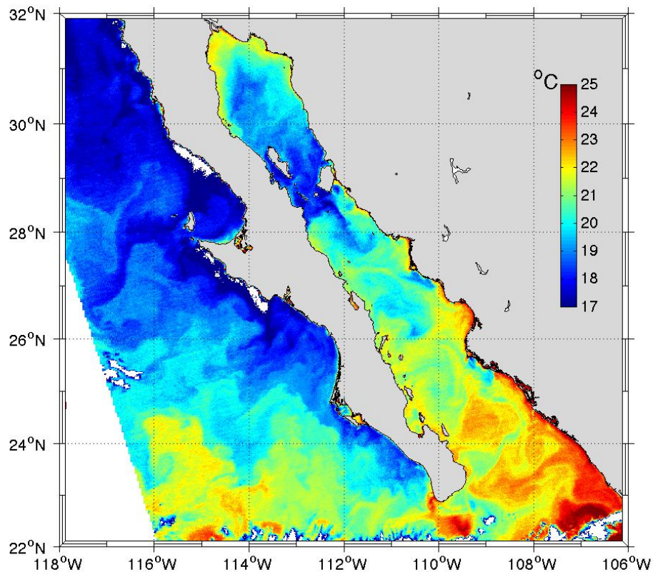
Figure 3: Advanced Very High Resolution Radiometer (AVHRR) satellite imagery of sea surface temperature (°C) of the area of operation during the PESCAR24 cruise of April 2013. This image was taken on 19 April 2013.
