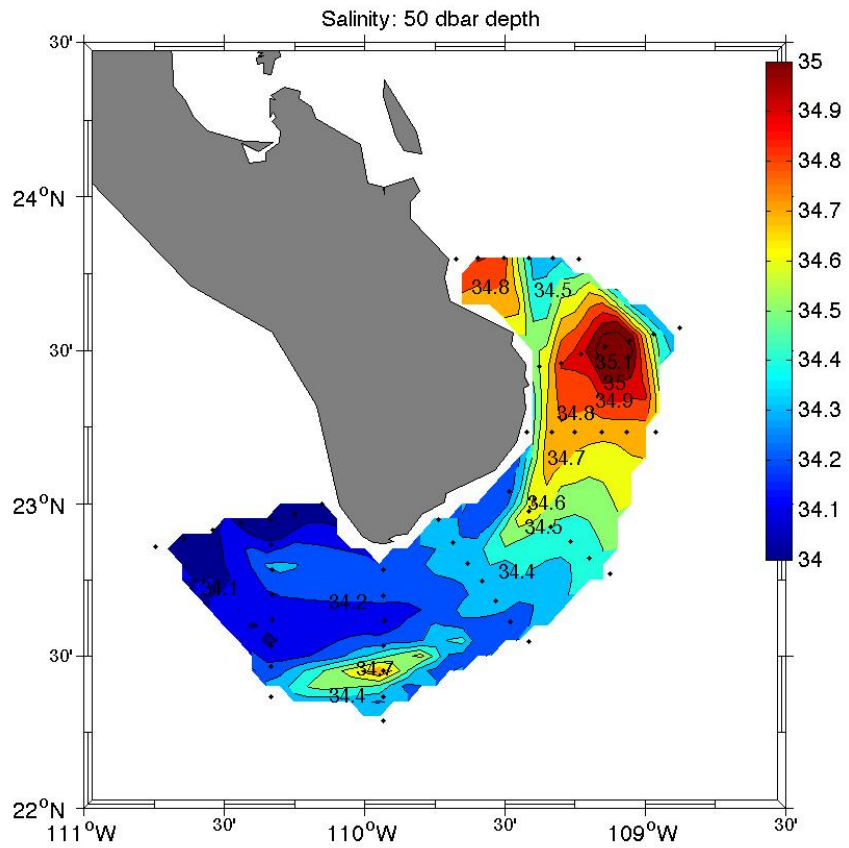
Figure 6. Salinity on the 50 dbar surface. Contour interval is \Delta S=0.1 . Black dots indicate station positions.
