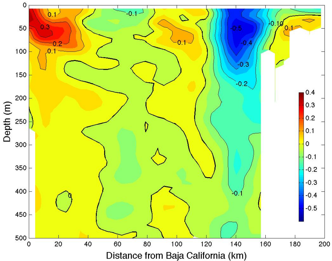
Figure 5. Flow into the Gulf of California across the Pescadero Basin section. Contour interval is 0.1 m/s. The black line is the zero isotach. Positive flow is in the direction of 339.5^{\circ}\text{T} . Data include both SADCP and LADCP observations.
