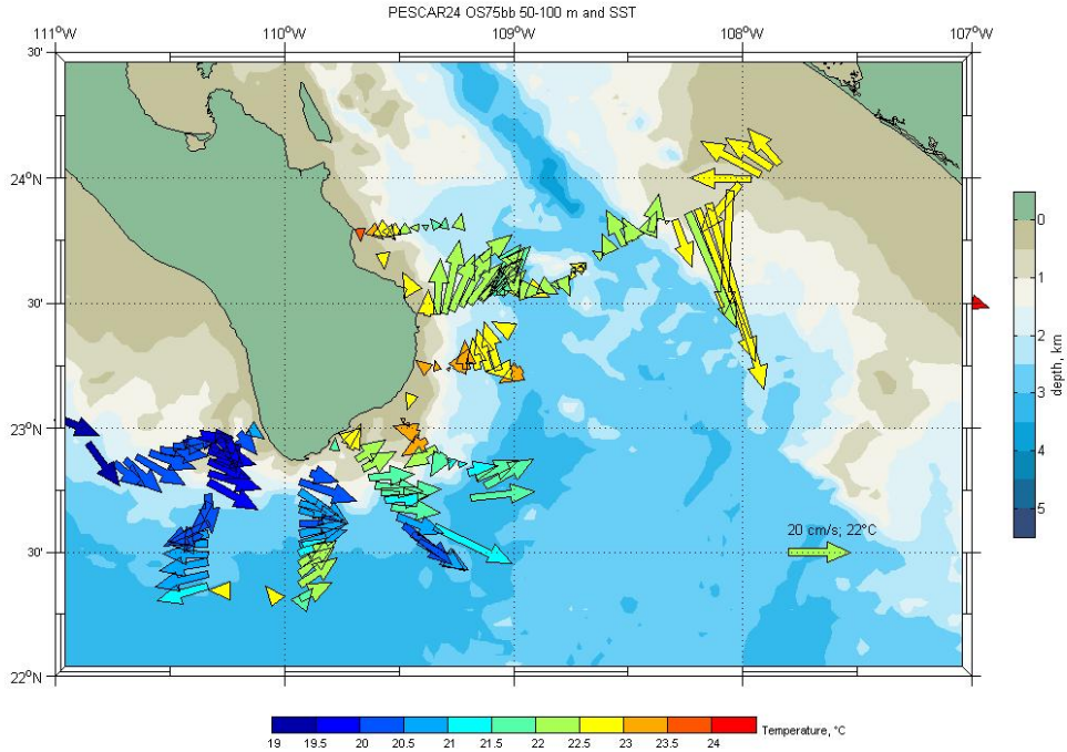
Figure 7: Shipboard Acoustic Doppler Current Profiler (SADCP) results from the PESCAR cruise of April 2013. The arrows are current vectors for currents averaged between 50 and 100 m. The colors of the current vectors reflect the sea surface temperature as measured (nominally at 3 meters) by the ship's underway data acquisition system (UDAS).
