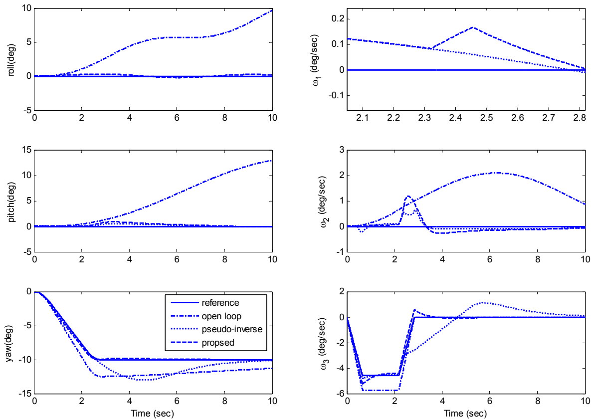
Figure 12: Resulting Slew Trajectories from Simulation
