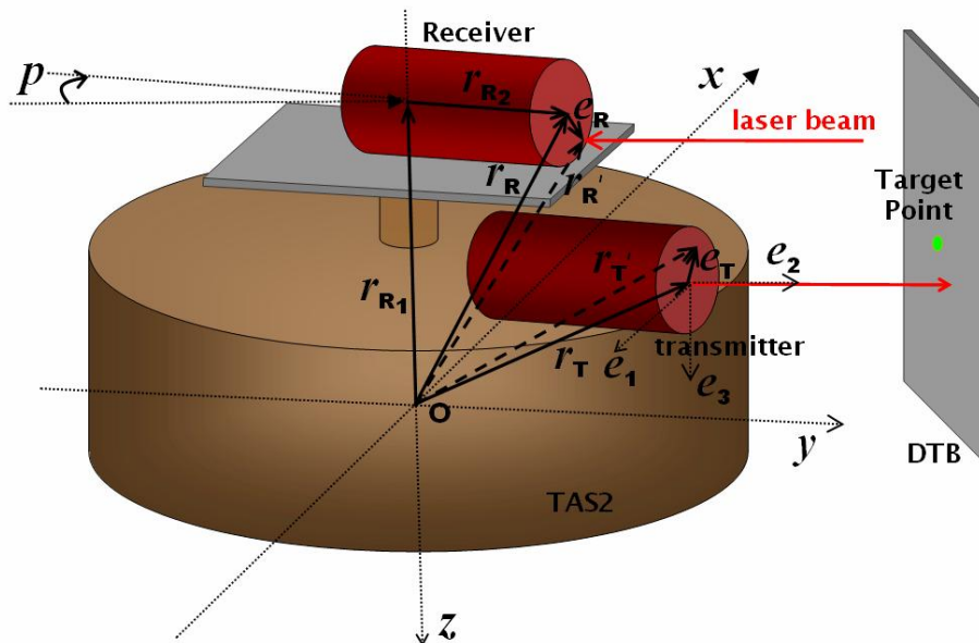
Figure 14: Laser Relaying Control Law Development for TAS2
