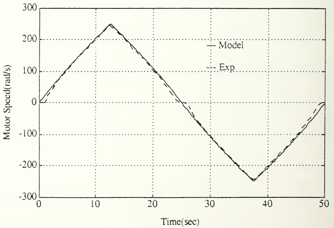
Figure 3.4 Triangular Wave, 50 Sec Period, Motor Voltage +/- 20.4 v
