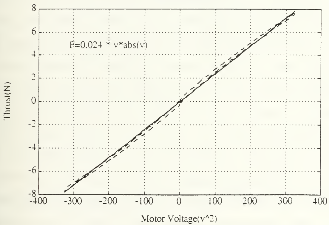
Figure 4.2 Force/Voltage Static Map
