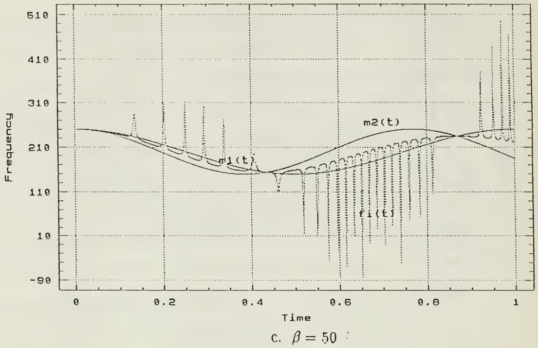
Fig. 2.1 Instantaneous Frequency for Tone Messages where a_1/a_2 = 1.2 , f_c = 200 Hz, f_1 = 1 Hz, f_2 = 1.3 Hz
