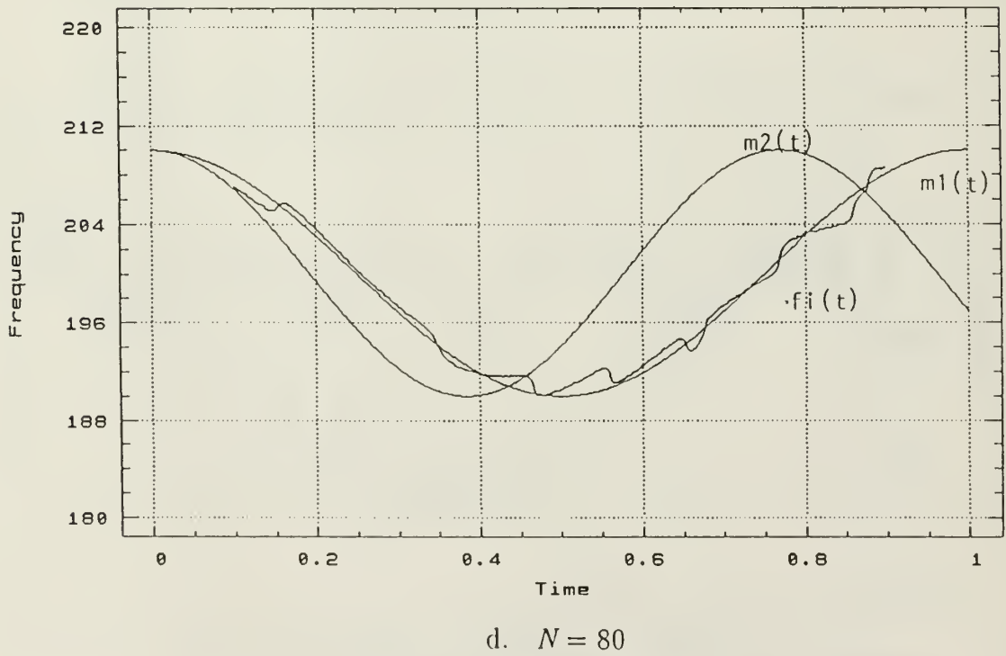
Fig. 4.3 Average Instantaneous Frequency Deviation for Tone Messages where a_1/a_2 = 1.2 , \beta = 10 , f_c = 200 Hz, f_1 = 1 Hz, f_2 = 1.3 Hz
