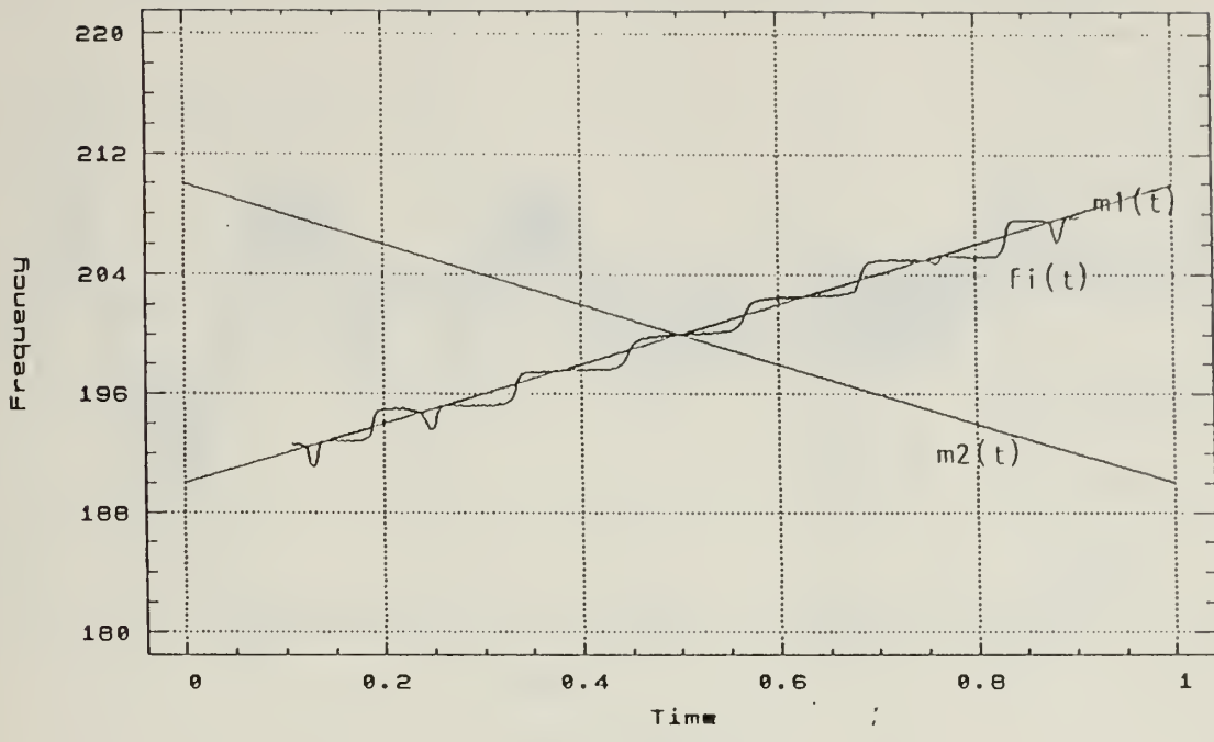
Fig. 4.1 Average instantaneous Frequency Deviation for CHIRPS
