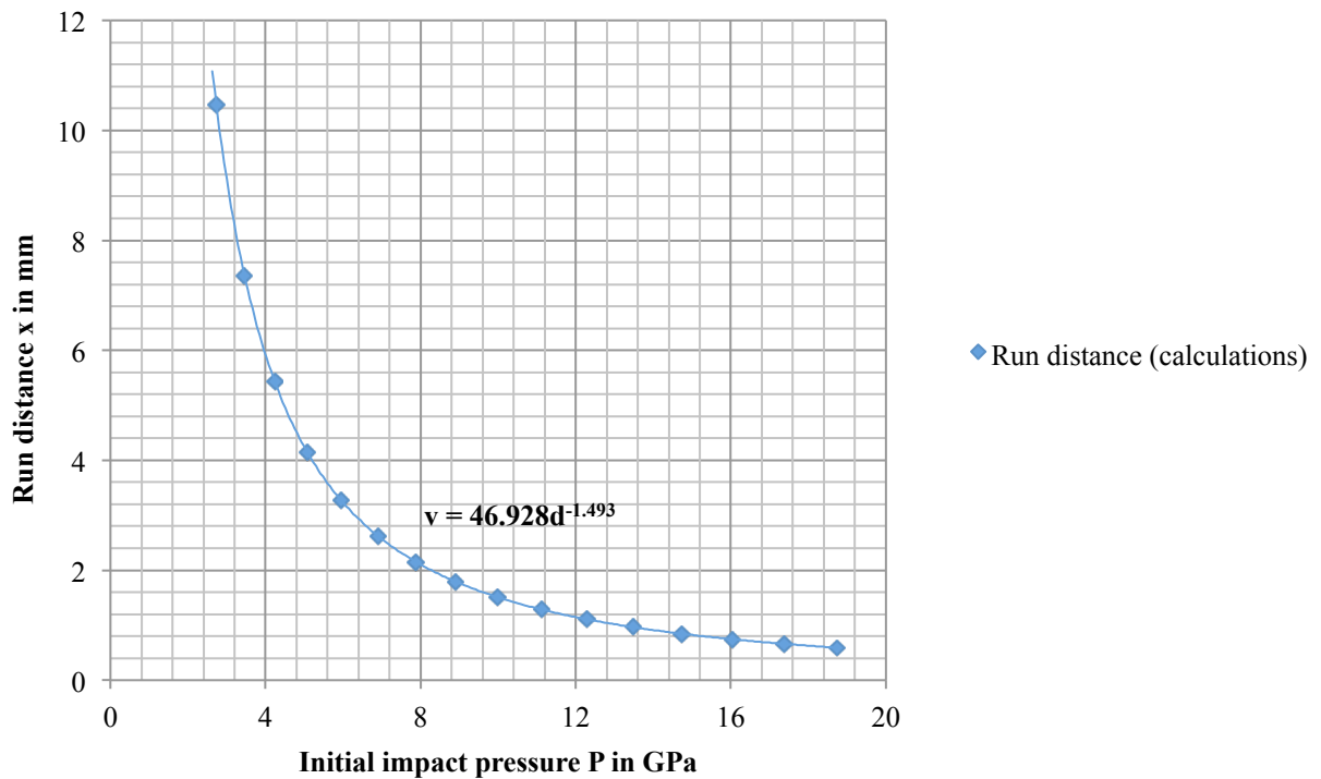
Figure 51: Run distance as a function of the initial impact pressure. Calculation results obtained for a steel projectile impacting a block of explosive PBX 9404 from Popalato.
