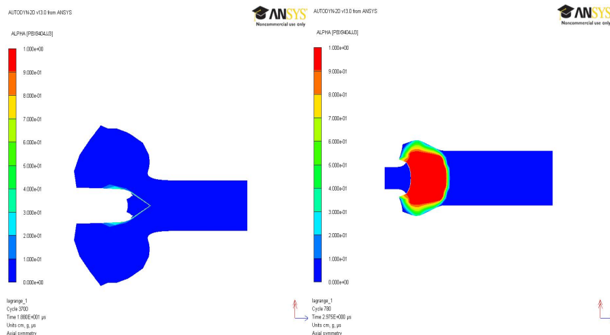
Figure 64: Use of the ALPHA variable and visualization of the detonation process. No detonation occurs on the left simulation (completely blue) while a detonation occurs on the right one (red in progress to the right).
