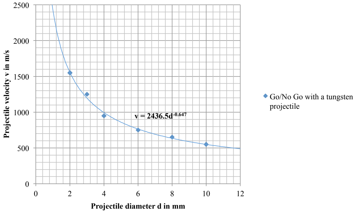
Figure 45: "Go/No Go" velocities as a function of the projectile diameter. Simulation results obtained for a tungsten projectile impacting a bare block of explosive PBX 9404 by a zoning of 2 cells/mm.
