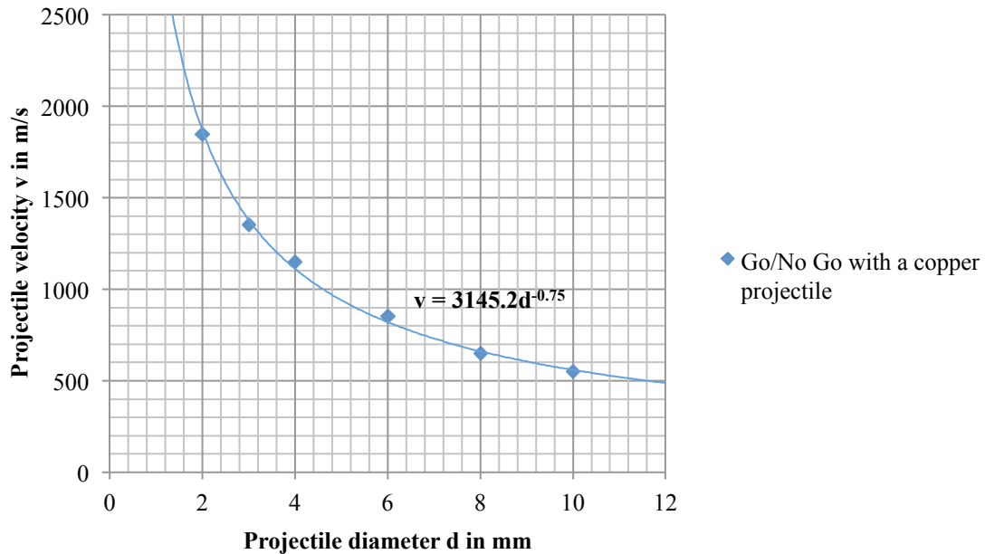
Figure 43: "Go/No Go" velocities as a function of the projectile diameter. Simulation results obtained for a copper projectile impacting a bare block of explosive PBX 9404 by a zoning of 2 cells/mm.
