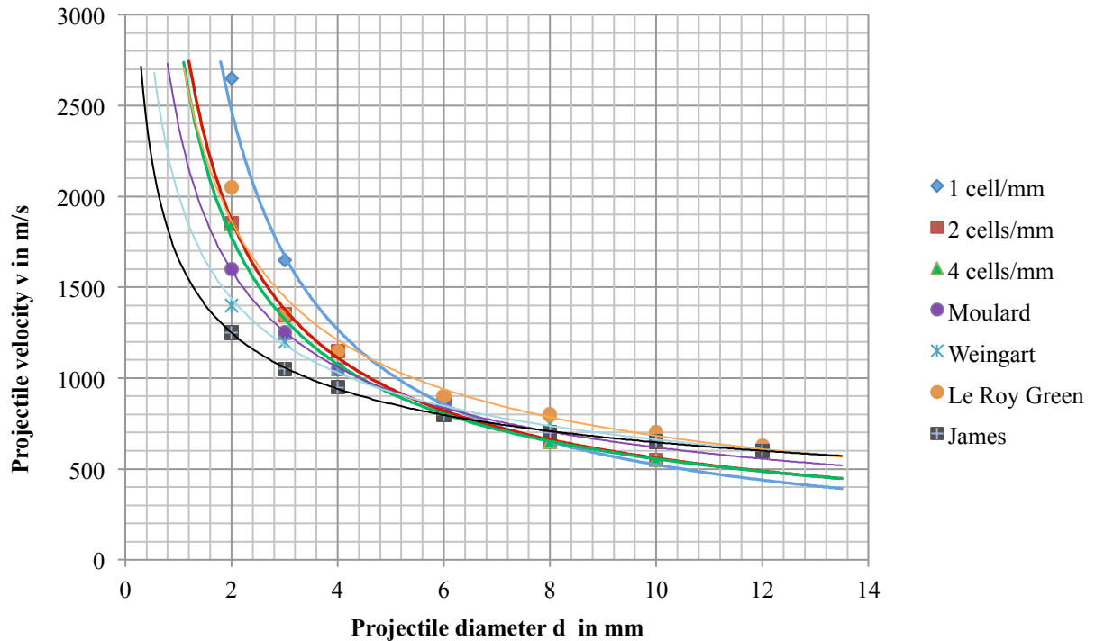
Figure 55: "Go/No Go" velocities as a function of the projectile diameter. Simulation results obtained for a steel projectile impacting a bare block of explosive PBX 9404 by a zoning of 1 cell/mm, 2 cells/mm and 4 cells/mm. Moulard, Weingart, LeRoy Green and James experimental results obtained in the literature [026, 027, 028, 029].
