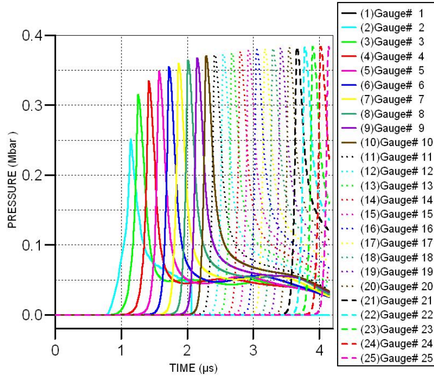
Figure 15: Example of a first-order detonation resulting from impact initiation. Increase of the pressure along the centerline as a function of the time. The reached steady state pressure after 4 \mu\text{s} is about 0.385 Mbar (Von Neumann Spike) and the detonation pressure is about 0.370 Mbar (Chapman Jouguet pressure). Simulation results obtained for a steel projectile with a diameter of 4 mm and a velocity of 1200 m/s impacting a bare block of explosive PBX 9404 at a zoning of 1 cell/mm. The gauge separation is 1 mm.
