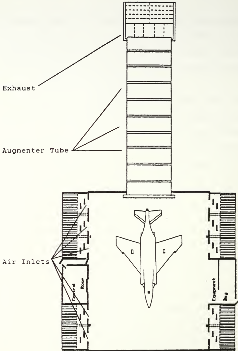
Figure 2.1 Actual Hush House (Top View Looking Down)
